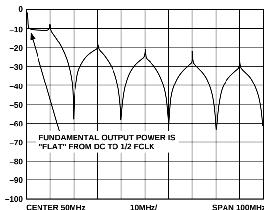
Figure 34. Inverse \text{SIN}(x)/x (Inverse SINC) Filter Engaged
