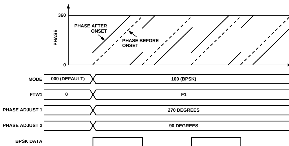
Figure 48. BPSK Mode
