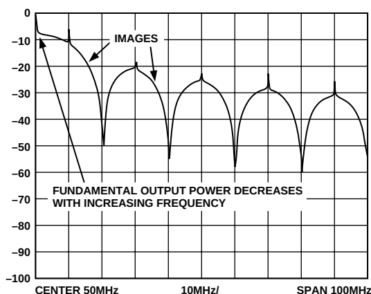
Figure 33. Normal \text{SIN}(x)/x DAC Output Power Envelope Filter
