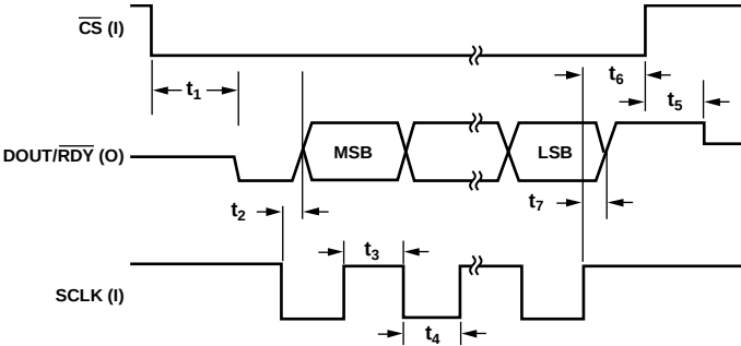
Figure 3. Read Cycle Timing Diagram
