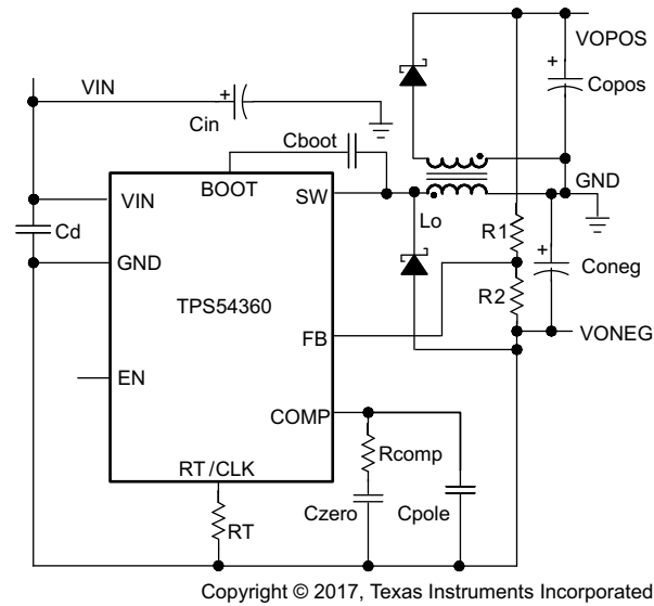
Figure 33. TPS54360 Split Rail Power Supply
