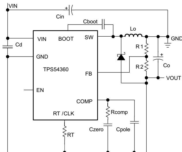
Figure 32. TPS54360 Inverting Power Supply
