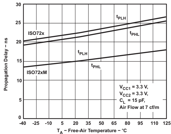
Figure 3. Propagation Delay vs Free-Air Temperature
