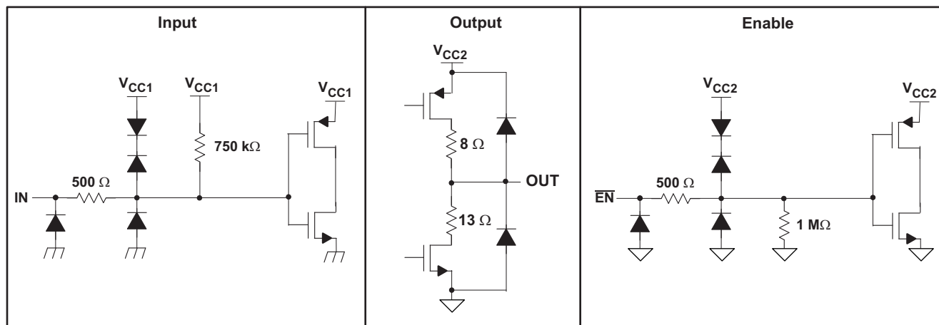
Figure 17. Equivalent Input and Output Schematic Diagrams
