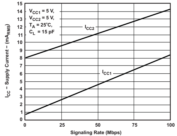
Figure 2. RMS Supply Current vs Signaling Rate
