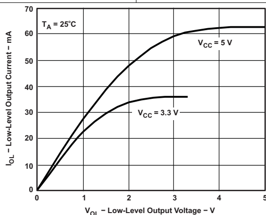
Figure 9. Low-Level Output Current vs Low-Level Output Voltage
