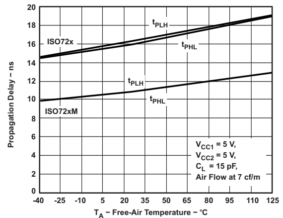
Figure 4. Propagation Delay vs Free-Air Temperature
