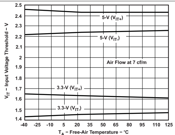
Figure 6. ISO72xM Input Threshold Voltage vs Free-Air Temperature
