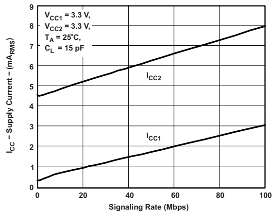
Figure 1. RMS Supply Current vs Signaling Rate
