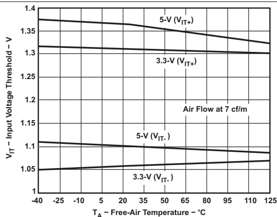
Figure 5. ISO72x Input Threshold Voltage vs Free-Air Temperature
