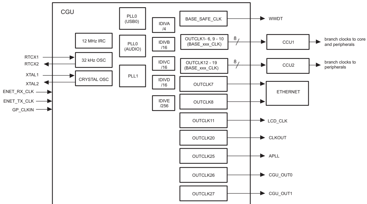
Fig 25. CGU and CCU1/2 block diagram
