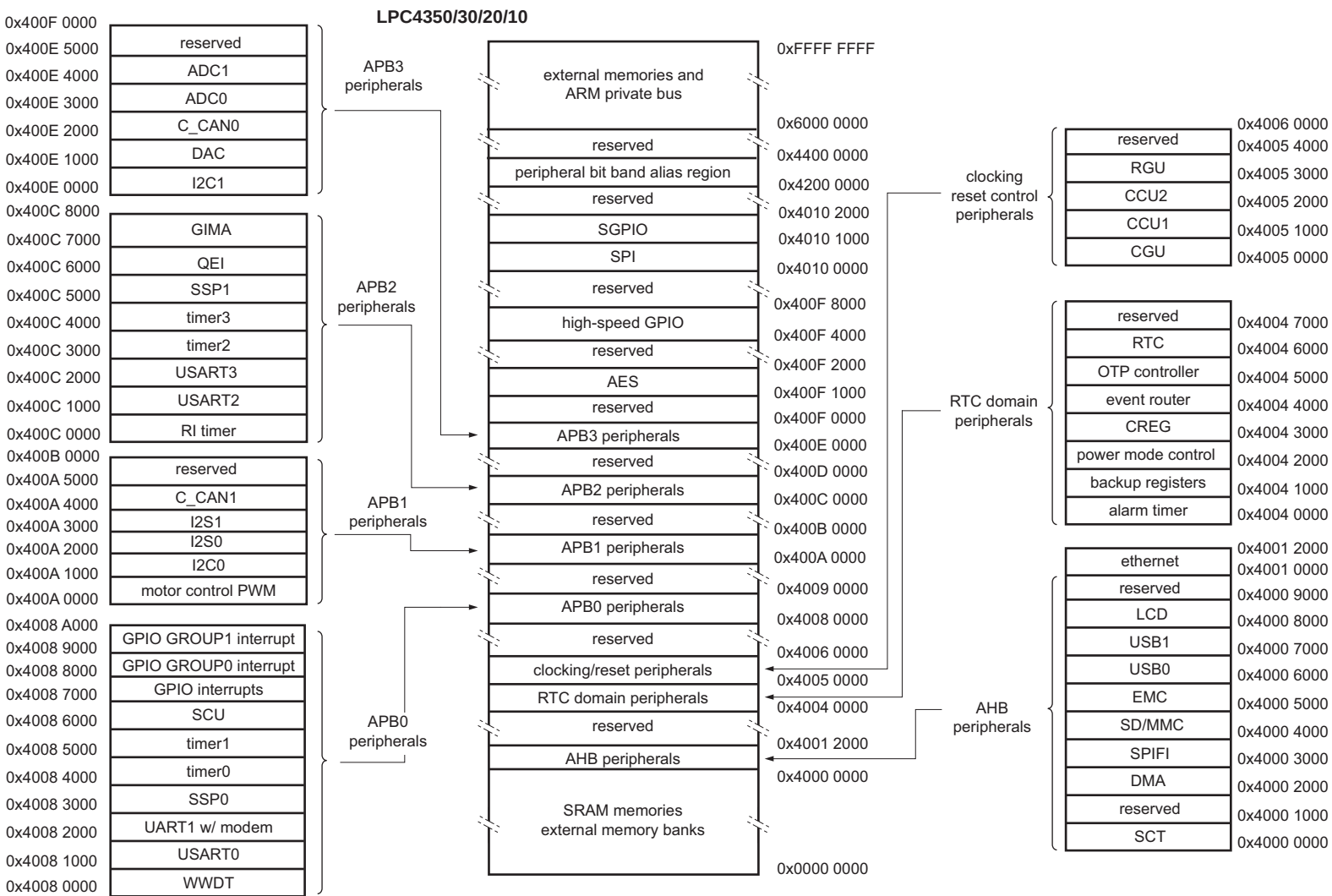
Fig 5. Memory map with peripherals (see Figure 4 for detailed addresses of memory blocks)
