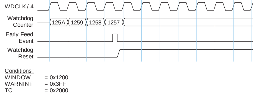
Fig 109. Early Watchdog Feed with Windowed Mode Enabled
