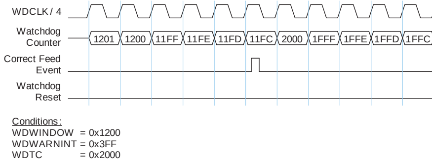
Fig 110. Correct Watchdog Feed with Windowed Mode Enabled
