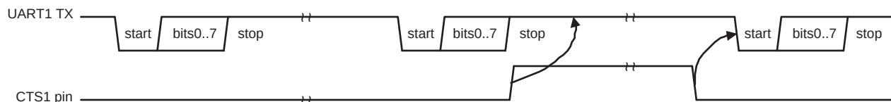
Fig 121. Auto-CTS Functional Timing
