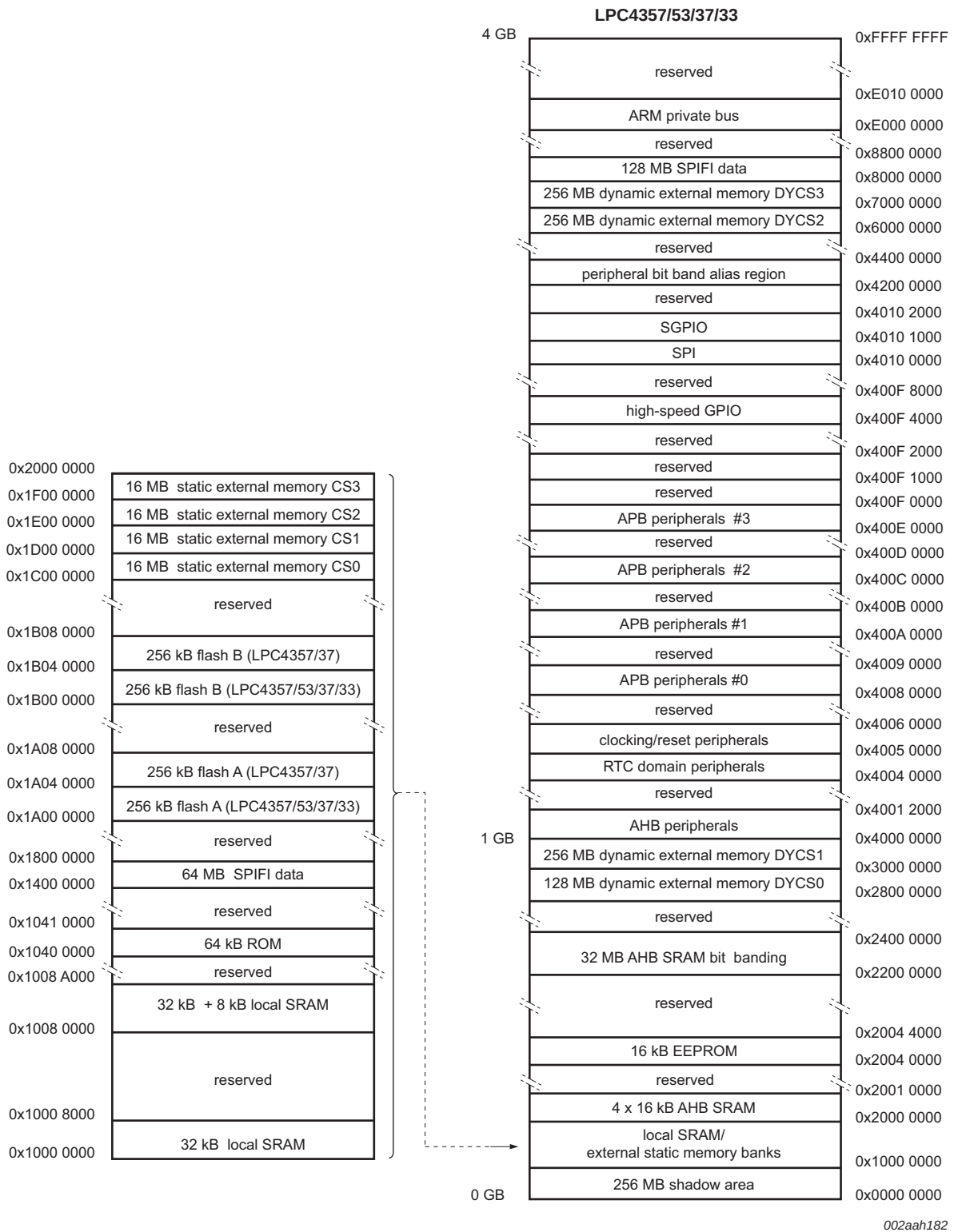
Fig 6. LPC4357/53/37/33 Memory mapping (overview)
