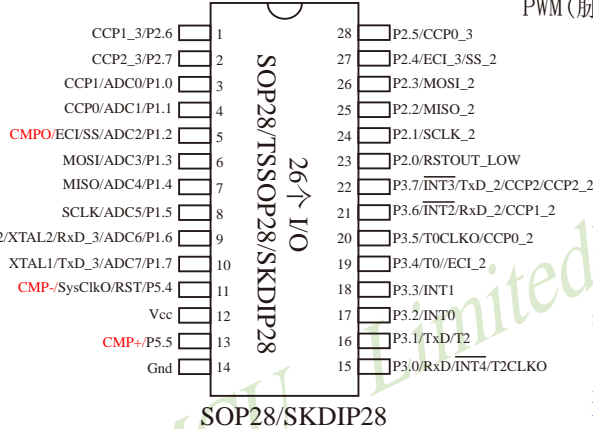
SOP28/SKDIP28
