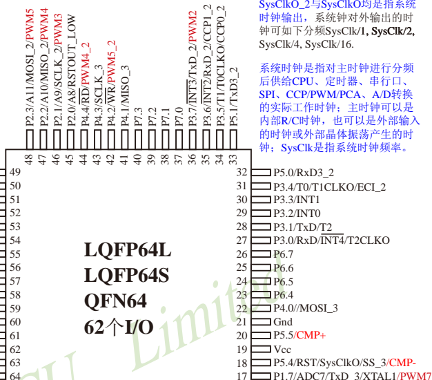
LQFP64L (16mm x 16mm)
