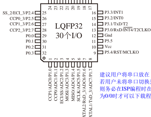
LQFP32 (9x9mm)
