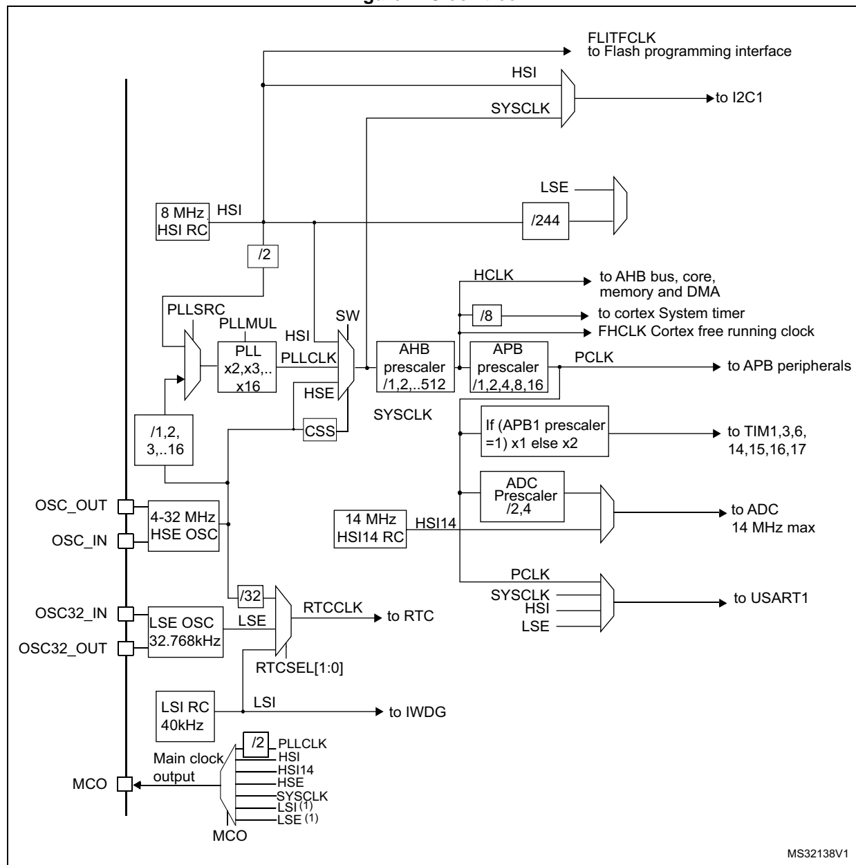
Figure 2. Clock tree
