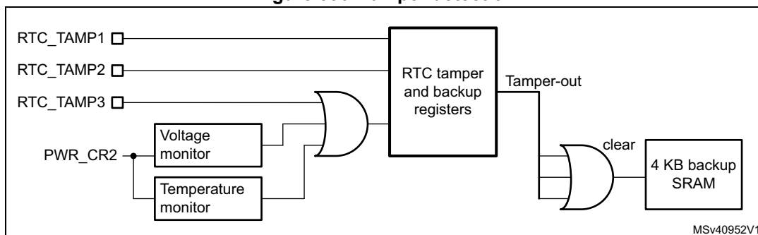
Figure 536. Tamper detection
