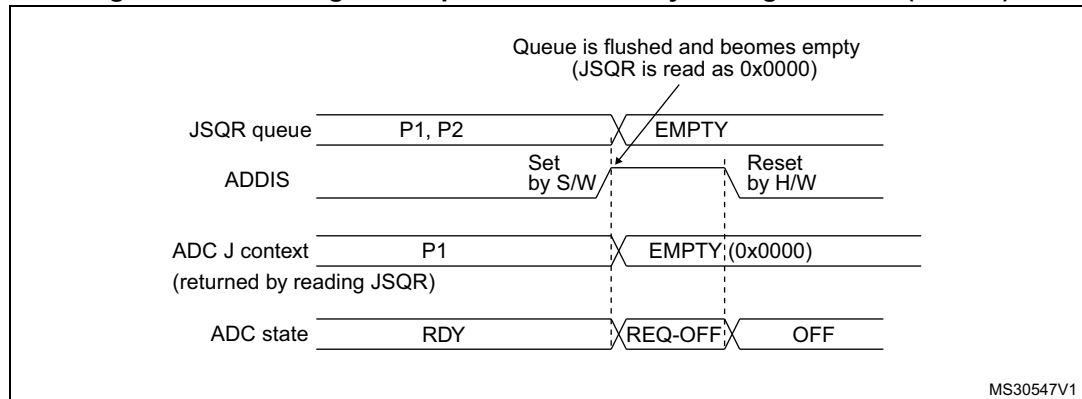
Figure 157. Flushing JSQR queue of context by setting ADDIS=1 (JQM=1)
