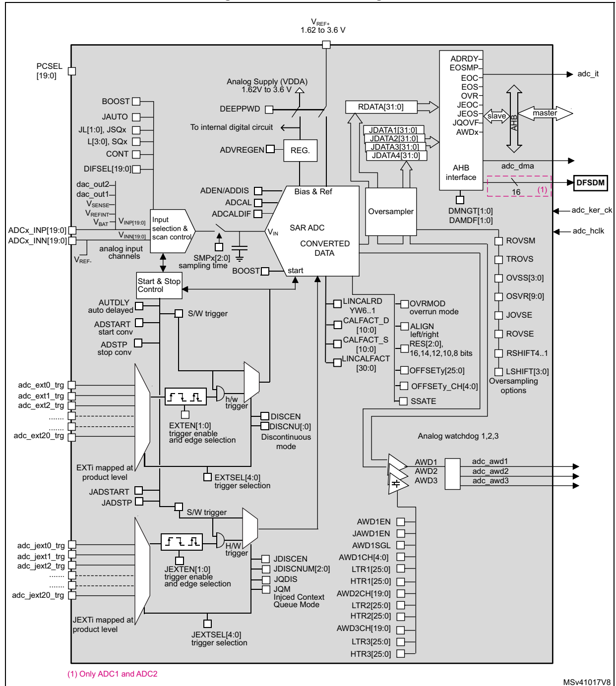
Figure 132. ADC block diagram
