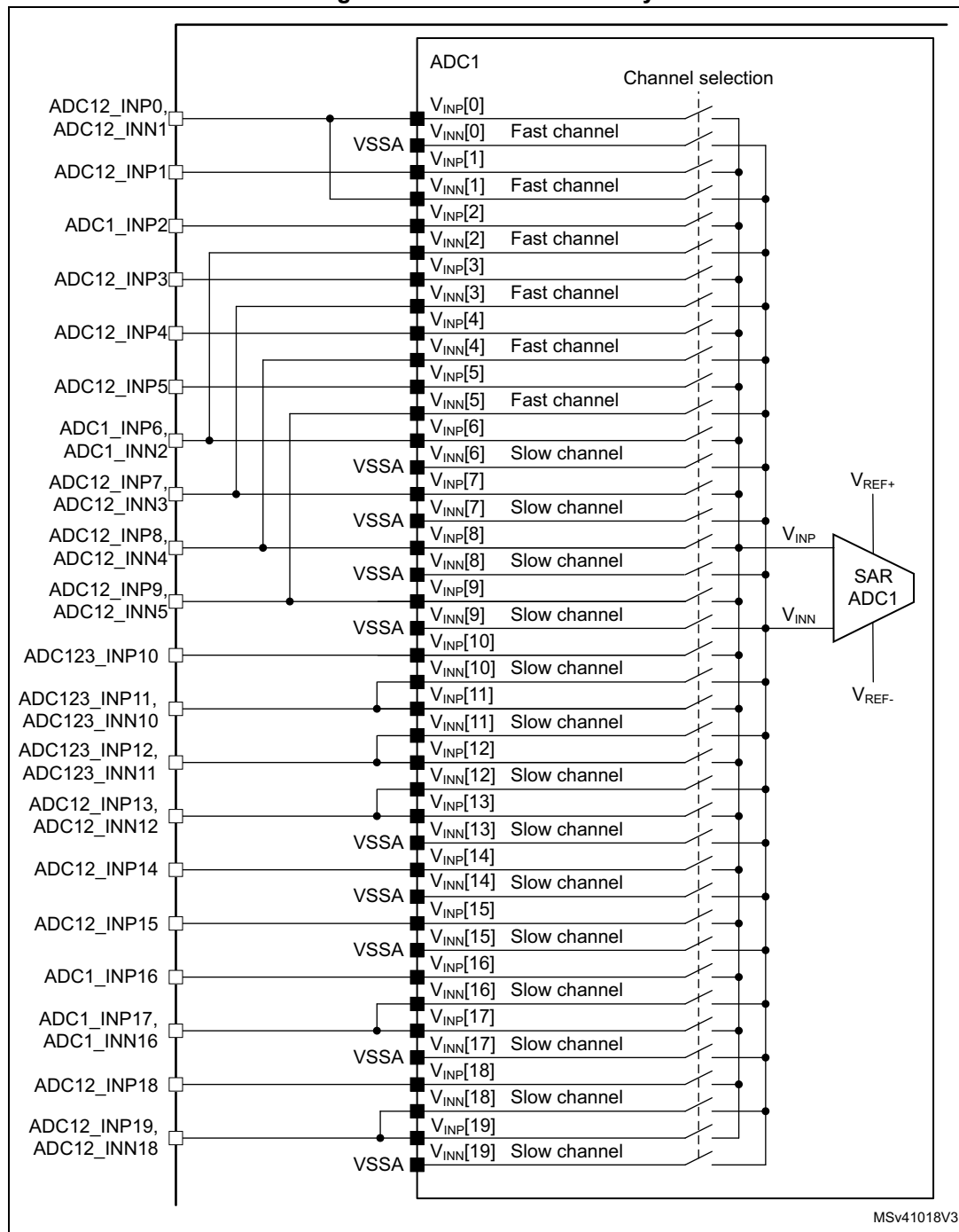
Figure 134. ADC1 connectivity
