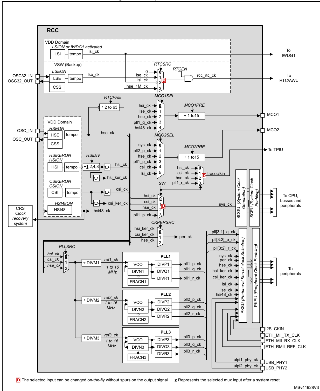
Figure 42. Top-level clock tree
