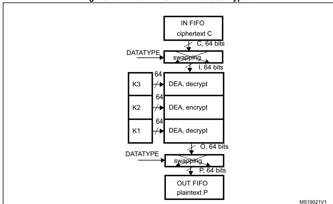
Figure 261. DES/TDES-ECB mode decryption
