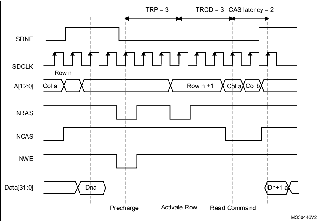
Figure 119. Read access crossing row boundary
