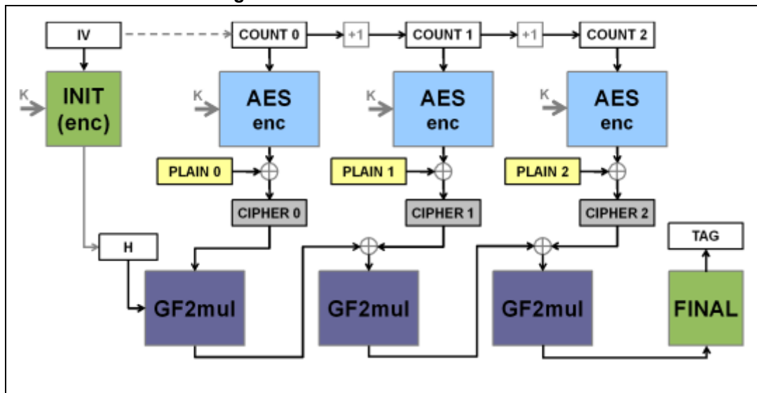
Figure 254. AES-GCM mode overview
