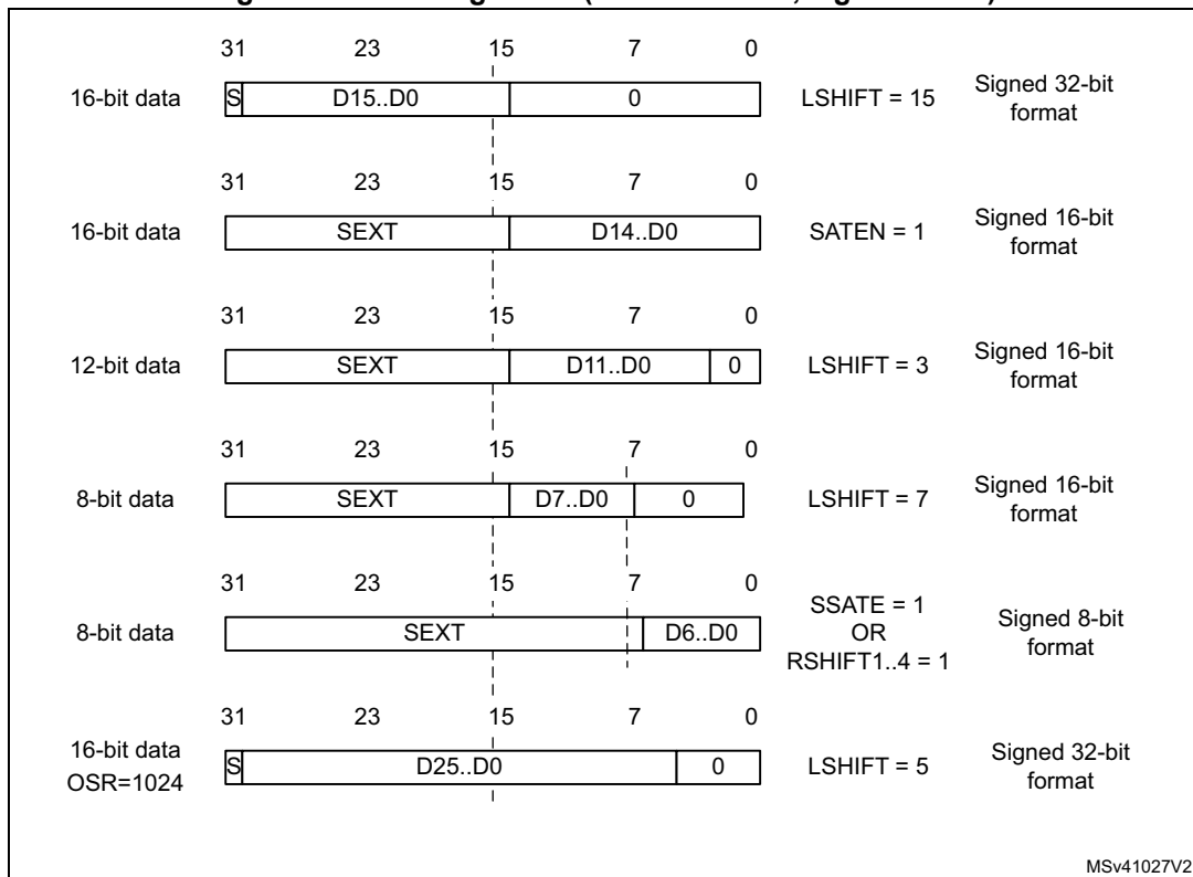
Figure 165. Left alignment (offset enabled, signed value)
