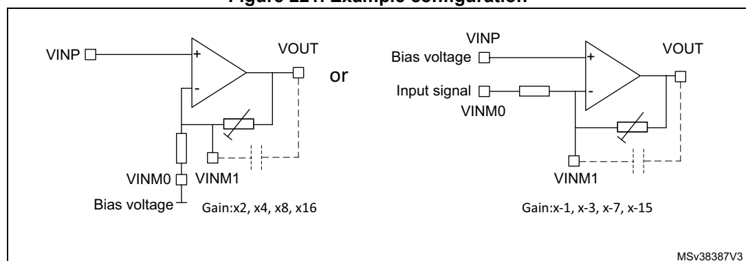
Figure 221. Example configuration
