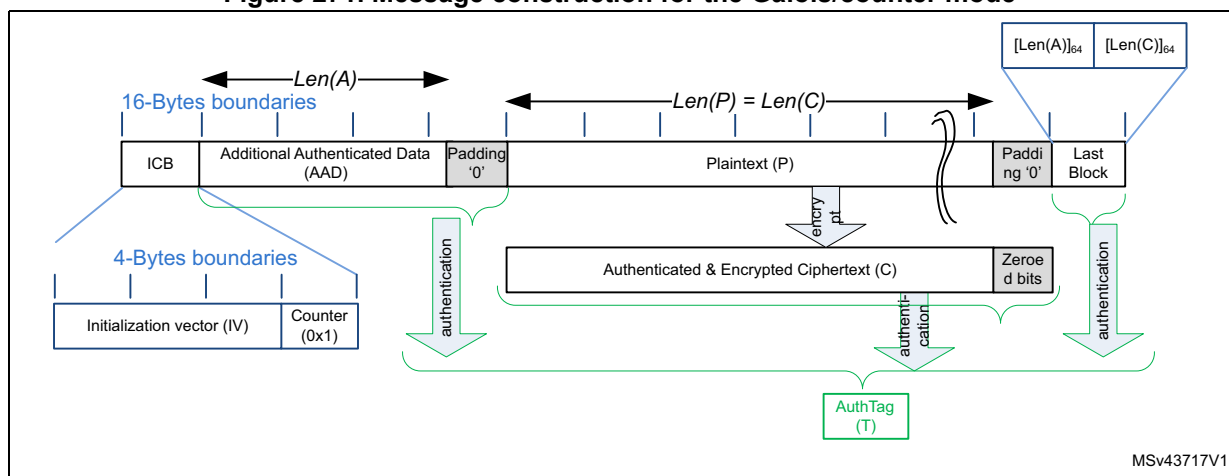
Figure 271. Message construction for the Galois/counter mode
