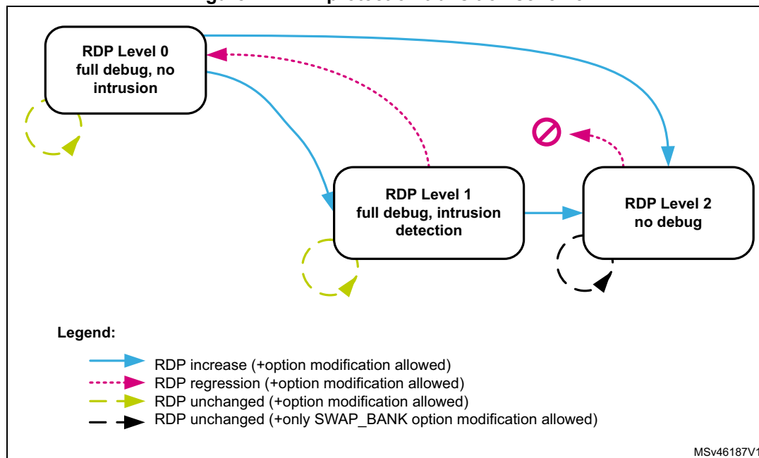
Figure 11. RDP protection transition scheme
