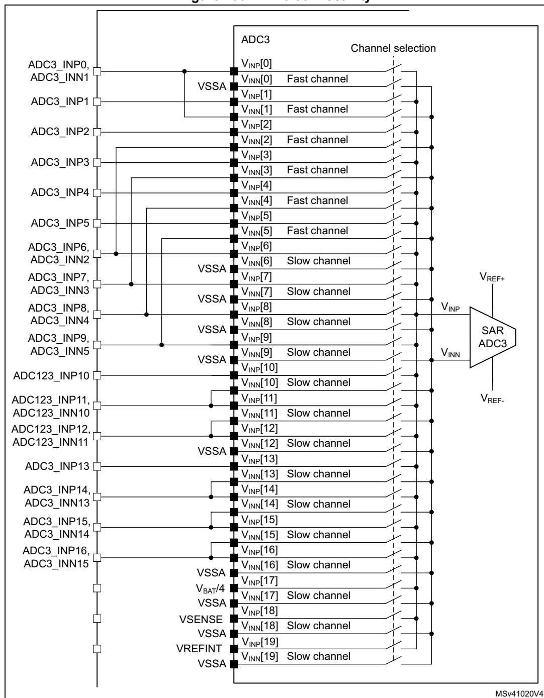
Figure 136. ADC3 connectivity
