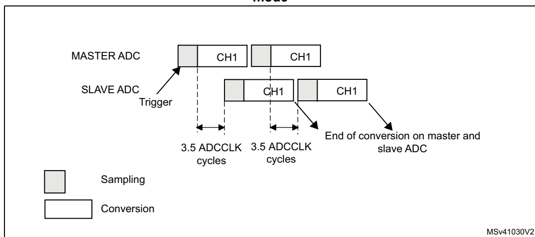
Figure 186. Interleaved mode on 1 channel in continuous conversion mode: dual ADC mode
