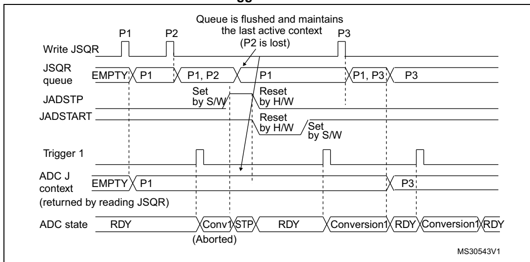
Figure 153. Flushing JSQR queue of context by setting JADSTP=1 (JQM=0). Case when JADSTP occurs during an ongoing conversion and a new trigger occurs.
