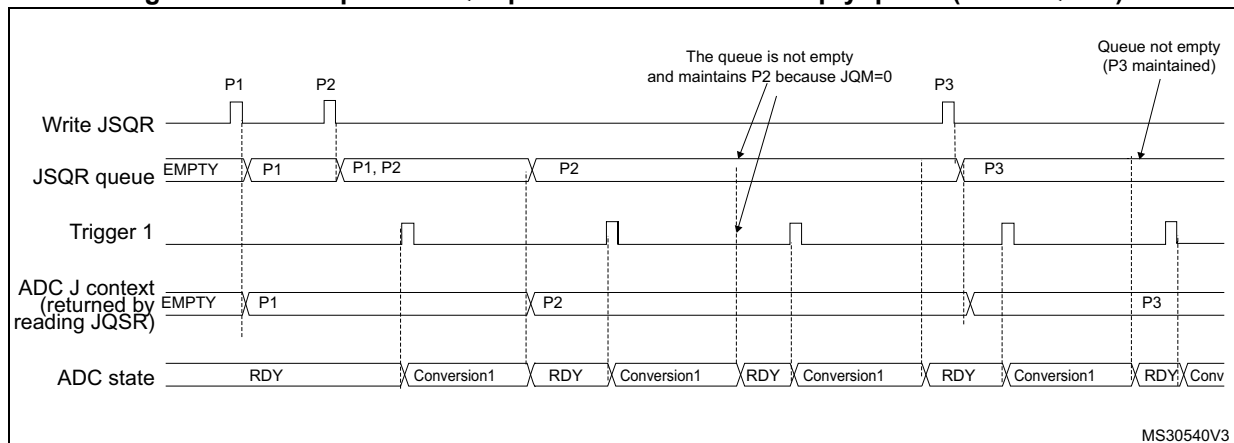
Figure 150. Example of JSQR queue of context with empty queue (case JQM=0)
