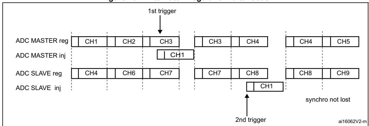
Figure 191. Alternate + regular simultaneous
