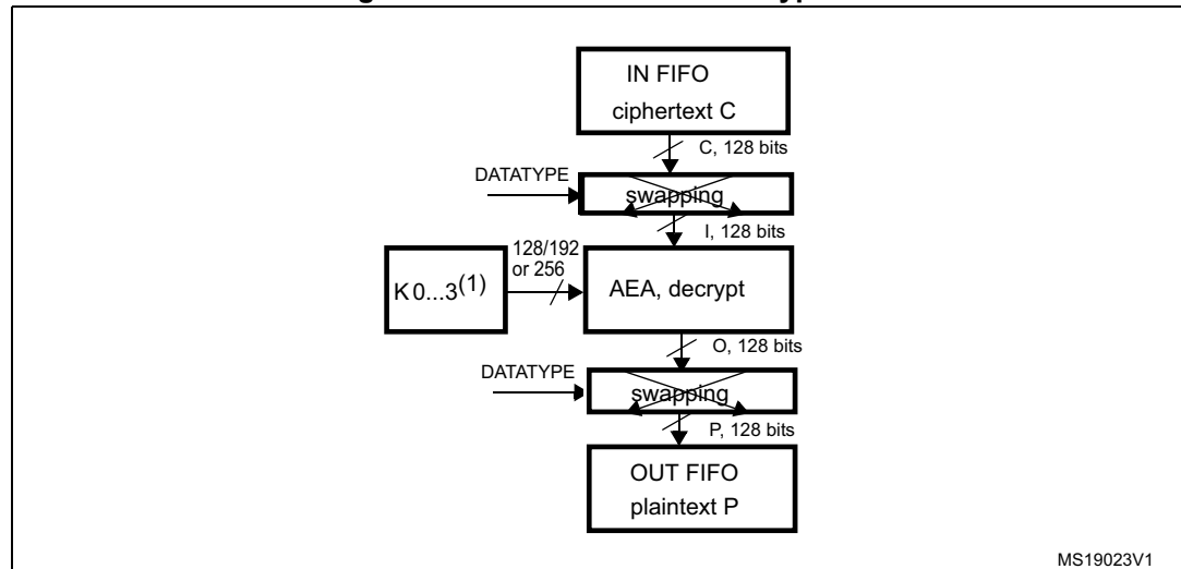
Figure 265. AES-ECB mode decryption
