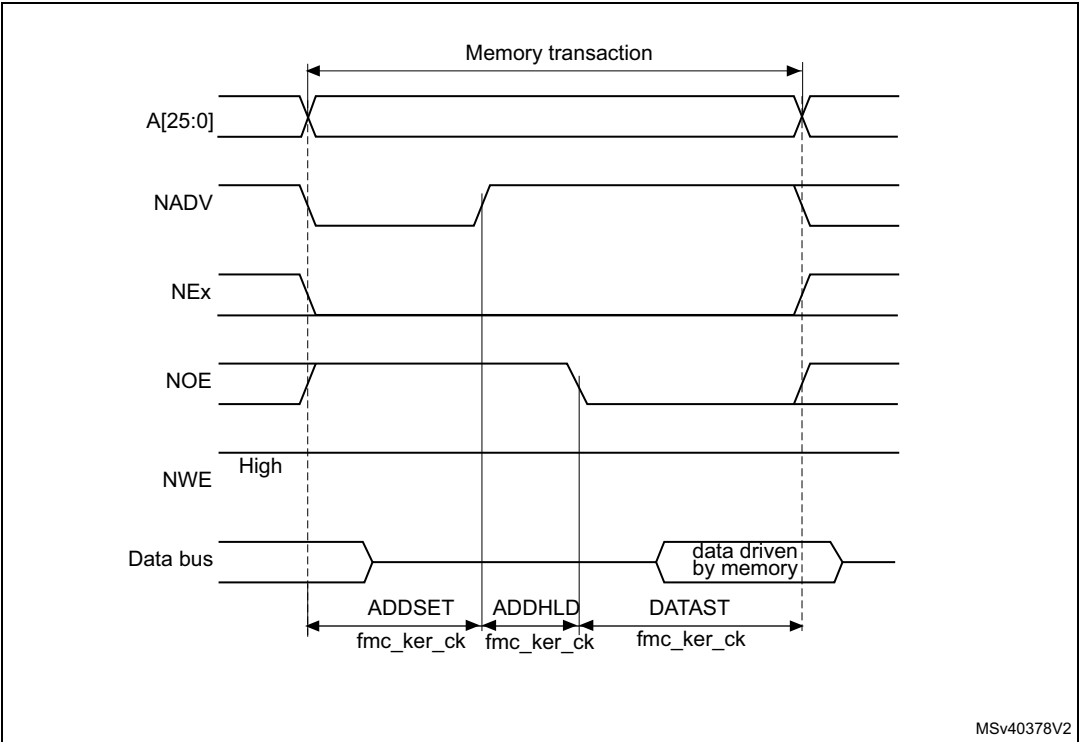
Figure 105. Mode D read access waveforms
