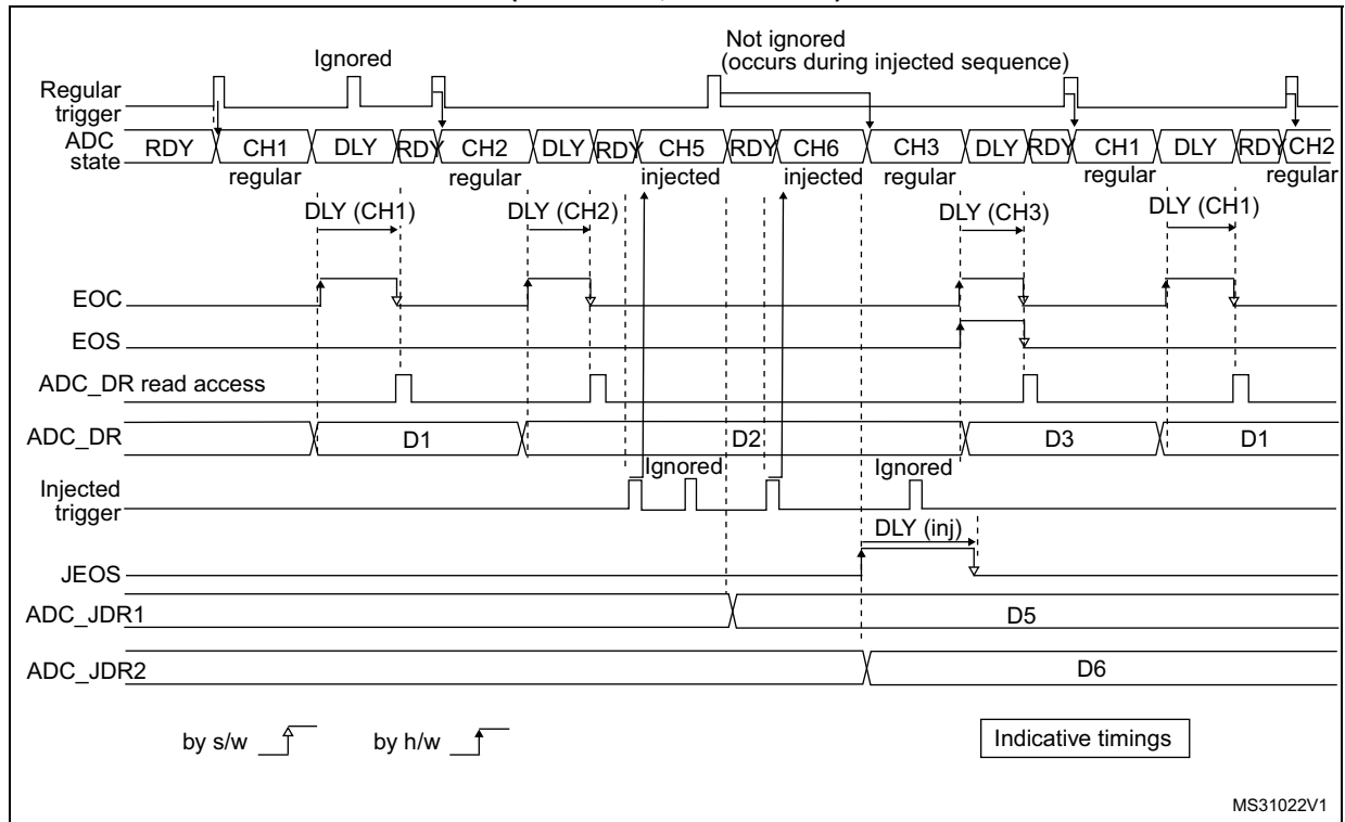
Figure 169. AUTDLY=1, regular HW conversions interrupted by injected conversions (DISCEN=1, JDISCEN=1)
