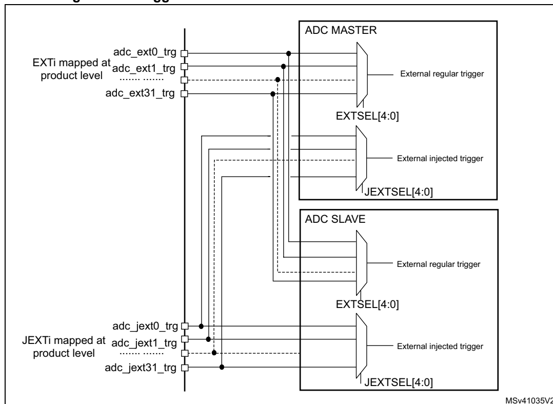
Figure 144. Triggers are shared between ADC master and ADC slave
