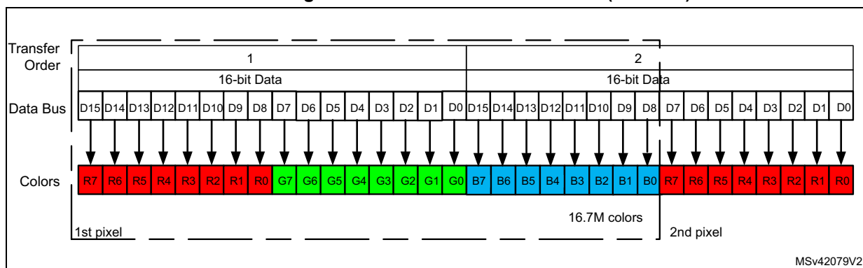
Figure 86. Intel 8080 18/24-bit mode (RGB888)
