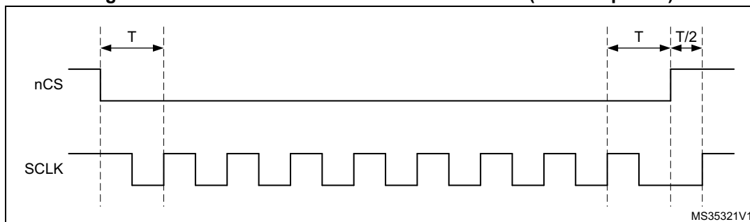
Figure 129. nCS when CKMODE = 1 in DDR mode ( T = \text{CLK period} )
