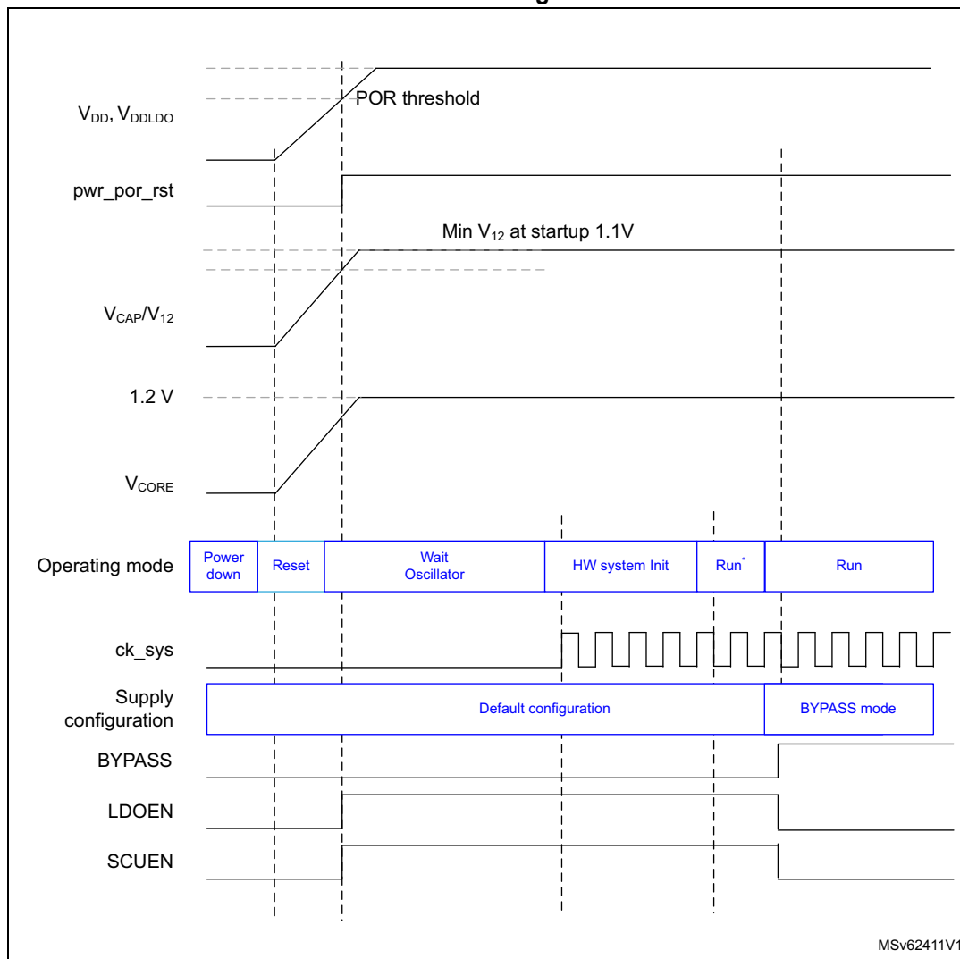
Figure 20. Device startup with V_{CORE} supplied in Bypass mode from external regulator
