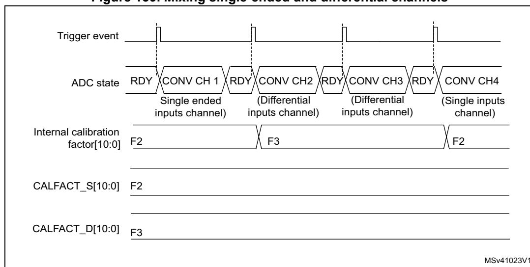
Figure 139. Mixing single-ended and differential channels
