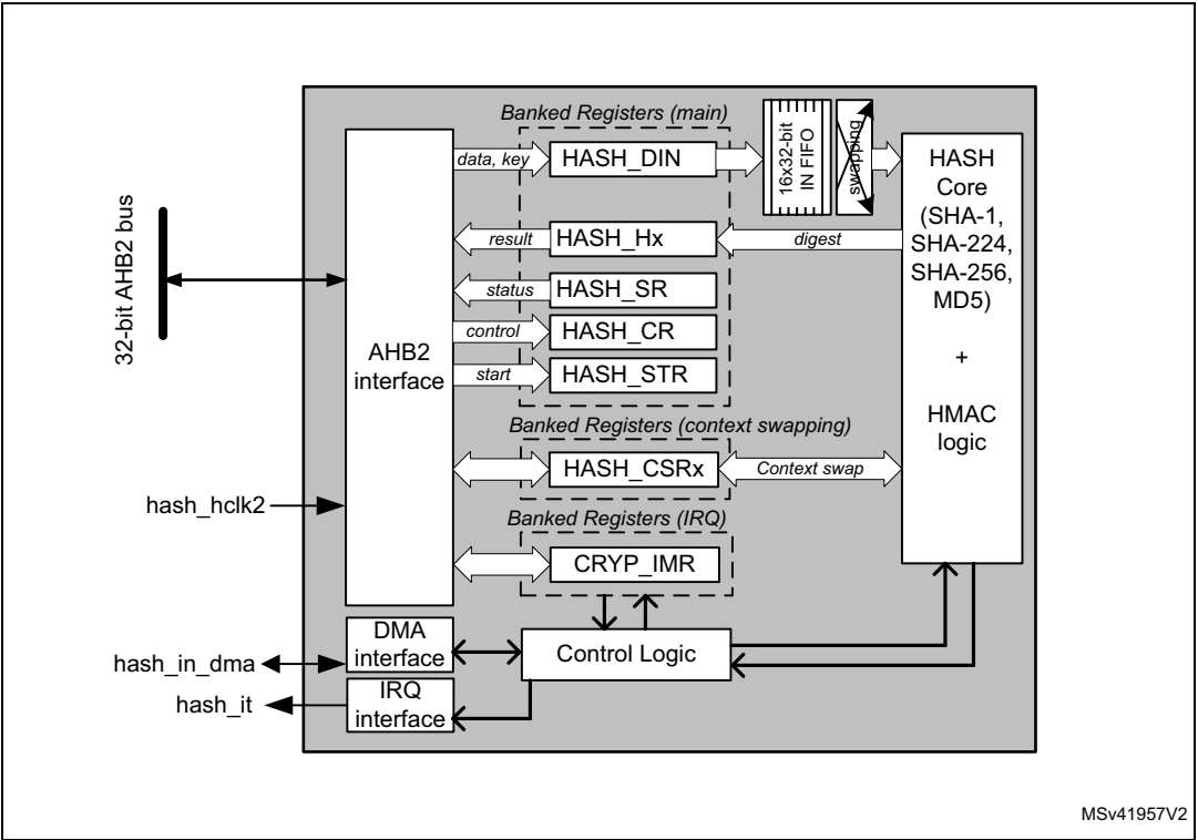
Figure 277. HASH block diagram
