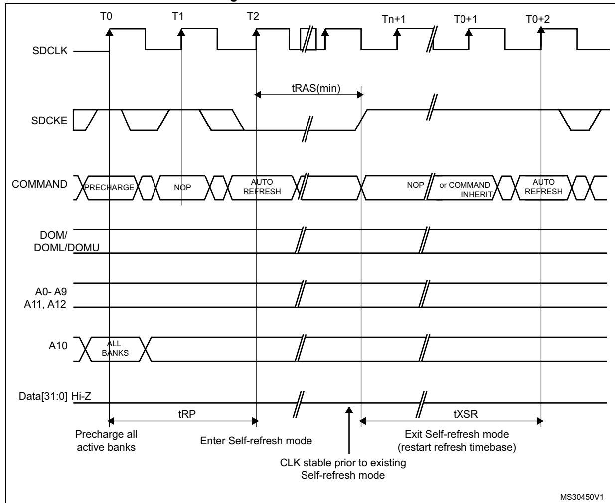
Figure 121. Self-refresh mode
