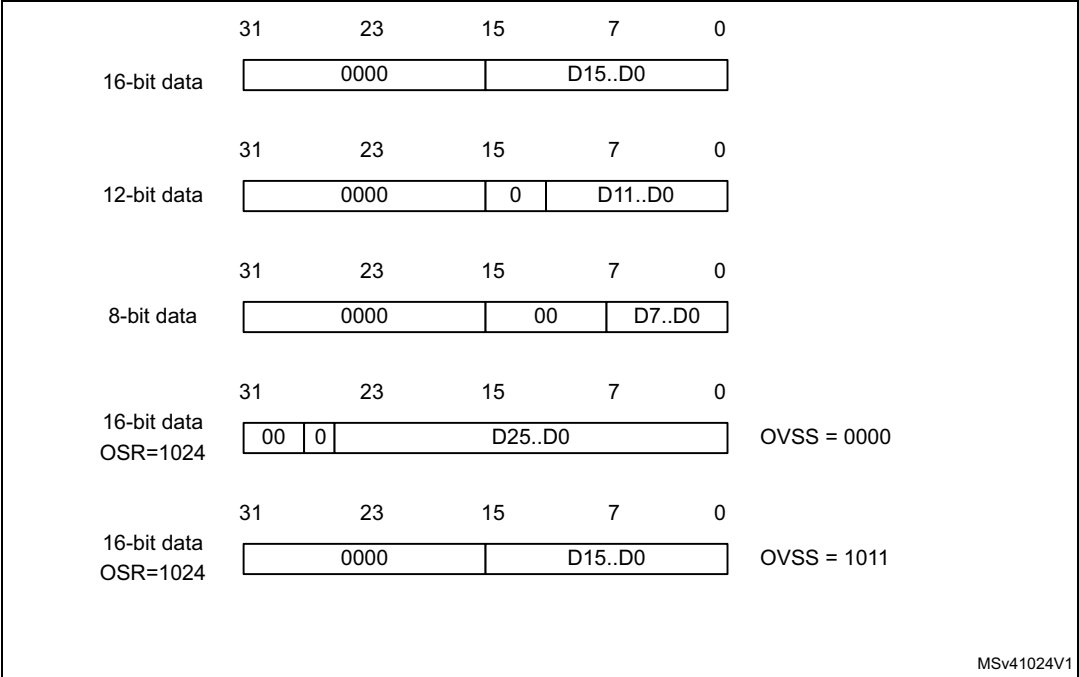
Figure 162. Right alignment (offset disabled, unsigned value)
