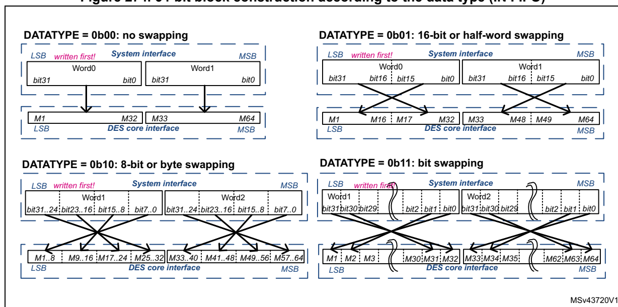
Figure 274. 64-bit block construction according to the data type (IN FIFO)
