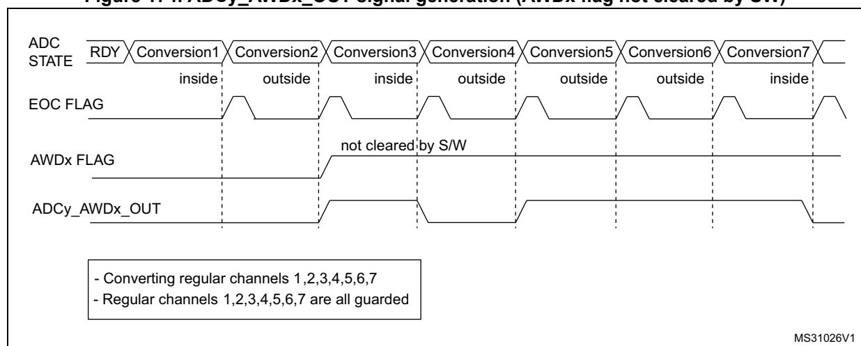
Figure 174. ADCy_AWDx_OUT signal generation (AWDx flag not cleared by SW)
