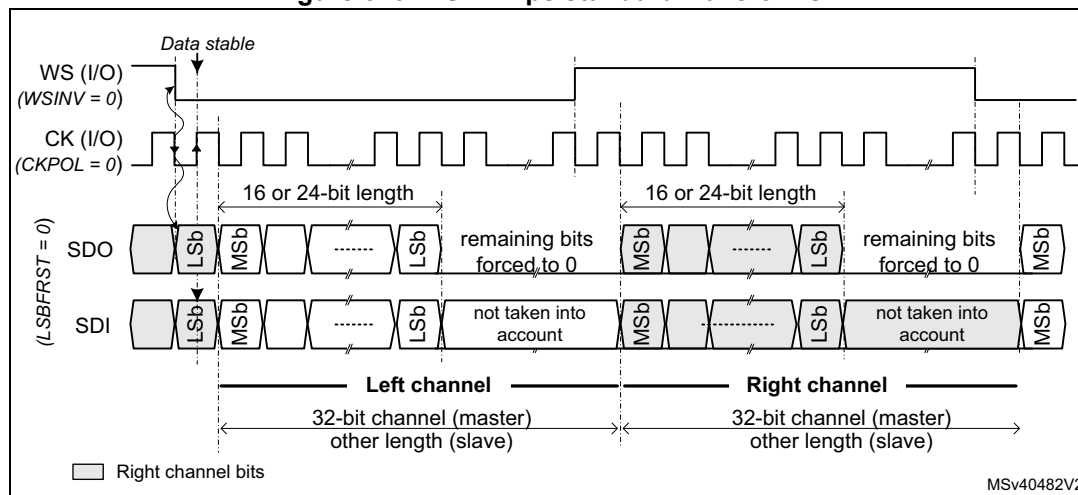
Figure 626. I2S Philips standard waveforms
