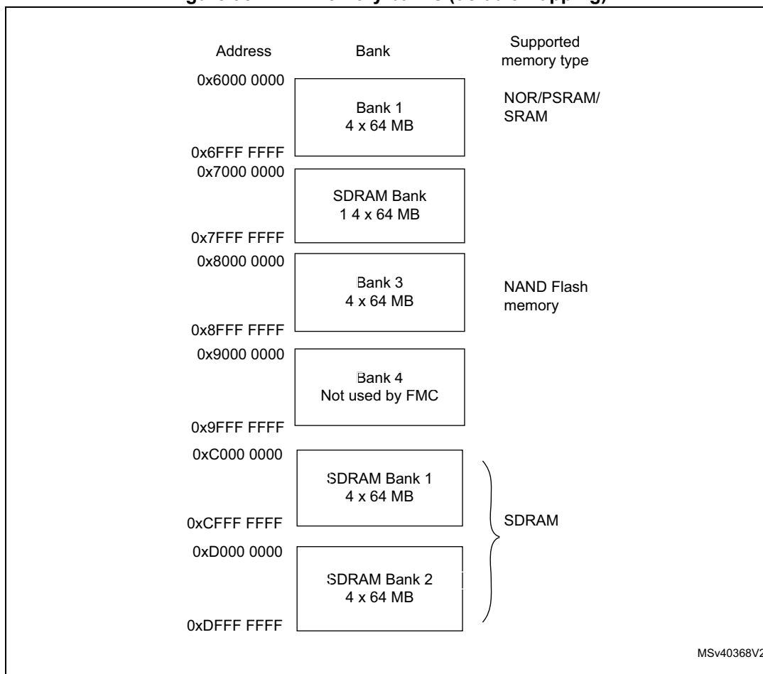
Figure 95. FMC memory banks (default mapping)
