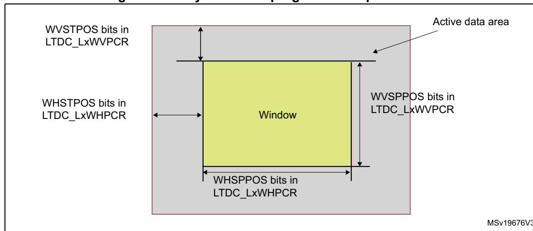
Figure 243. Layer window programmable parameters
