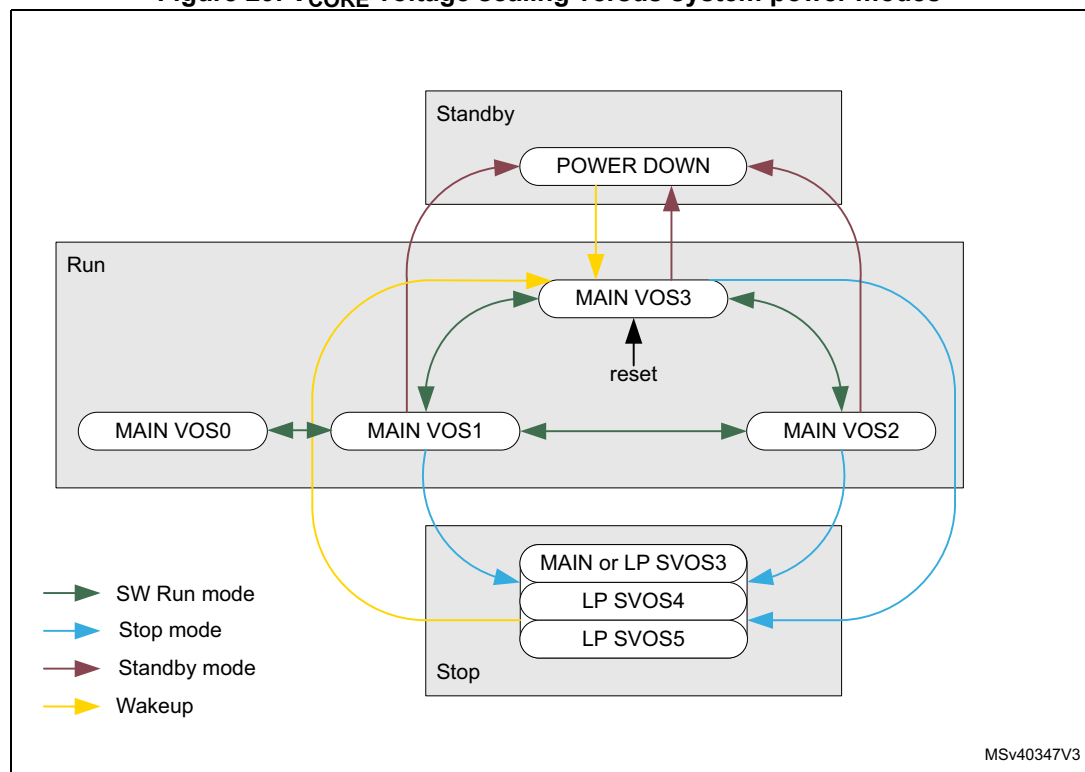
Figure 29. V_{CORE} voltage scaling versus system power modes
