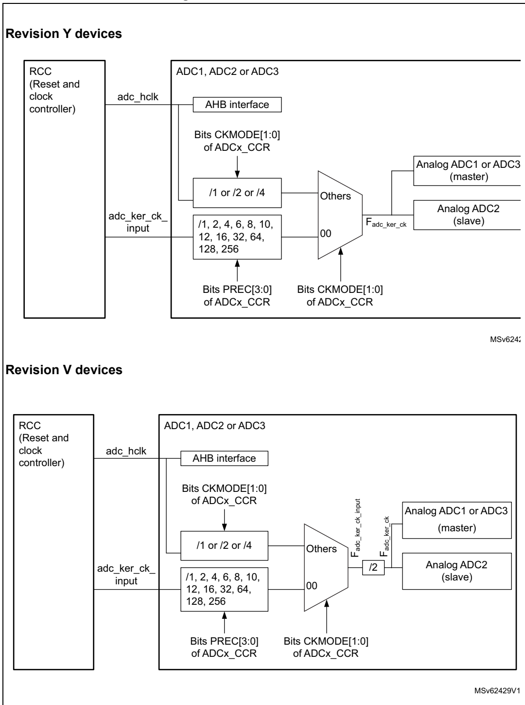
Figure 133. ADC clock scheme
