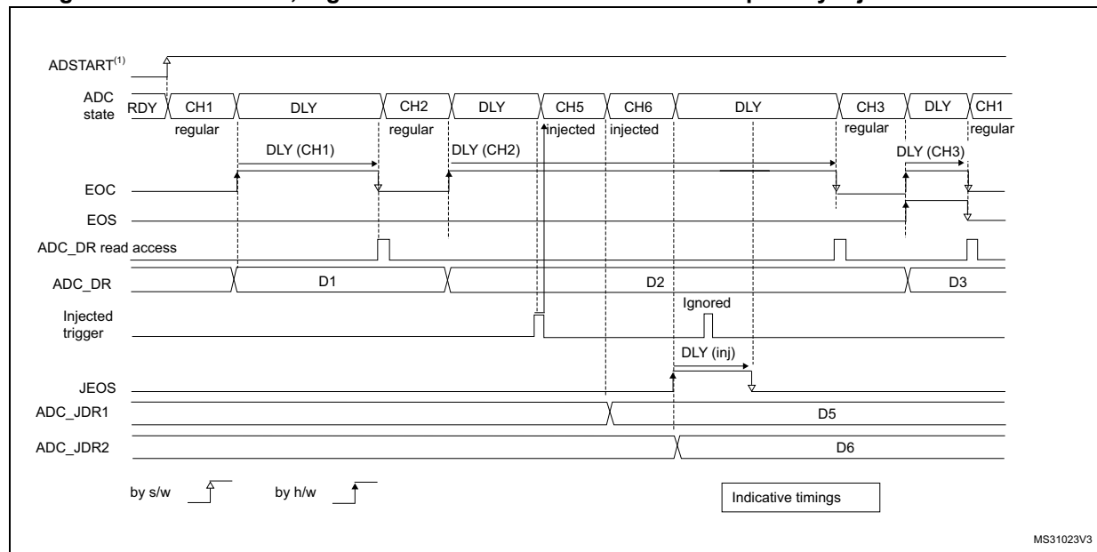
Figure 170. AUTDLY=1, regular continuous conversions interrupted by injected conversions
