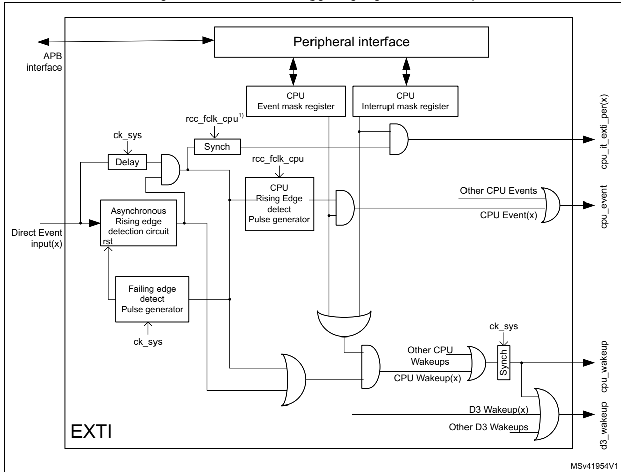
Figure 90. Direct event triggering logic CPU Wakeup
