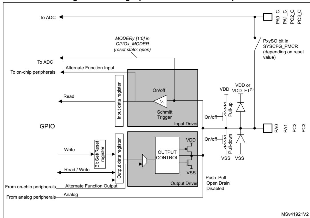
Figure 73. Analog inputs connected to ADC inputs
