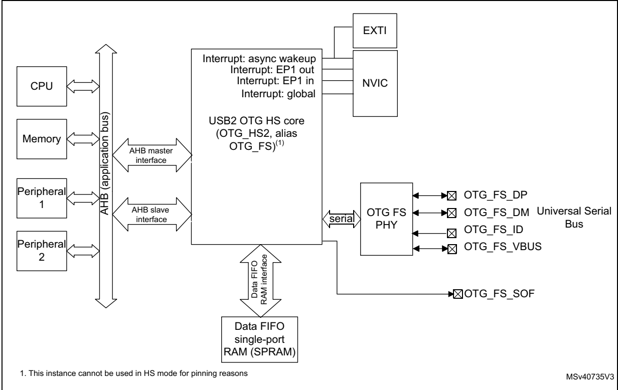
Figure 748. USB2 OTG high-speed block diagram (OTG_HS2)
