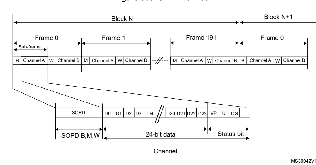
Figure 658. SPDIF format
