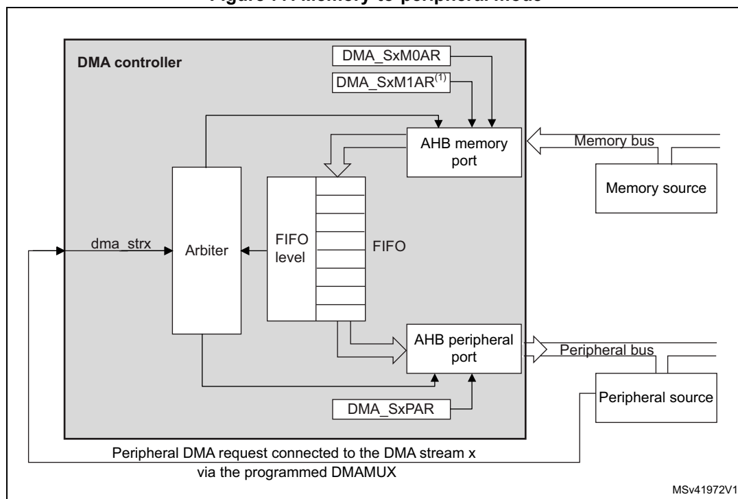
Figure 77. Memory-to-peripheral mode
