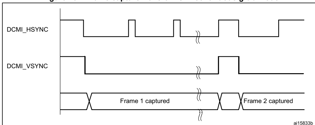
Figure 237. Frame capture waveforms in continuous grab mode
