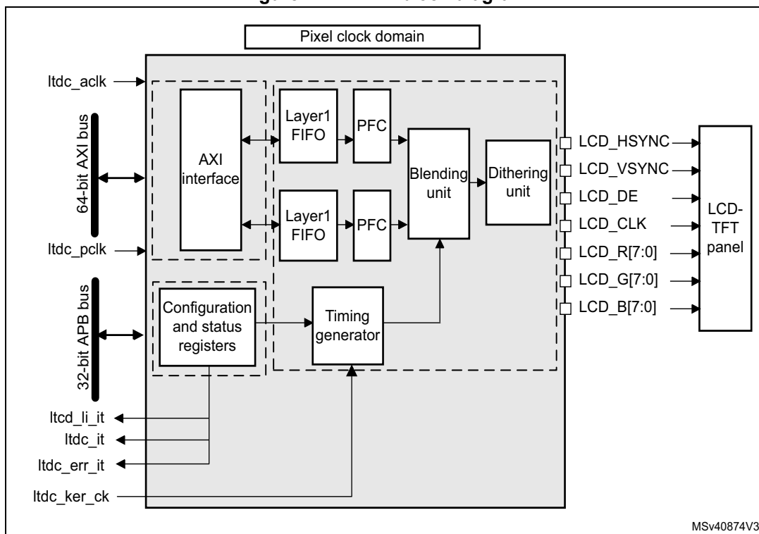
Figure 241. LTDC block diagram
