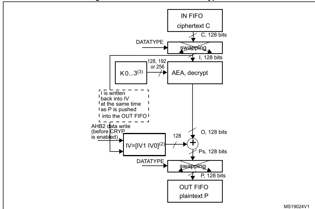
Figure 267. AES-CBC mode decryption
