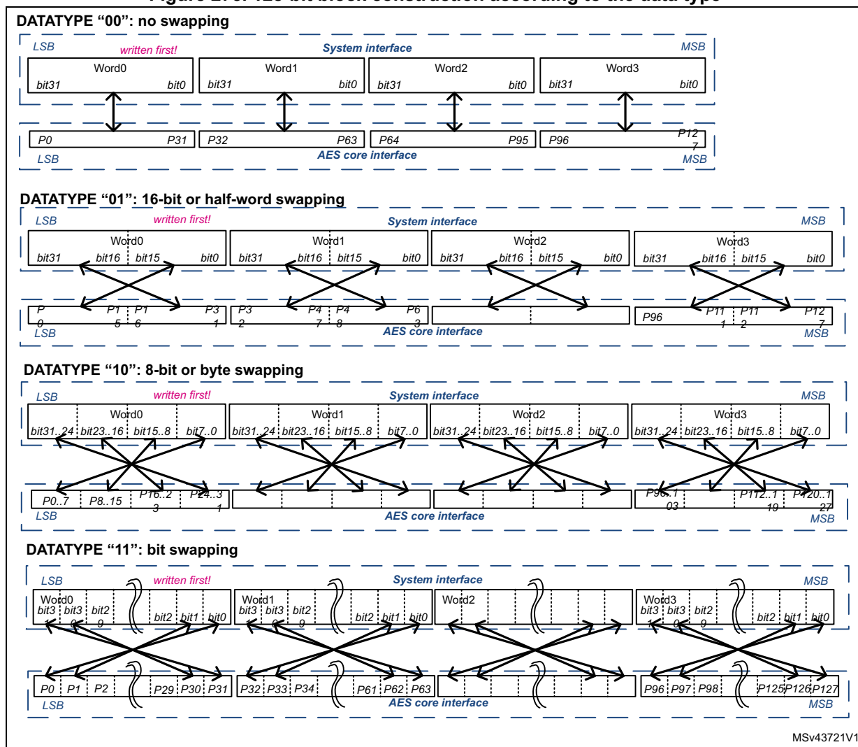
Figure 275. 128-bit block construction according to the data type
