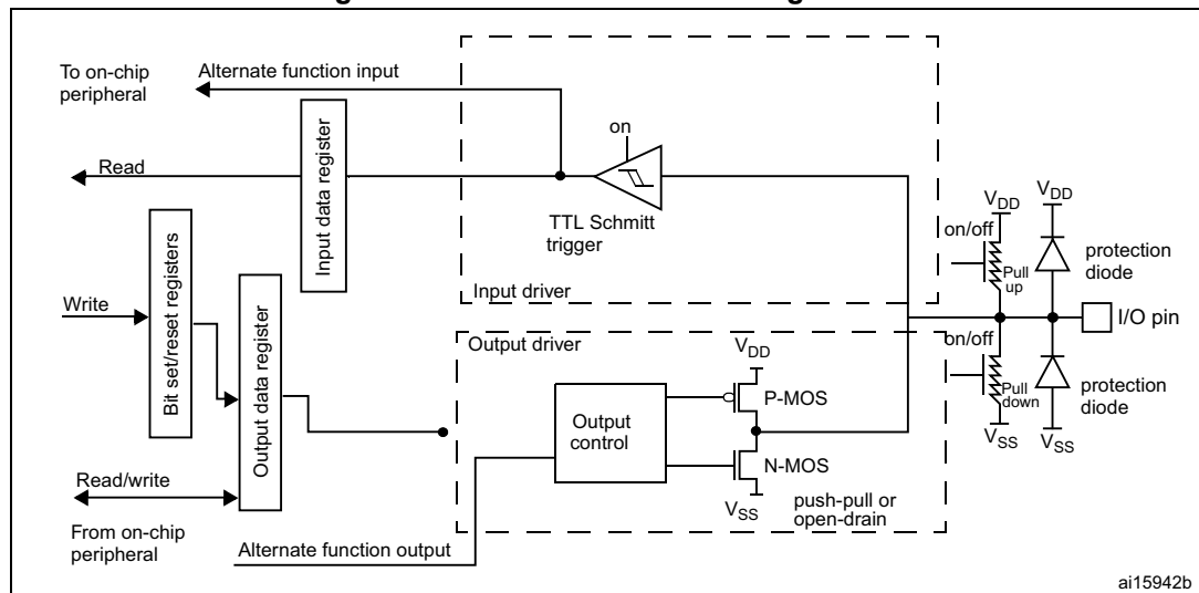
Figure 71. Alternate function configuration
