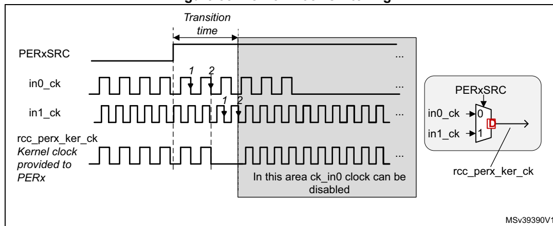
Figure 58. Kernel Clock switching
