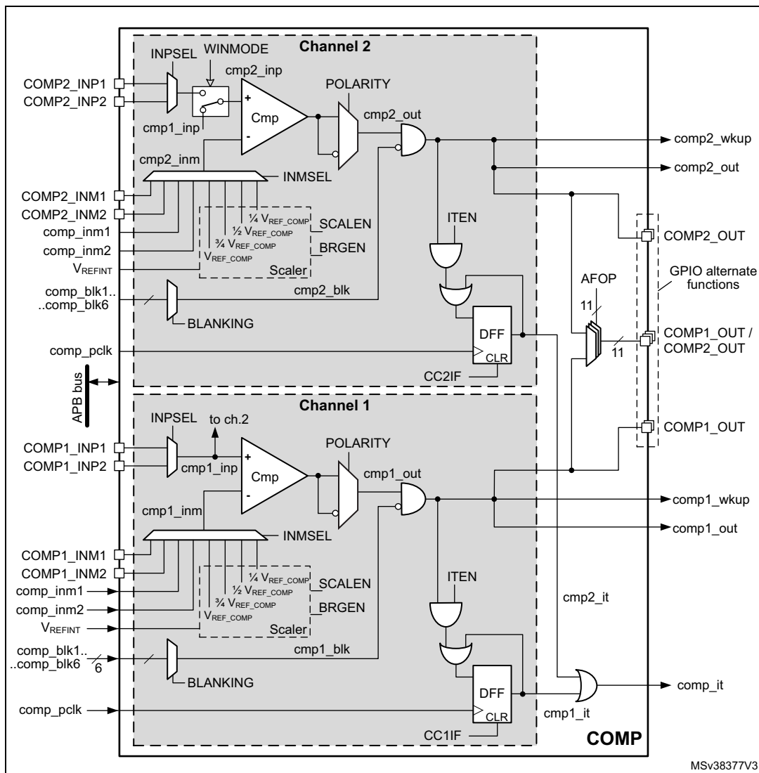
Figure 211. Comparator functional block diagram
