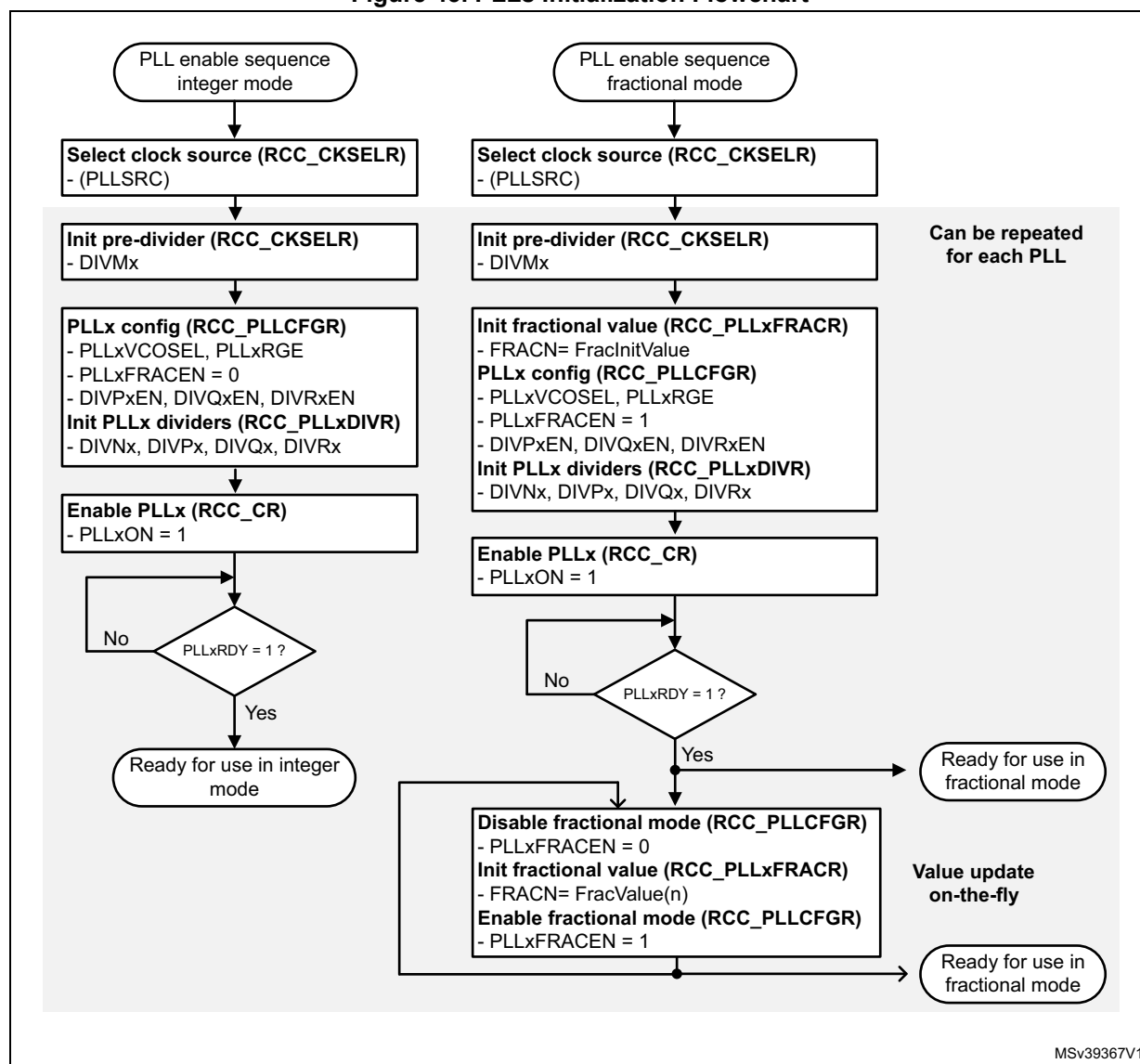
Figure 45. PLLs Initialization Flowchart
