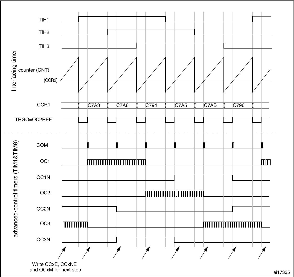
Figure 399. Example of Hall sensor interface
