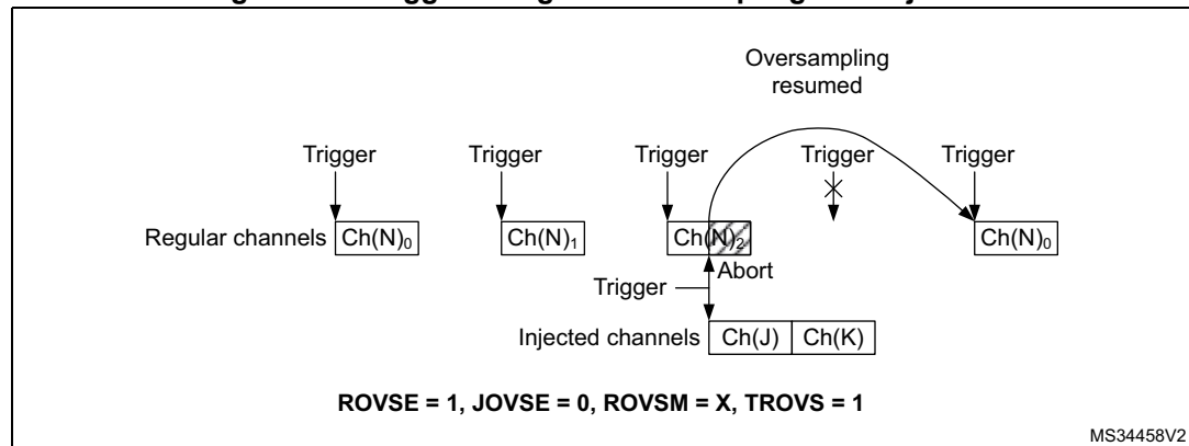
Figure 181. Triggered regular oversampling with injection
