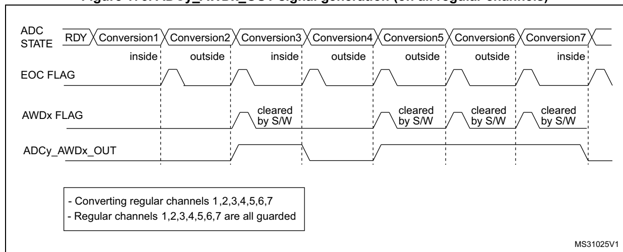
Figure 173. ADCy_AWDx_OUT signal generation (on all regular channels)
