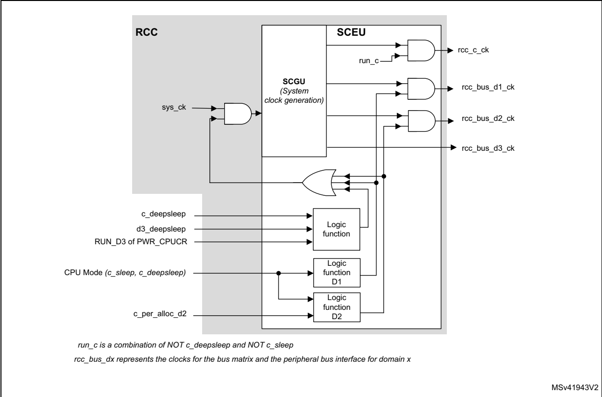
Figure 60. Bus clock enable logic
