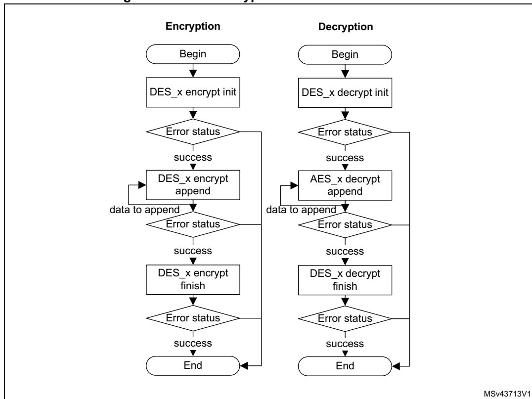
Figure 257. STM32 cryptolib DES/TDES flowcharts
