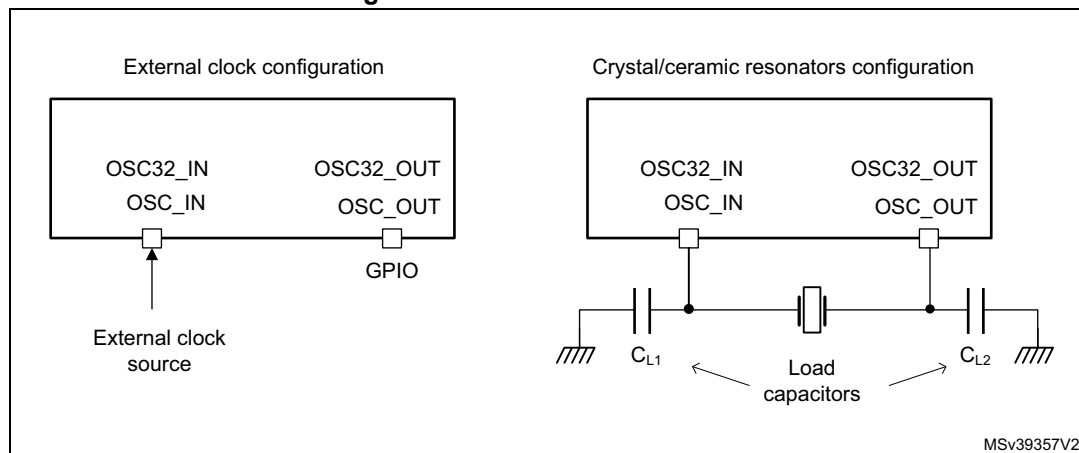
Figure 43. HSE/LSE clock source
