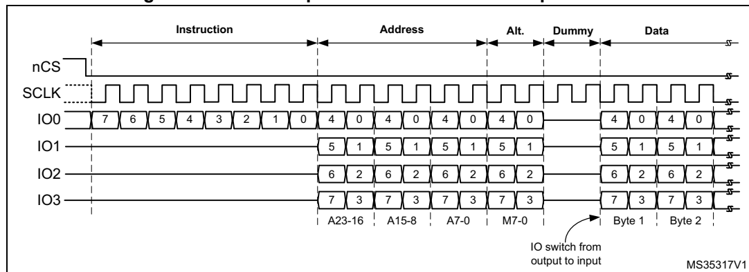
Figure 125. An example of a read command in quad mode
