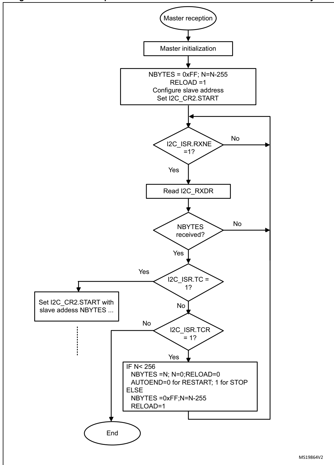
Figure 558. Transfer sequence flowchart for I2C master receiver for N &gt; 255 bytes
