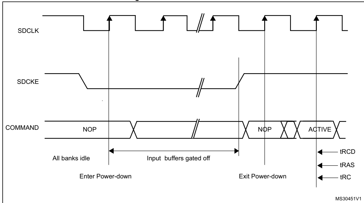
Figure 122. Power-down mode
