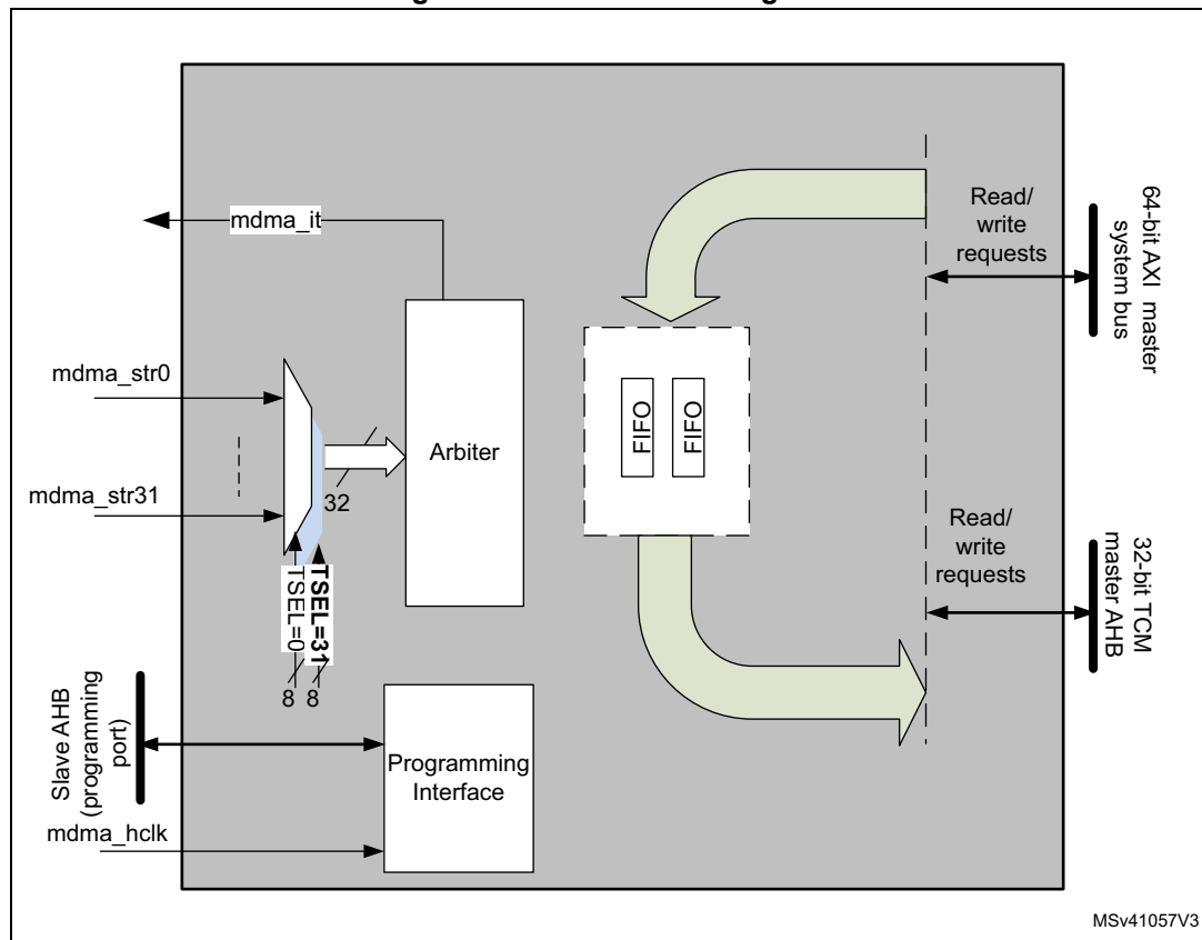
Figure 74. MDMA block diagram
