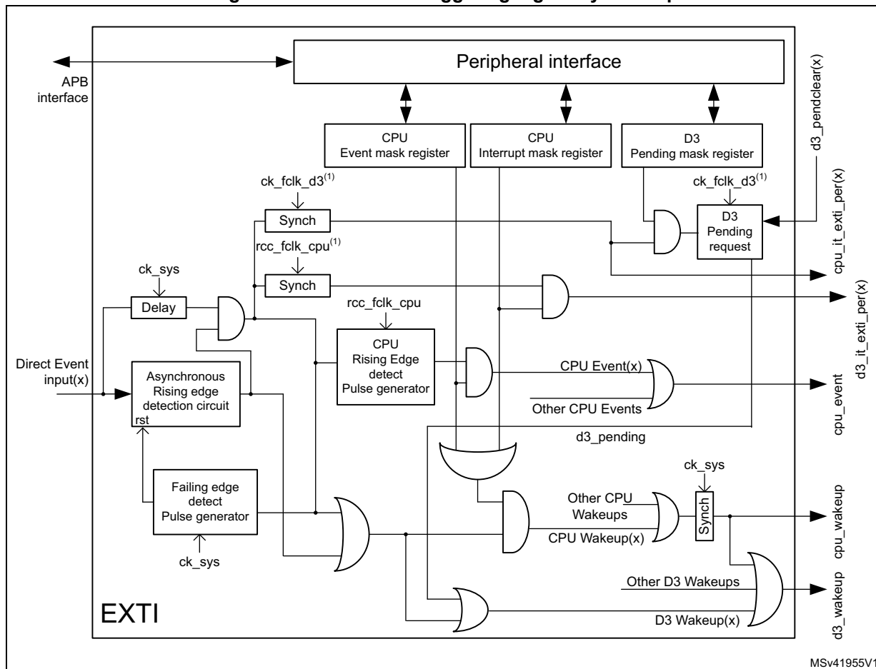
Figure 91. Direct event triggering logic Any Wakeup
