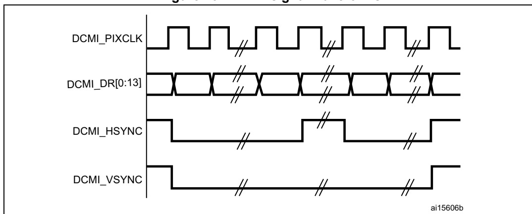
Figure 234. DCMI signal waveforms
