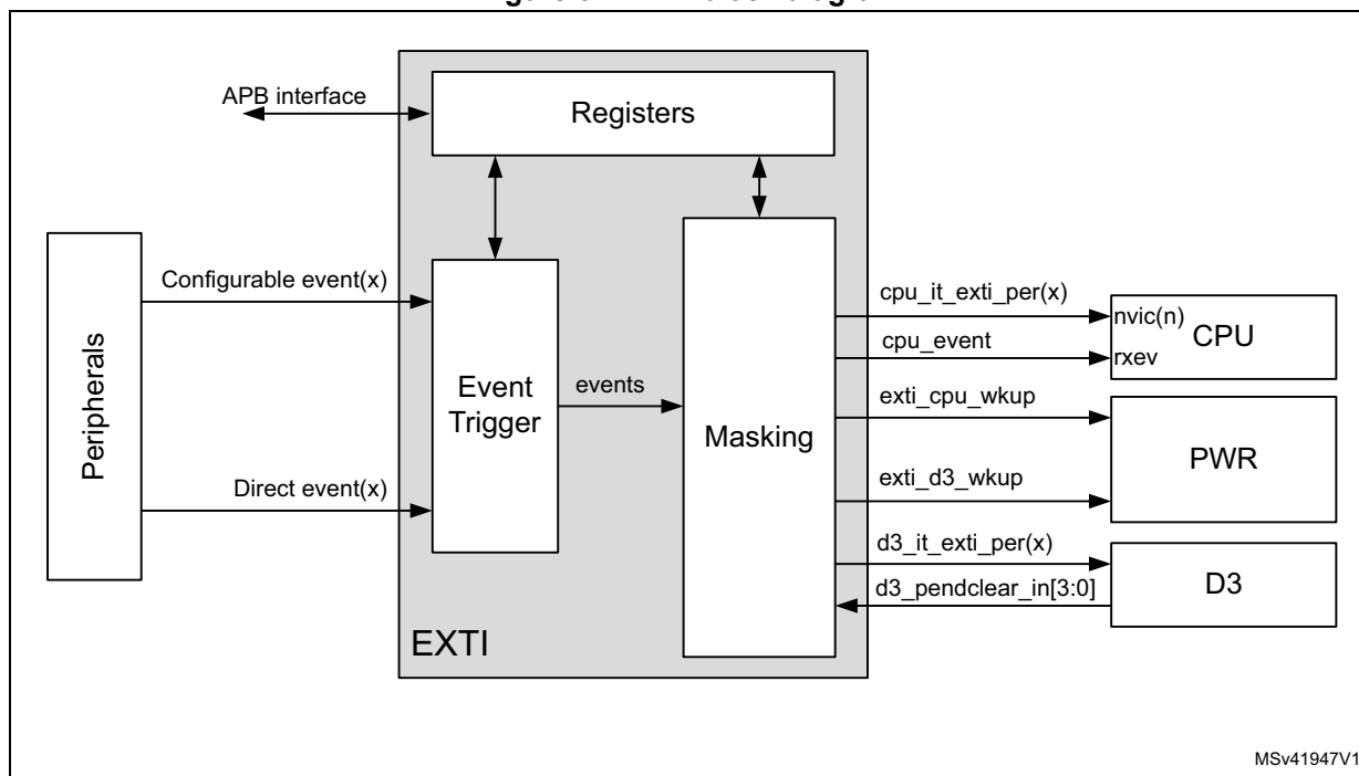
Figure 87. EXTI block diagram
