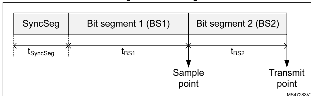
Figure 740. Bit timing
