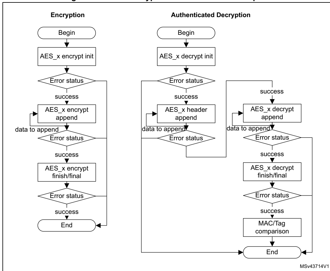
Figure 258. STM32 cryptolib AES flowchart examples
