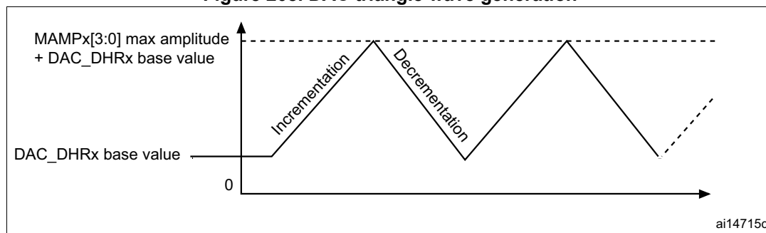
Figure 208. DAC triangle wave generation
