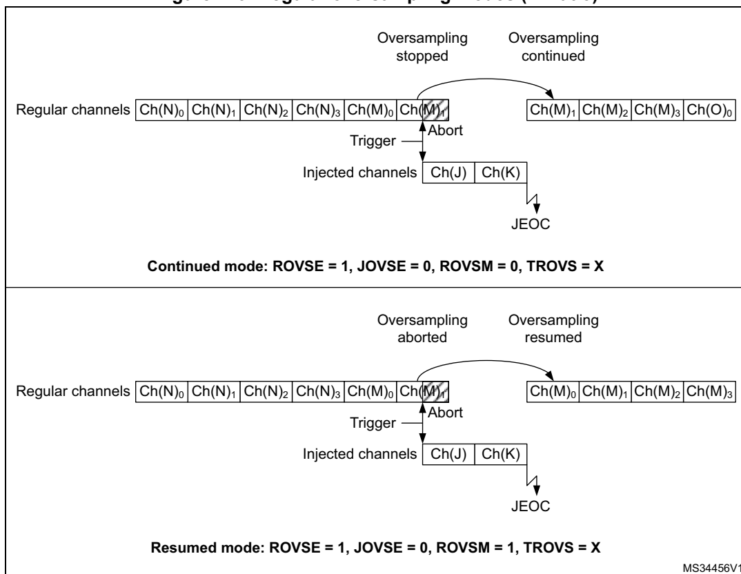
Figure 179. Regular oversampling modes (4x ratio)
