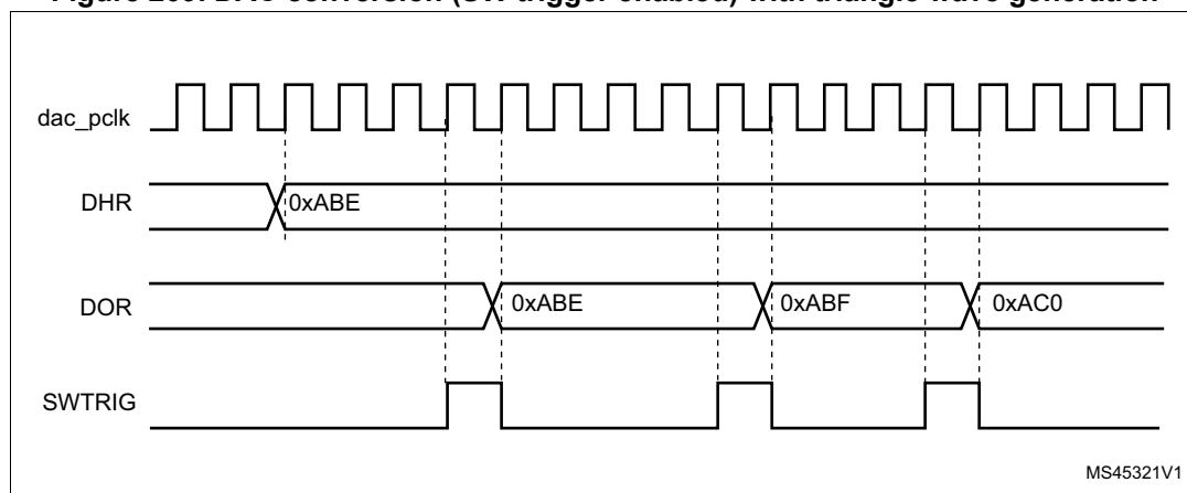
Figure 209. DAC conversion (SW trigger enabled) with triangle wave generation
