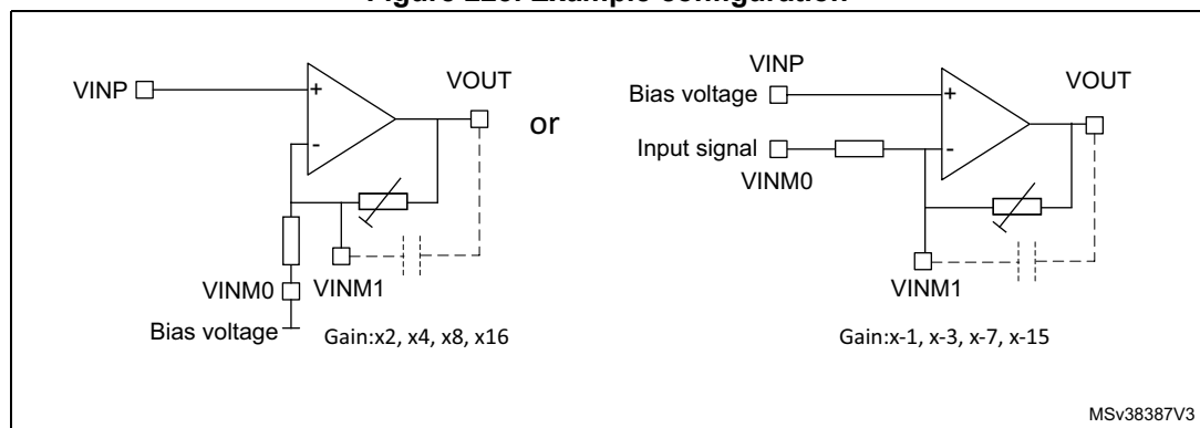
Figure 223. Example configuration
