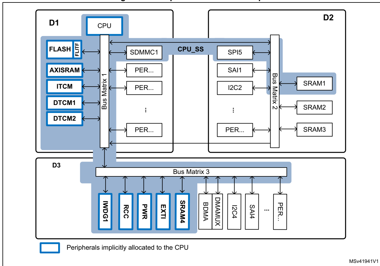
Figure 57. Peripheral allocation example
