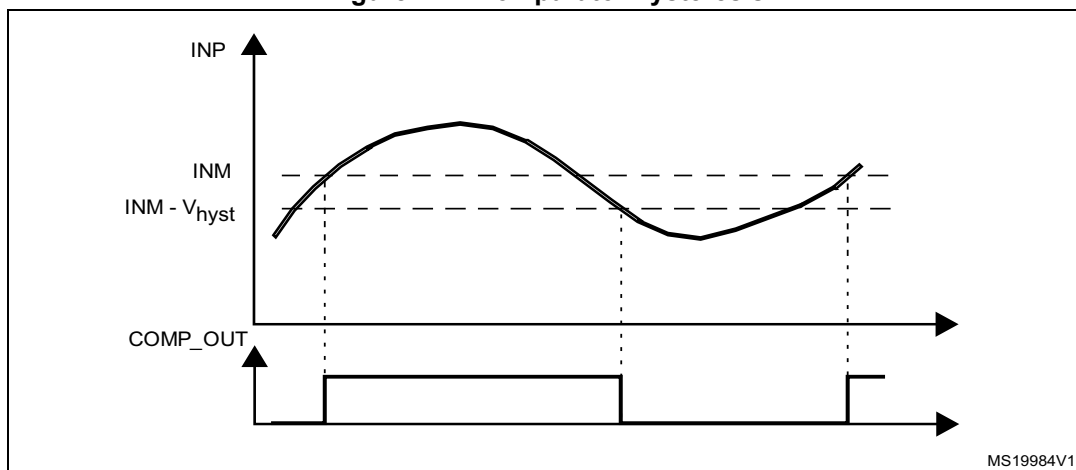
Figure 212. Comparator hysteresis
