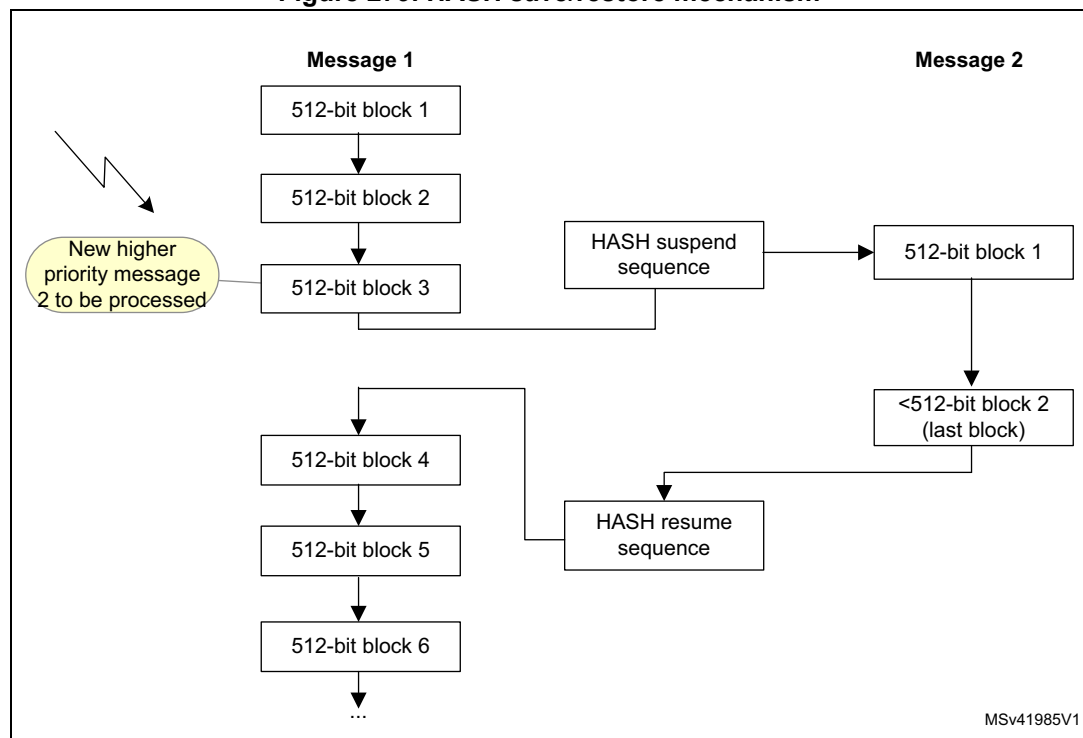
Figure 279. HASH save/restore mechanism
