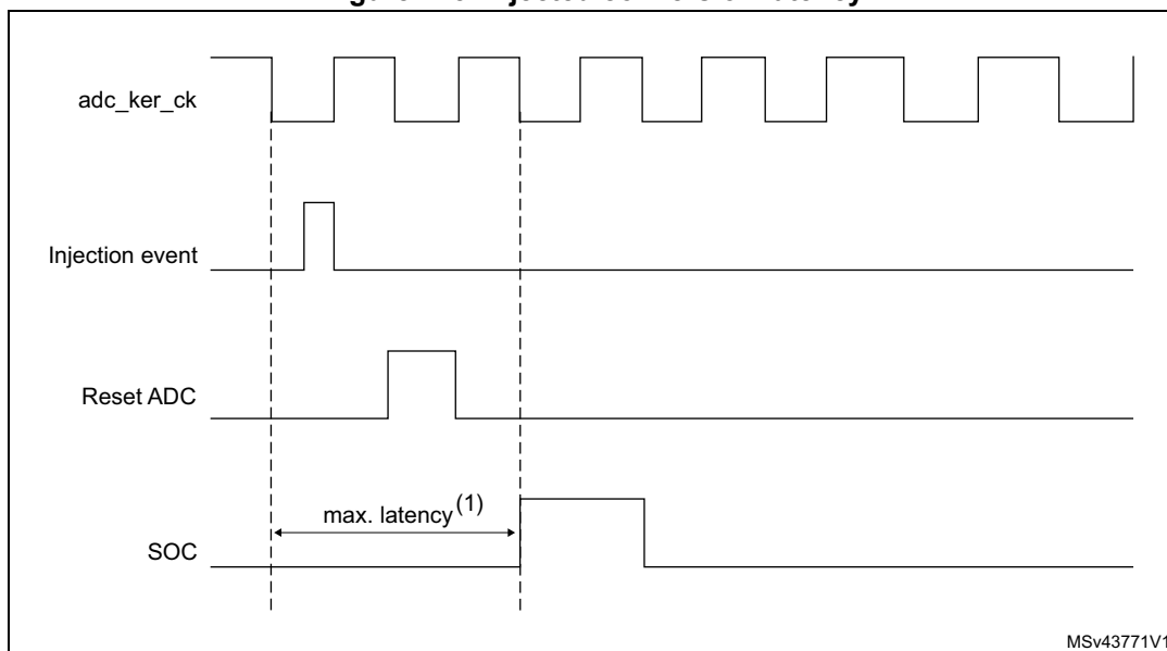
Figure 145. Injected conversion latency
