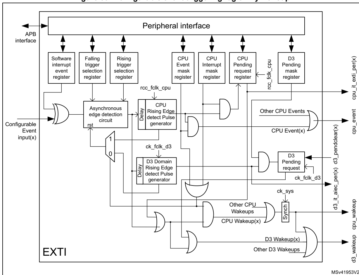
Figure 89. Configurable event triggering logic Any wakeup
