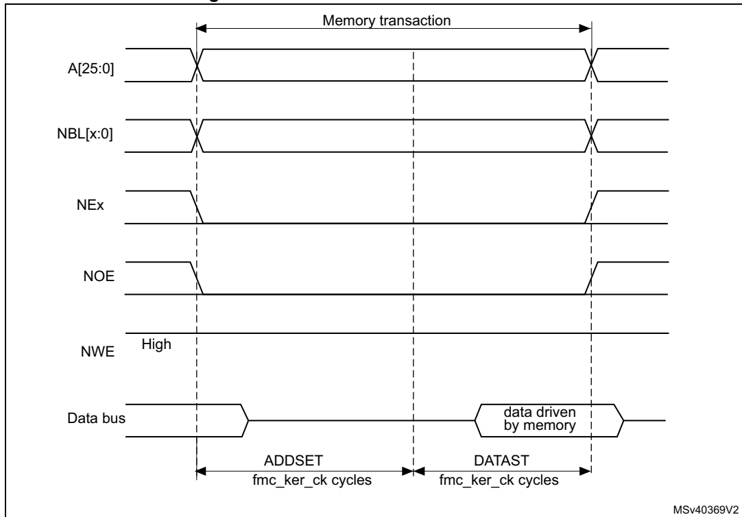
Figure 96. Mode 1 read access waveforms
