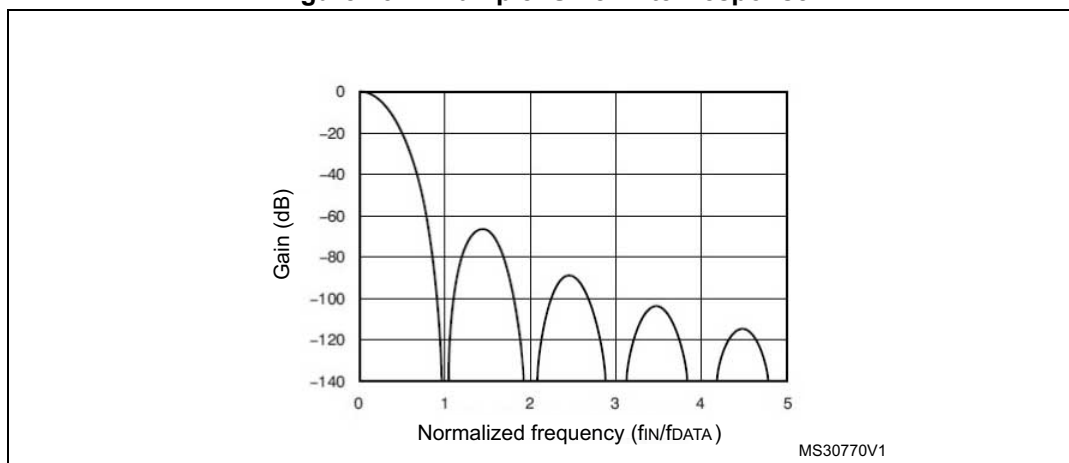
Figure 231. Example: Sinc 3 filter response
