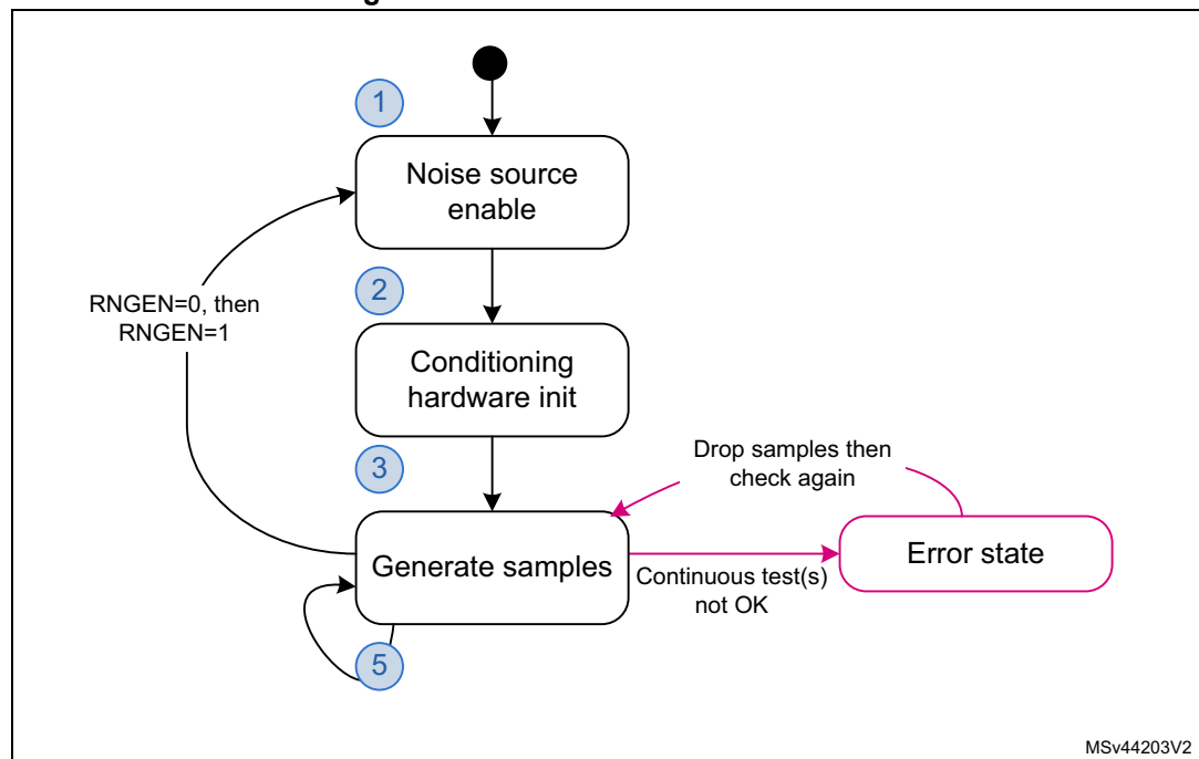
Figure 249. RNG initialization overview
