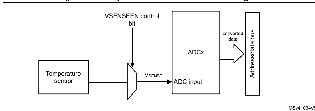
Figure 199. Temperature sensor channel block diagram
