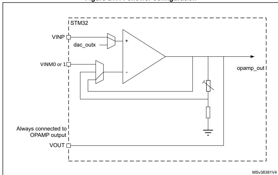
Figure 217. Follower configuration
