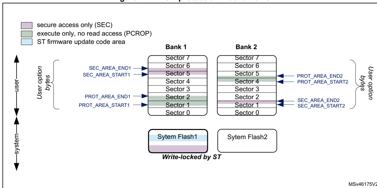
Figure 7. FLASH protection mechanisms
