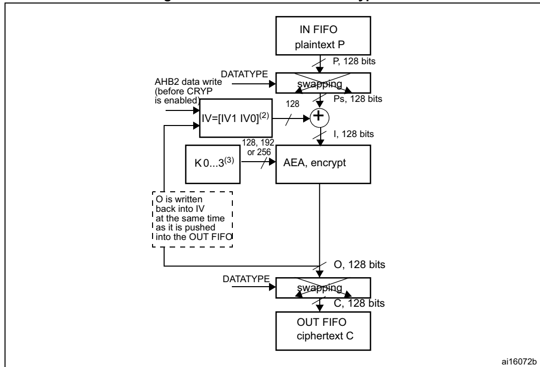
Figure 266. AES-CBC mode encryption
