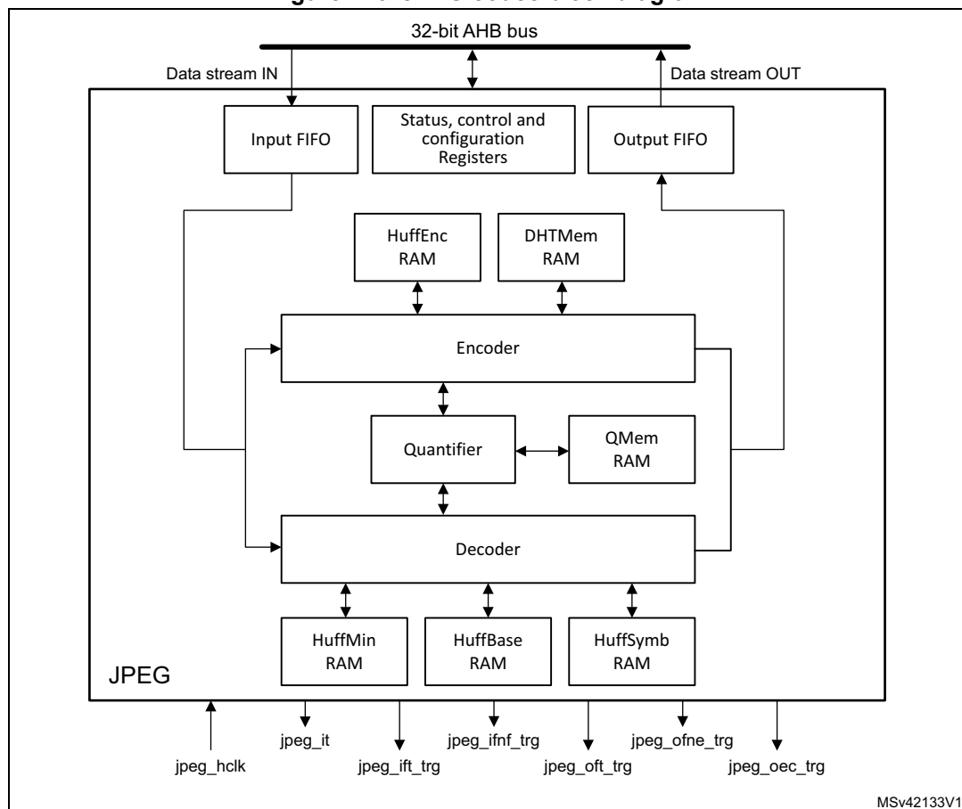
Figure 246. JPEG codec block diagram
