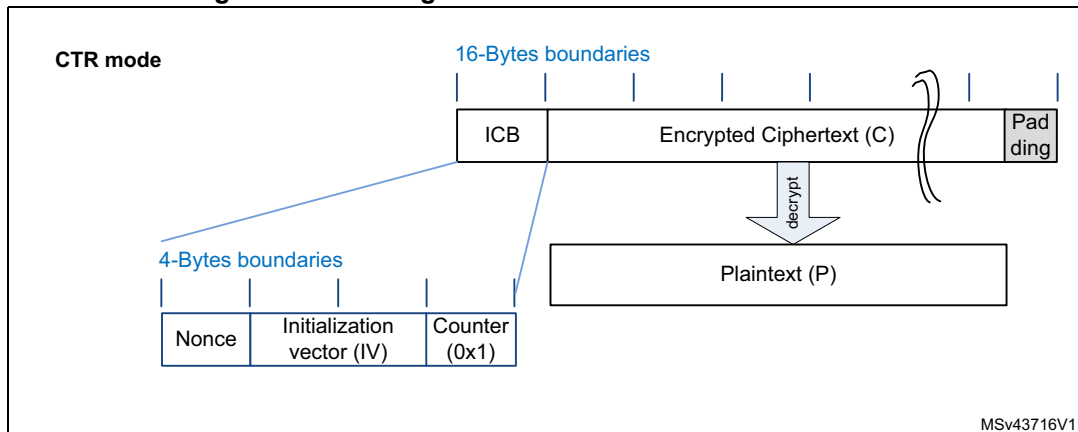
Figure 268. Message construction for the Counter mode
