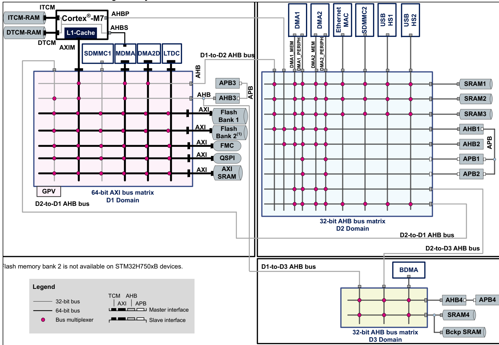
Figure 1. System architecture for STM32H742/743/53xx and STM32H750xB devices
