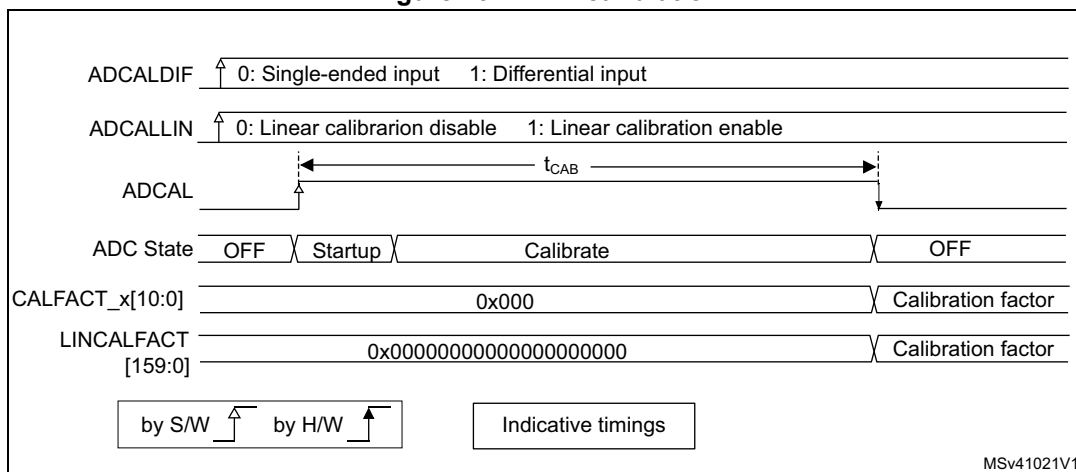
Figure 137. ADC calibration
