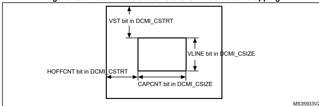
Figure 238. Coordinates and size of the window after cropping
