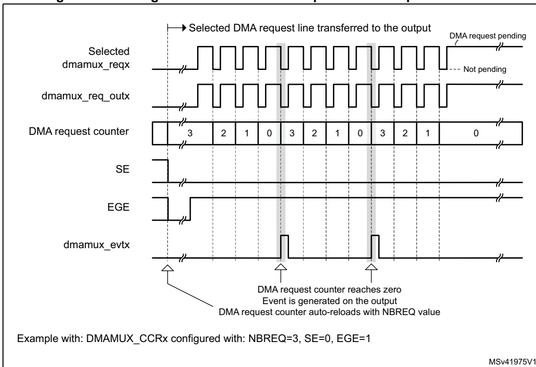
Figure 83. Event generation of the DMA request line multiplexer channel
