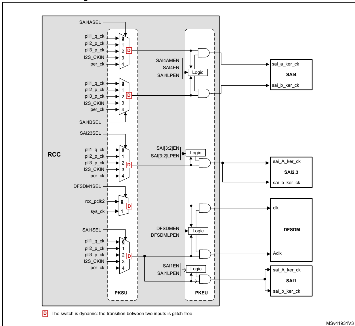
Figure 47. Kernel clock distribution for SAI4 and DFSDM
