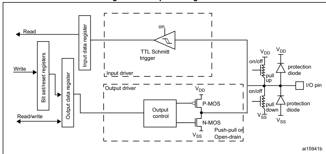
Figure 70. Output configuration
