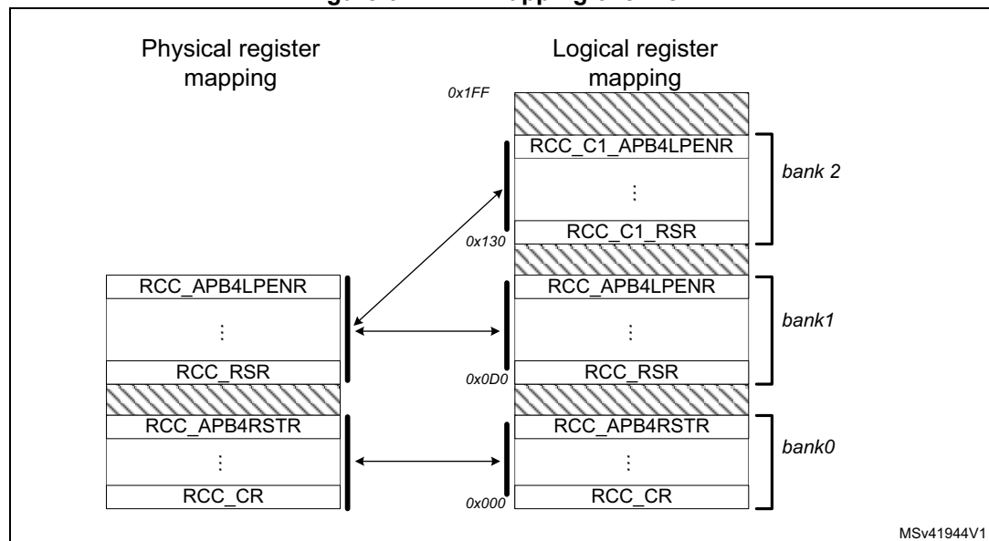
Figure 61. RCC mapping overview
