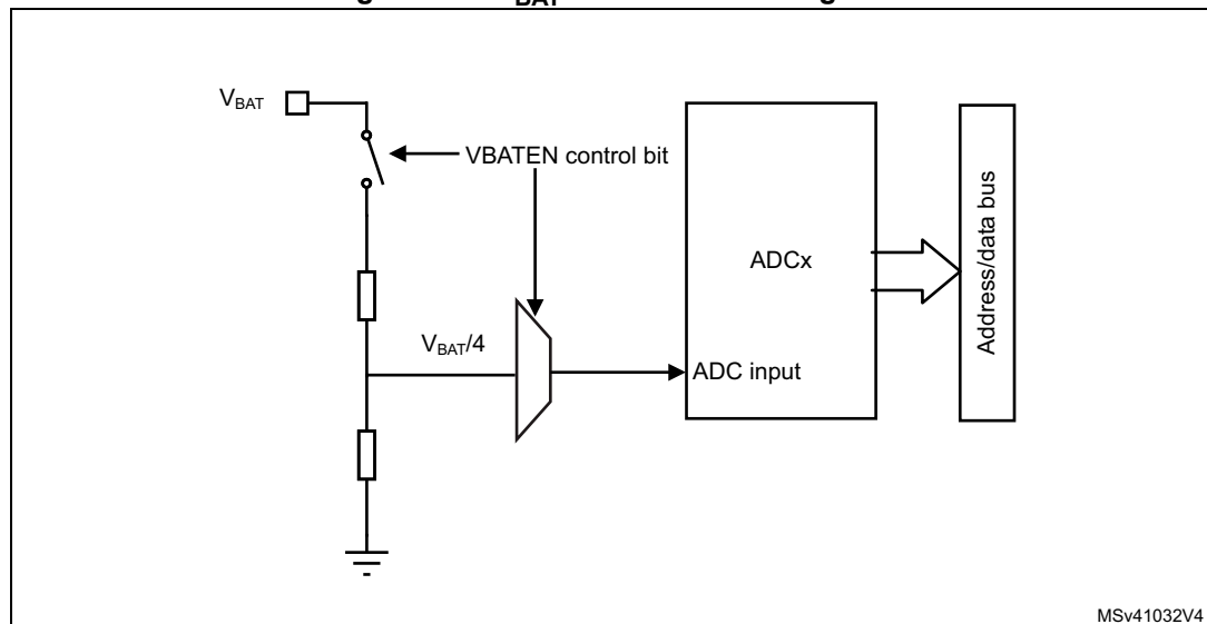
Figure 200. V_{BAT} channel block diagram
