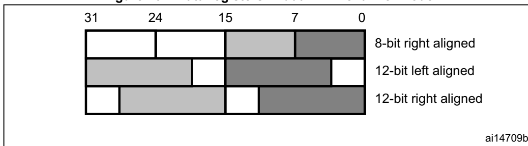
Figure 204. Data registers in dual DAC channel mode
