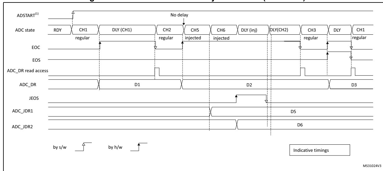
Figure 171. AUTDLY=1 in auto-injected mode (JAUTO=1)
