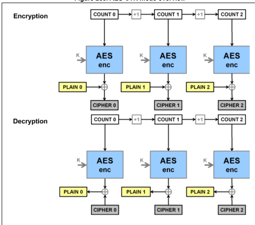
Figure 253. AES-CTR mode overview
