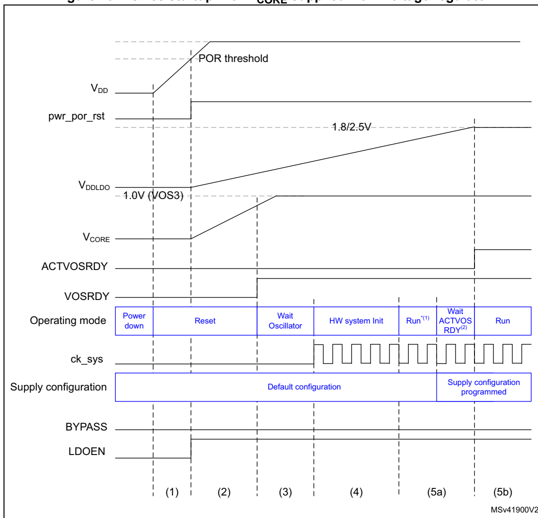
Figure 19. Device startup with V_{CORE} supplied from voltage regulator
