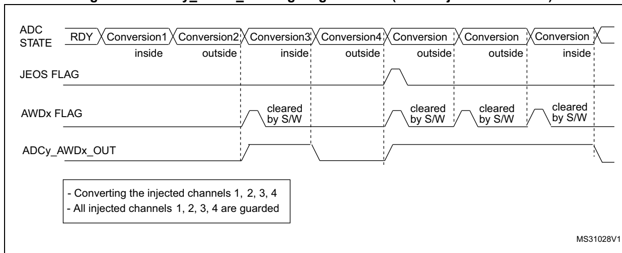
Figure 176. ADCy_AWDx_OUT signal generation (on all injected channels)
