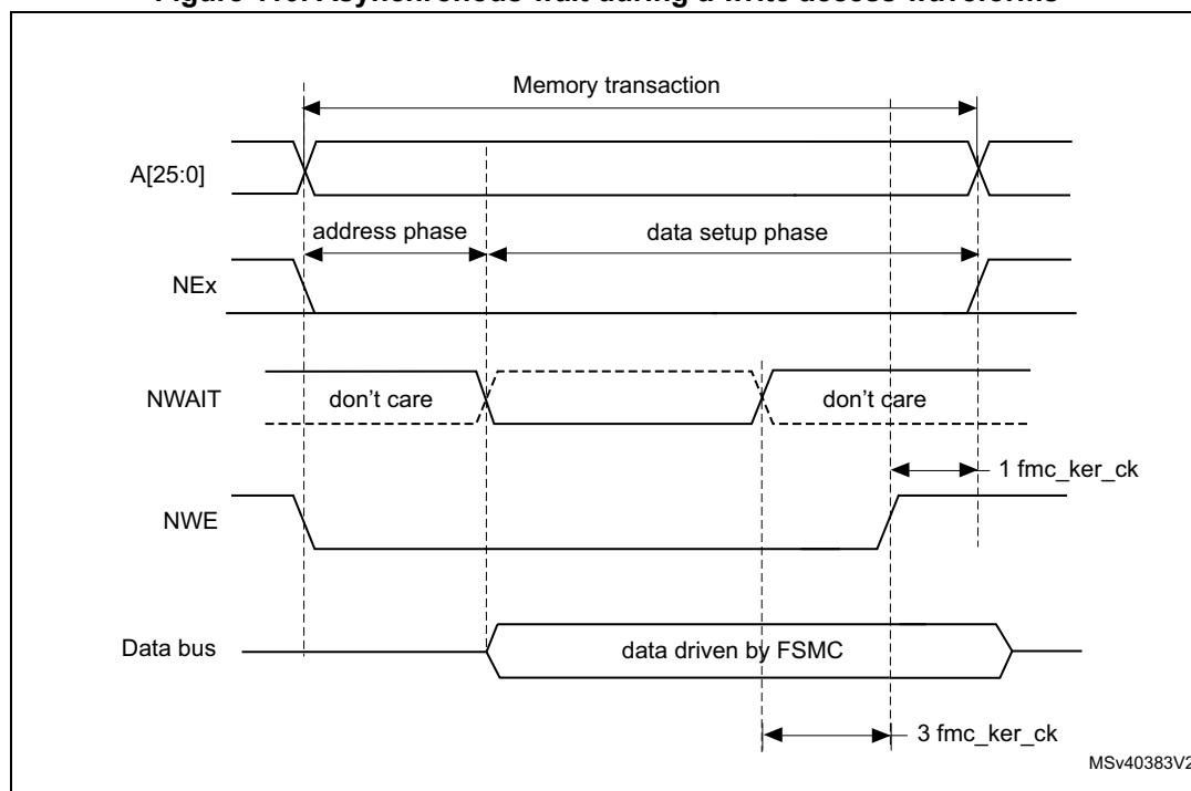
Figure 110. Asynchronous wait during a write access waveforms
