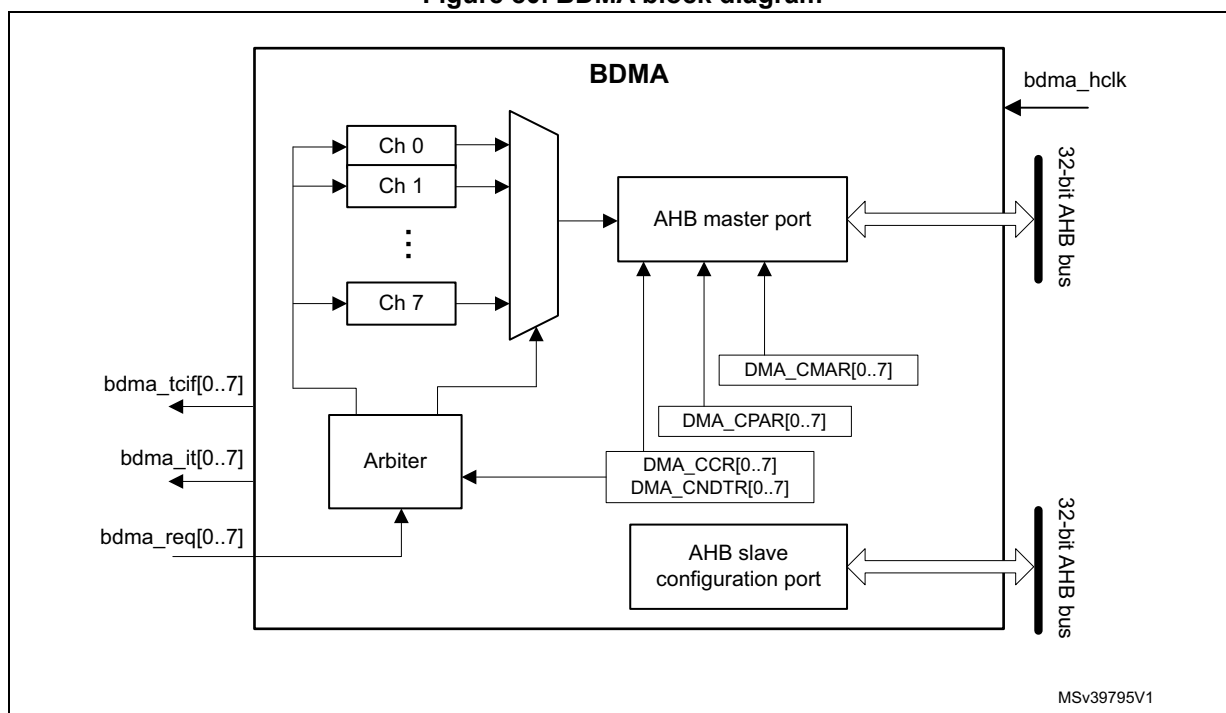
Figure 80. BDMA block diagram
