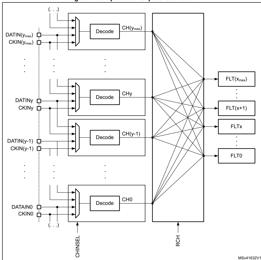
Figure 225. Input channel pins redirection
