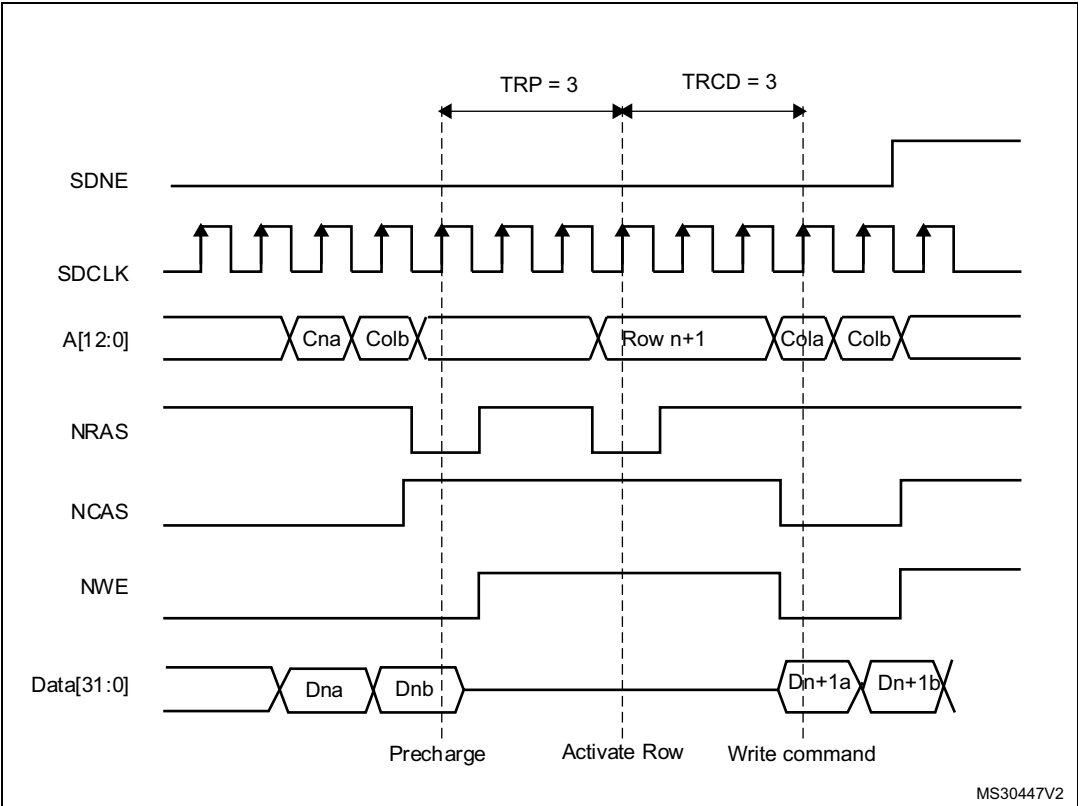
Figure 120. Write access crossing row boundary
