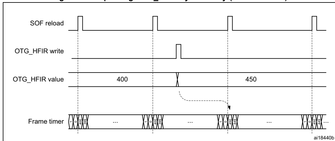
Figure 750. Updating OTG_HFIR dynamically (RLDCTRL = 0)
