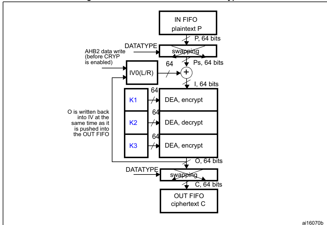
Figure 262. DES/TDES-CBC mode encryption
