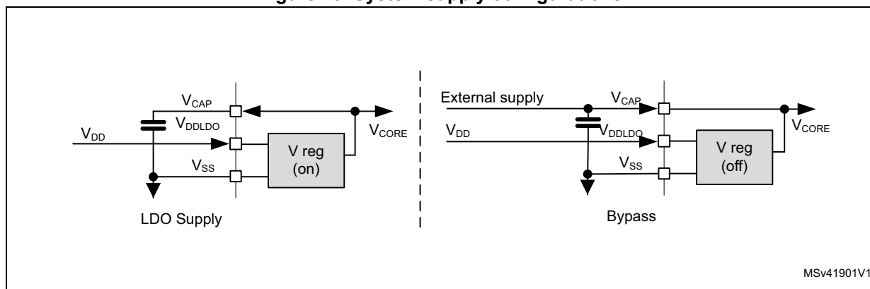
Figure 18. System supply configurations
