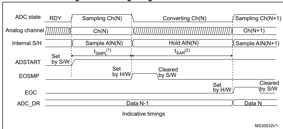
Figure 141. Analog to digital conversion time
