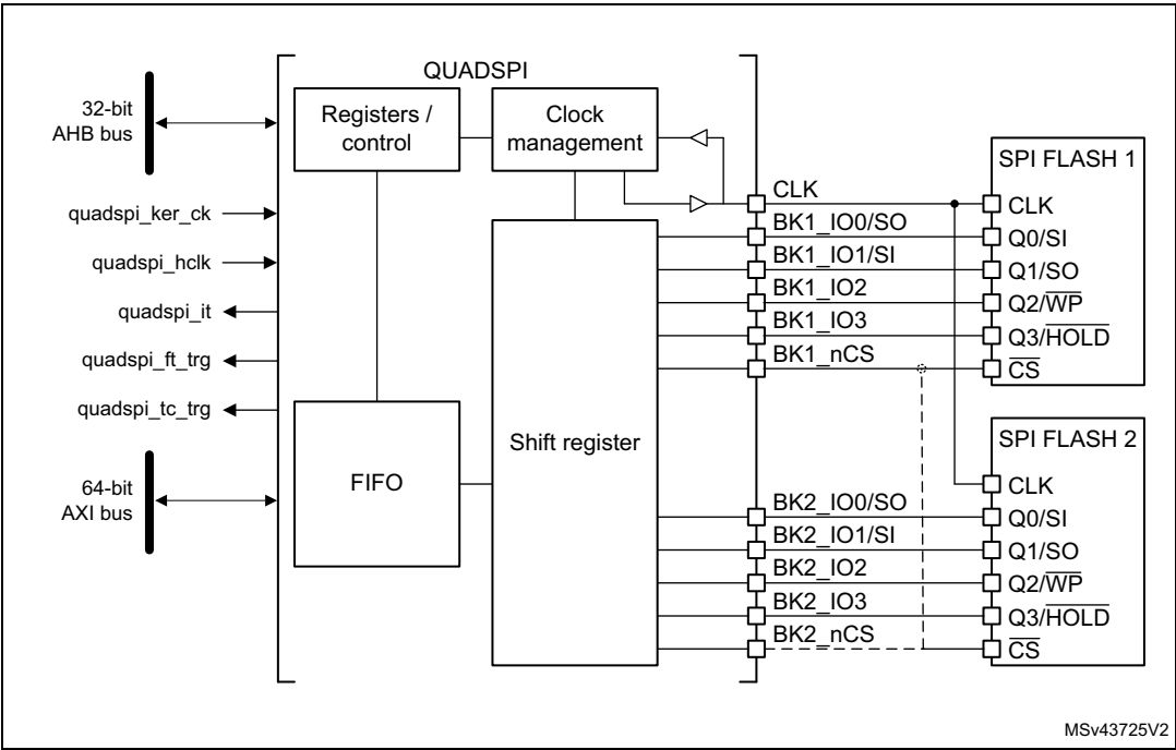
Figure 124. QUADSPI block diagram when dual-flash mode is enabled
