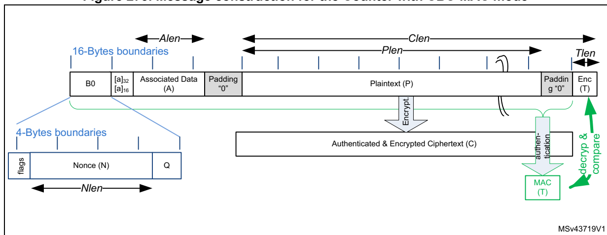
Figure 273. Message construction for the Counter with CBC-MAC mode
