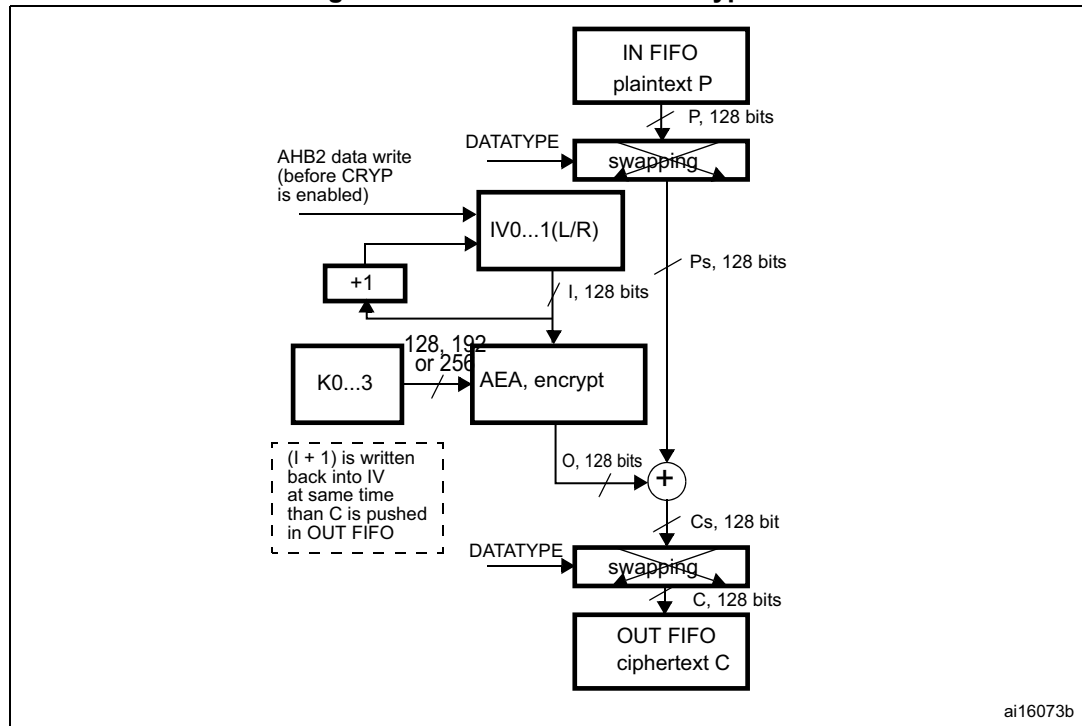
Figure 269. AES-CTR mode encryption
