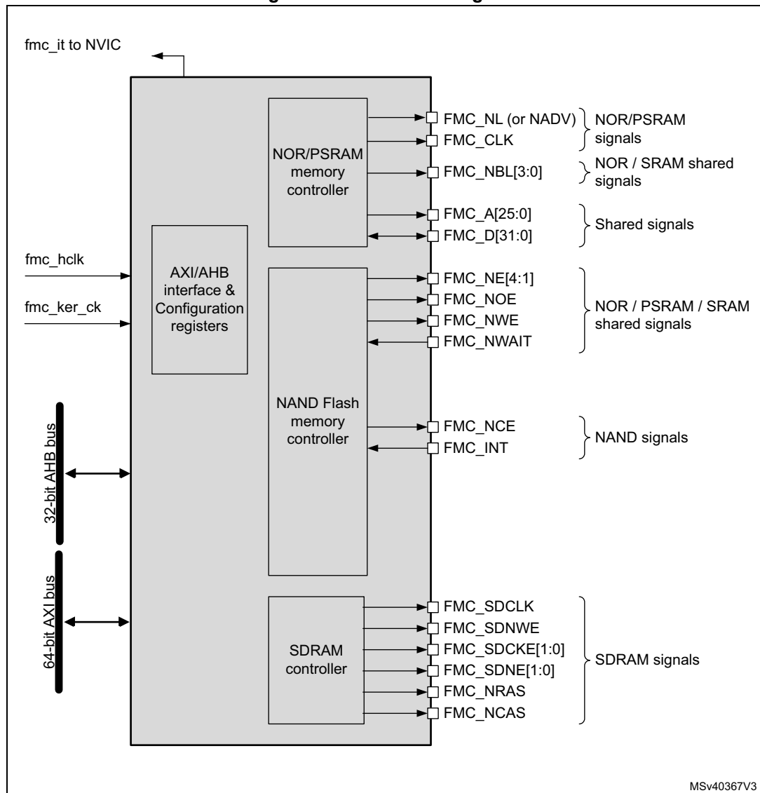
Figure 94. FMC block diagram
