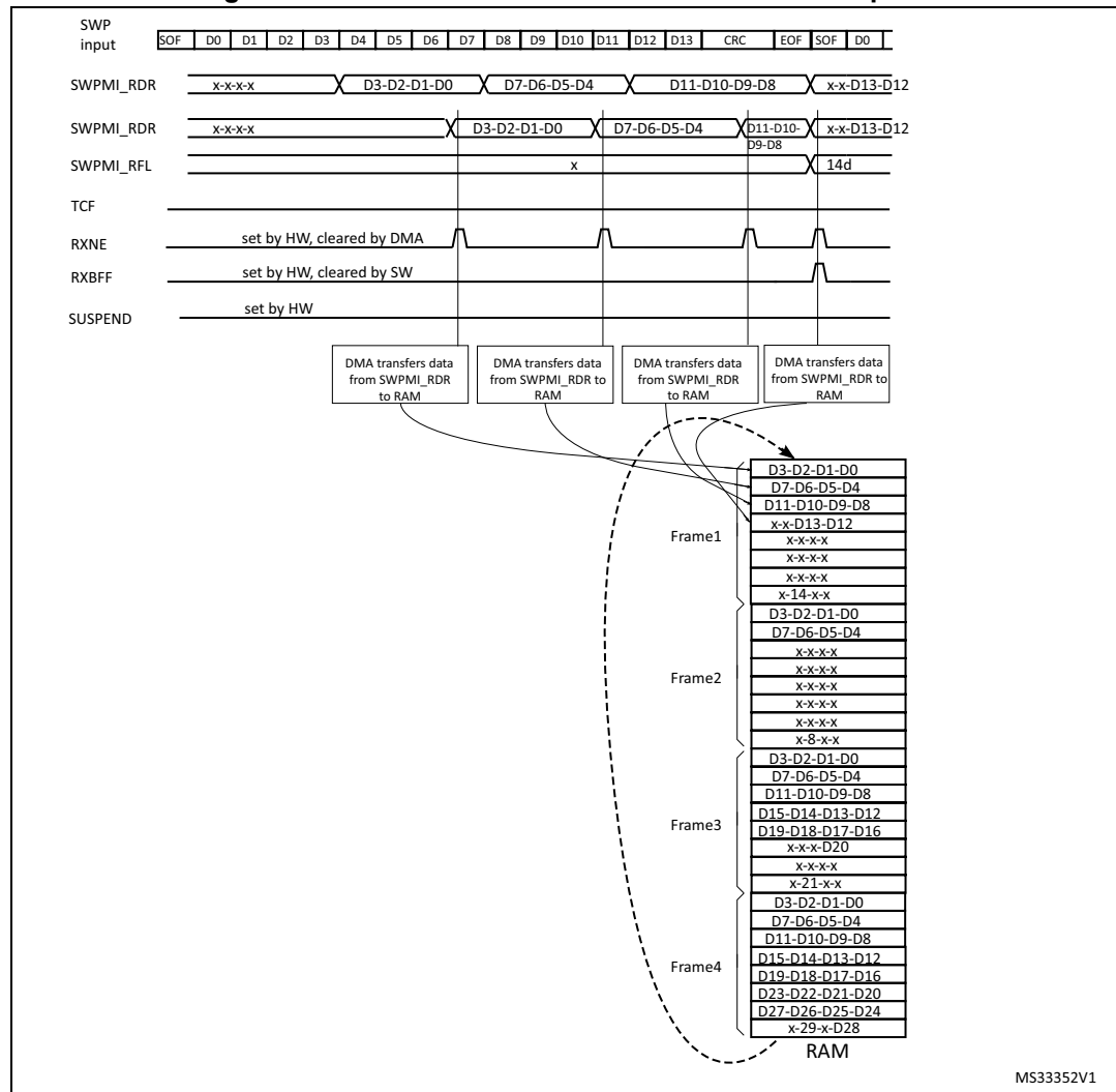
Figure 691. SWPMI Multi software buffer mode reception
