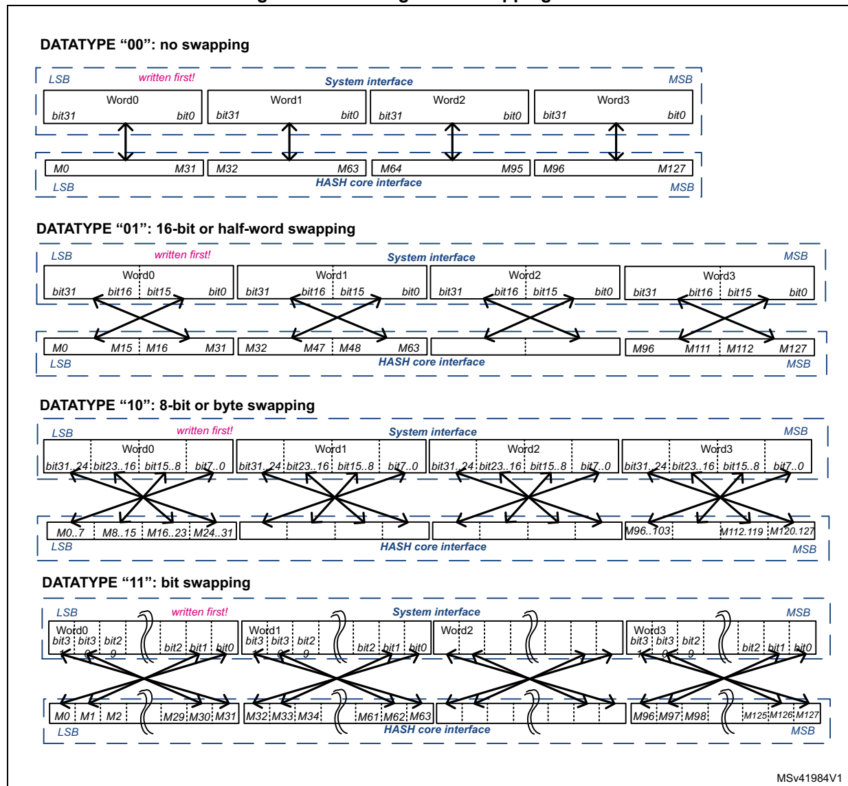
Figure 278. Message data swapping feature
