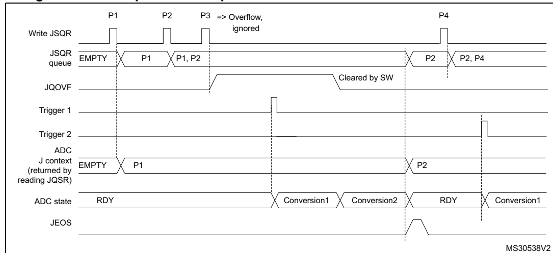
Figure 148. Example of JSQR queue of context with overflow before conversion
