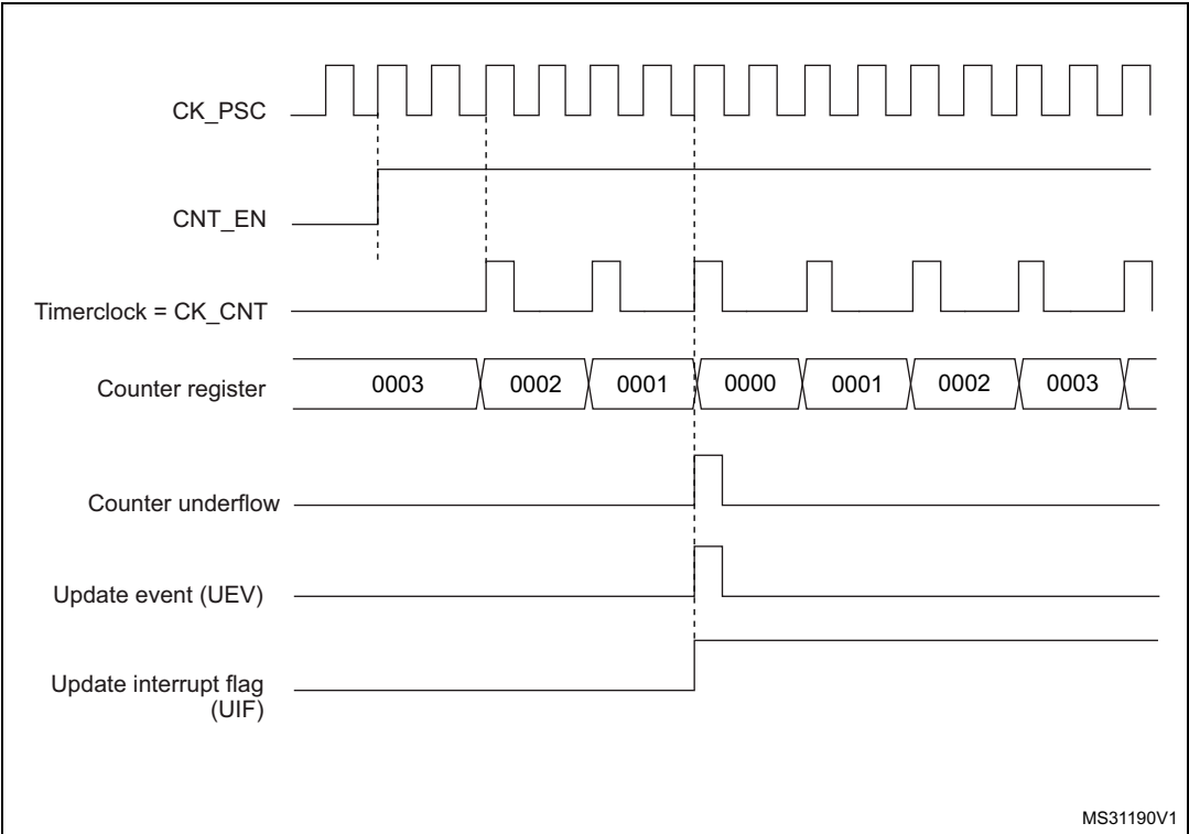
Figure 419. Counter timing diagram, internal clock divided by 2
