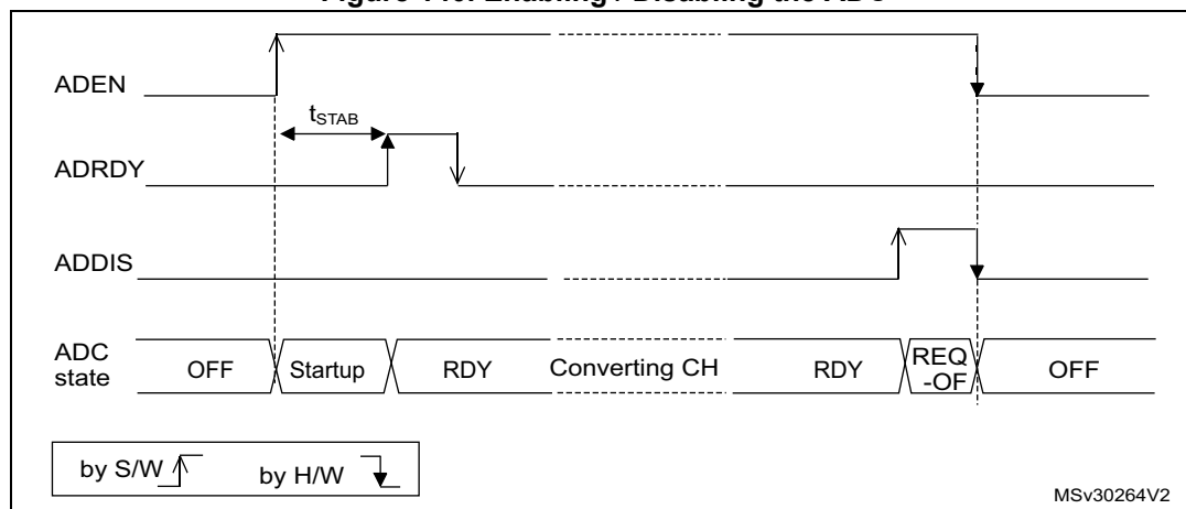
Figure 140. Enabling / Disabling the ADC
