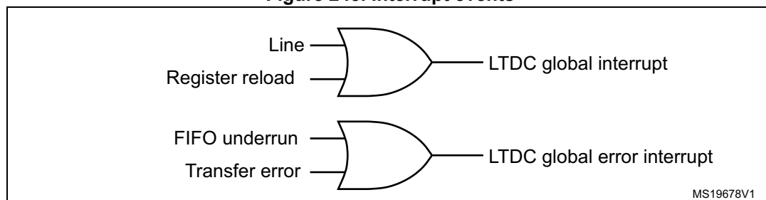
Figure 245. Interrupt events
