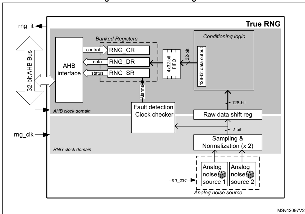
Figure 247. RNG block diagram
