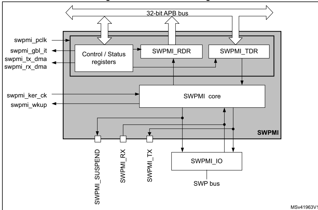
Figure 683. SWPMI block diagram
