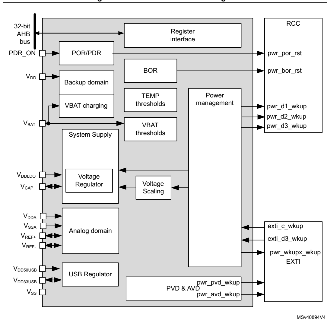
Figure 16. Power control block diagram
