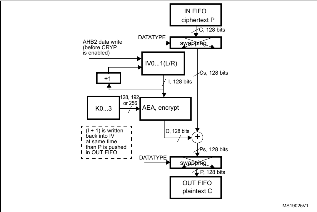
Figure 270. AES-CTR mode decryption
