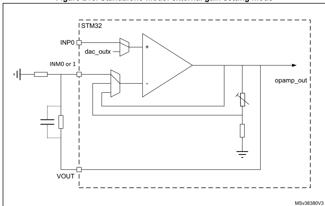
Figure 216. Standalone mode: external gain setting mode
