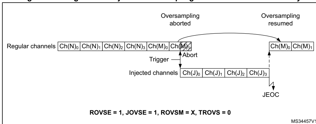
Figure 180. Regular and injected oversampling modes used simultaneously
