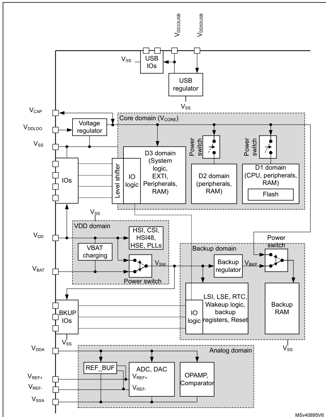
Figure 17. Power supply overview
