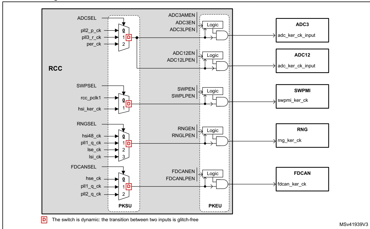
Figure 55. Kernel clock distribution for ADCs, SWPMI, RNG and FDCAN (2)
