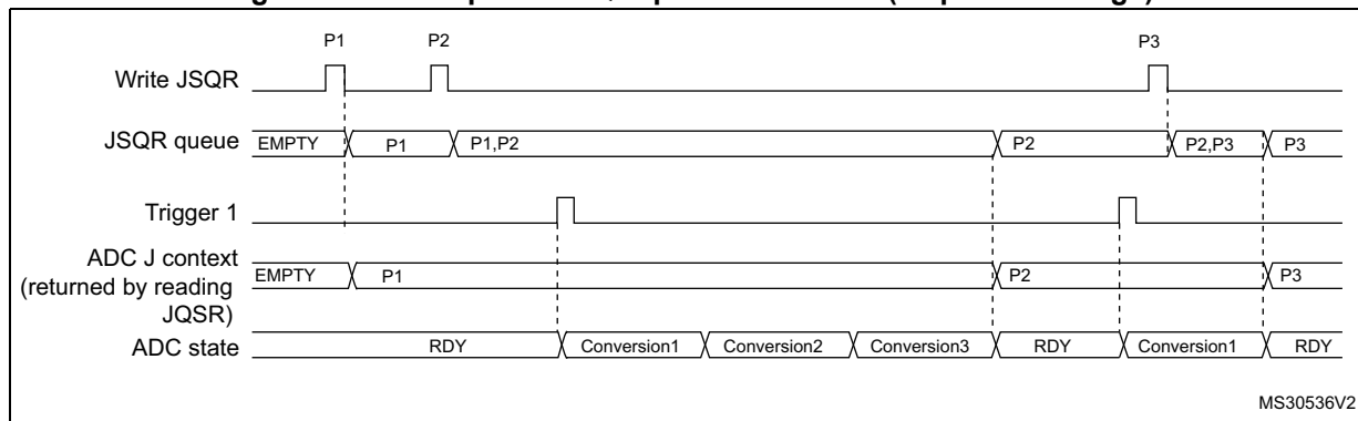
Figure 146. Example of JSQR queue of context (sequence change)
