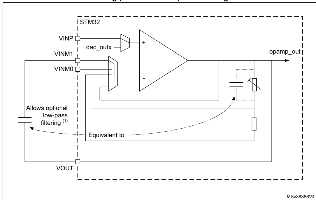
Figure 222. PGA mode, non-inverting gain setting (x2/x4/x8/x16) or inverting gain setting (x-1/x-3/x-7/x-15) with filtering
