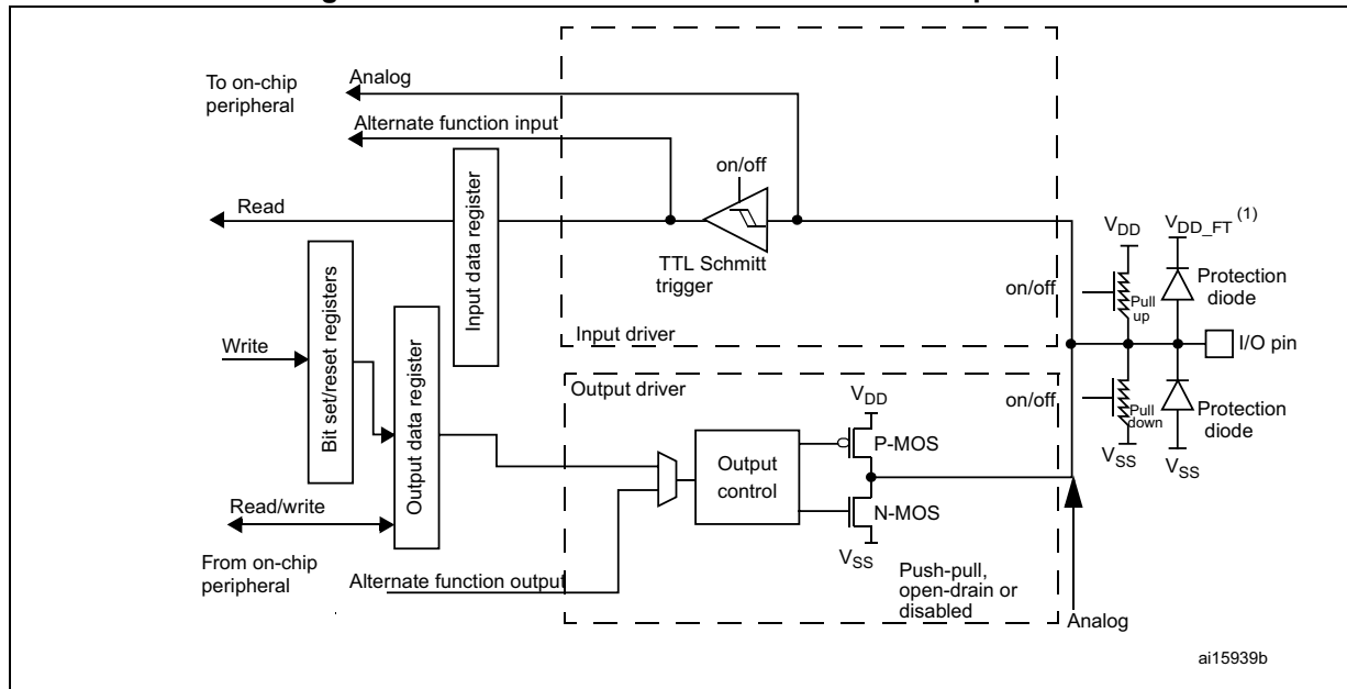
Figure 68. Basic structure of a 5-Volt tolerant I/O port bit
