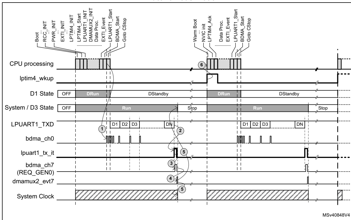
Figure 38. Timing diagram of LPUART1 transmission with D3 domain in Autonomous mode
