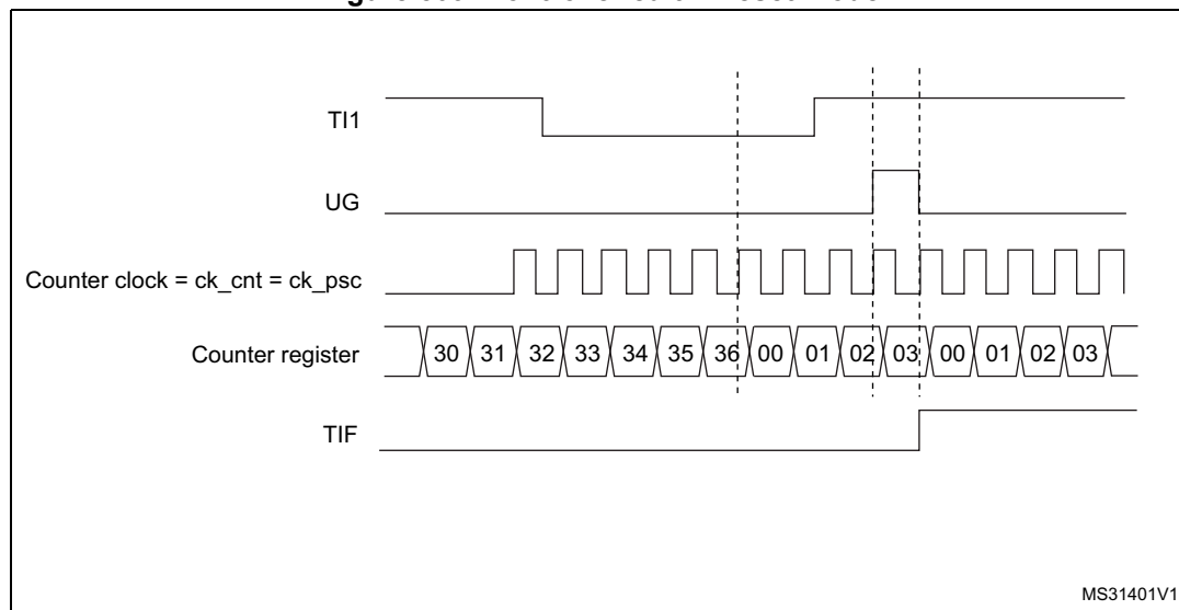
Figure 509. Control circuit in reset mode
