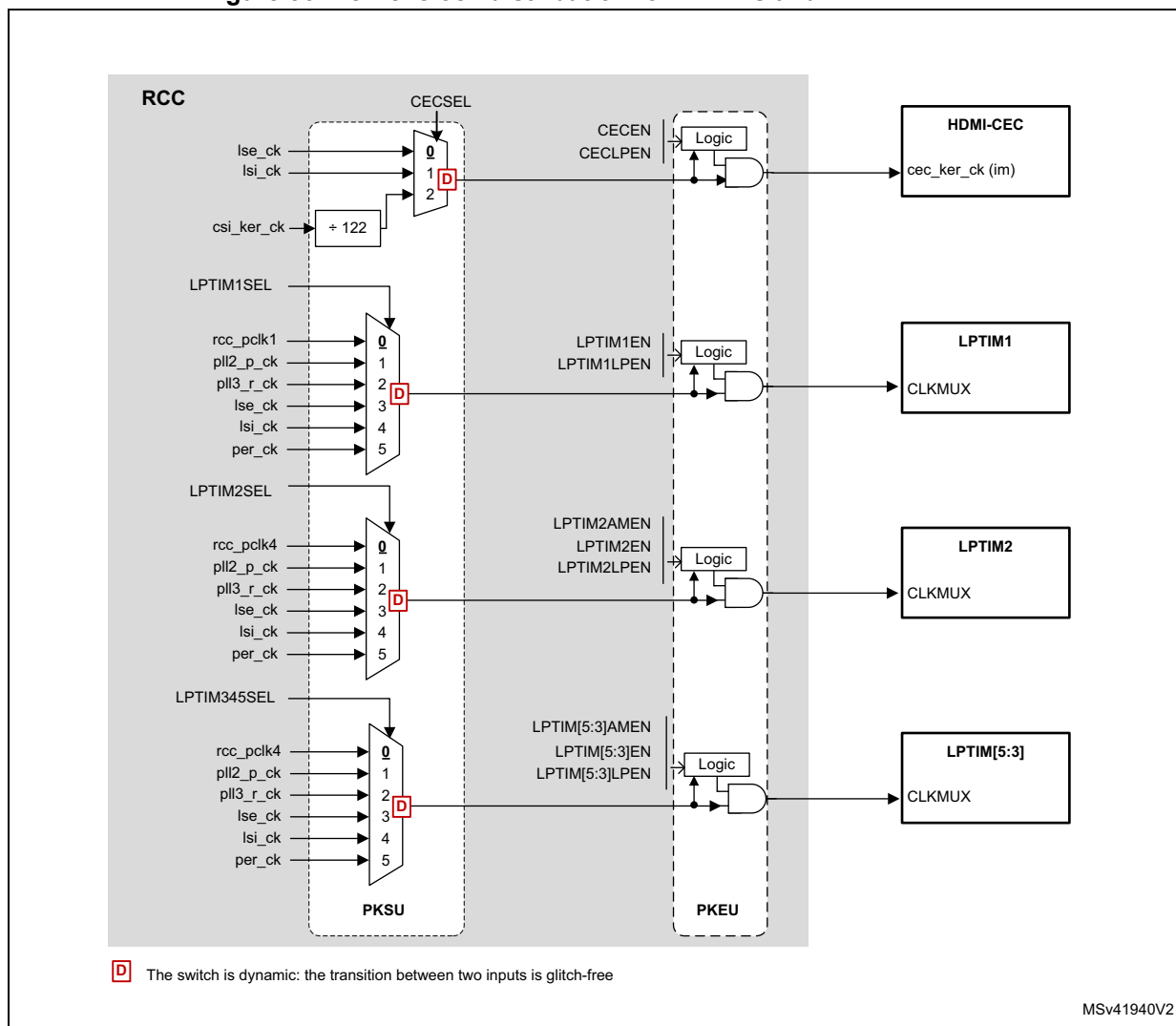
Figure 56. Kernel clock distribution for LPTIMs and HDMI-CEC (2)
