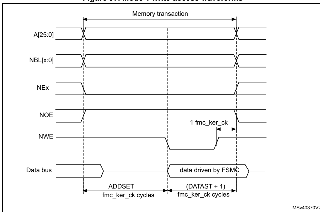
Figure 97. Mode 1 write access waveforms
