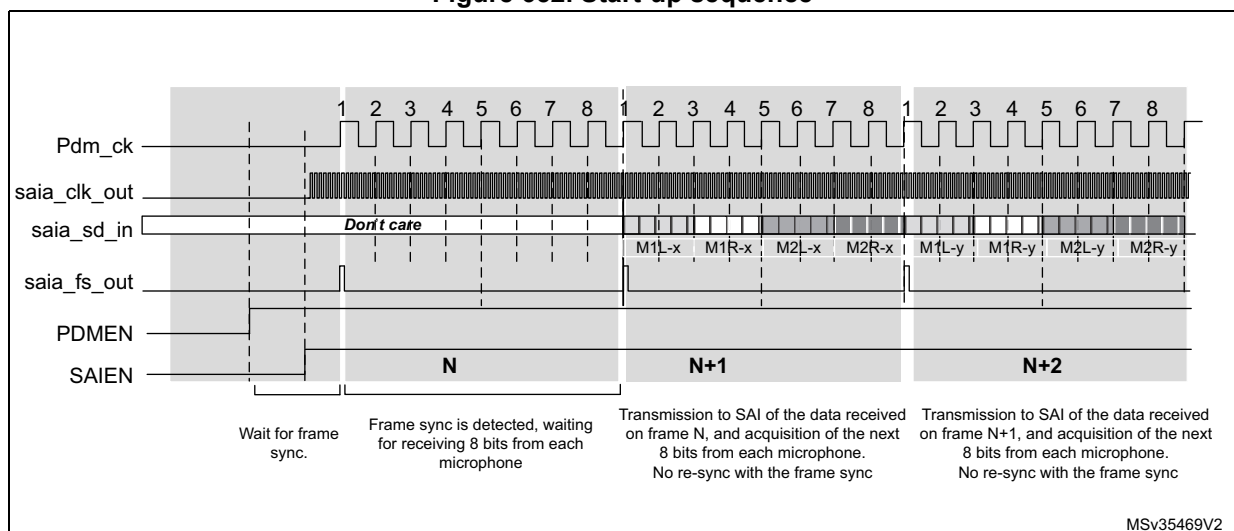
Figure 652. Start-up sequence
