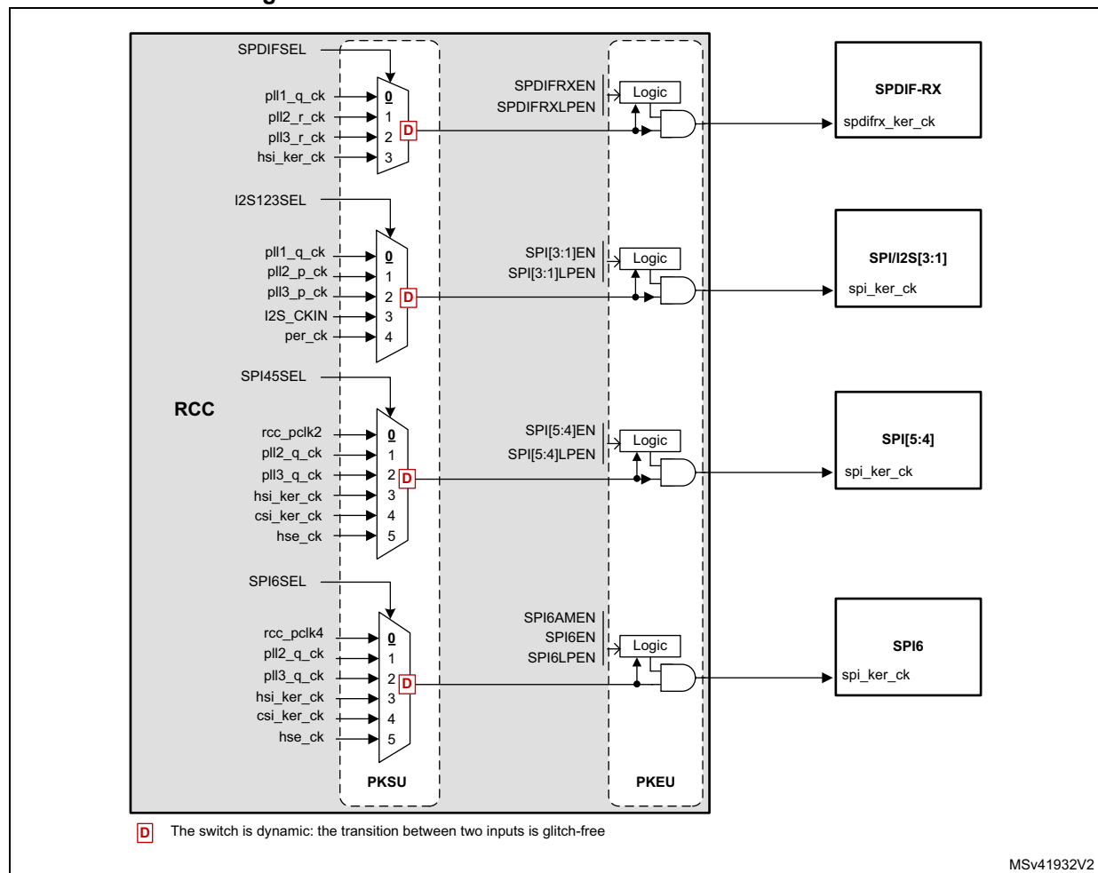
Figure 48. Kernel clock distribution for SPIs and SPI/I2S
