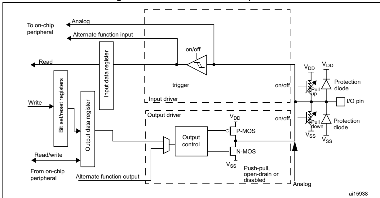
Figure 67. Basic structure of an I/O port bit
