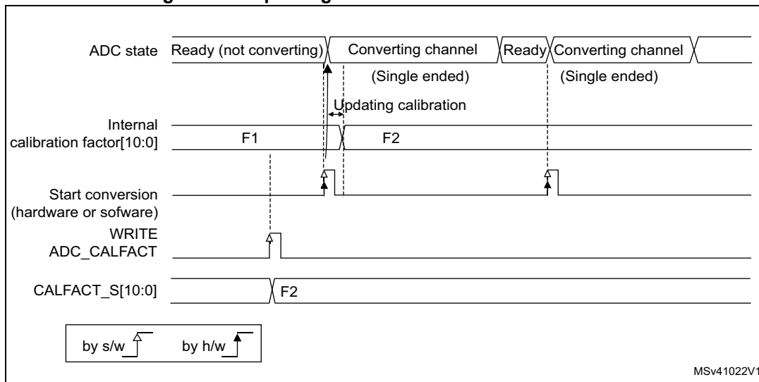
Figure 138. Updating the ADC offset calibration factor
