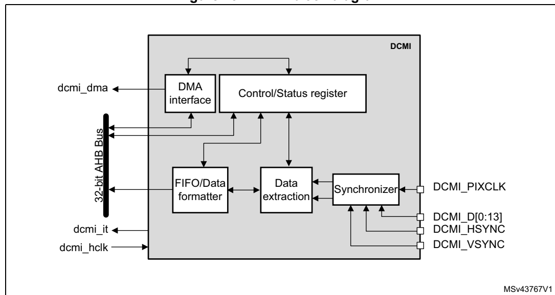
Figure 233. Top-level block diagram
