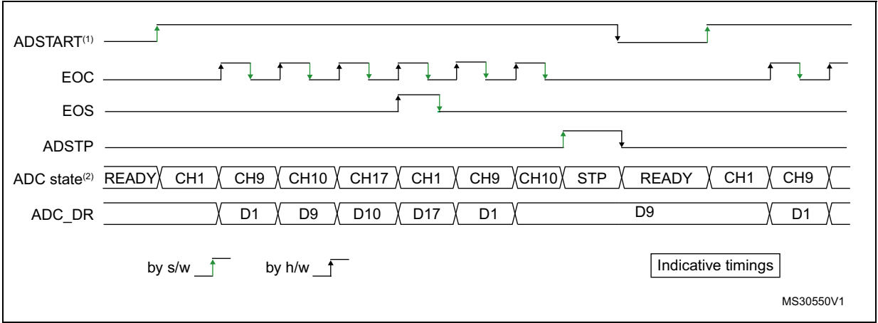
Figure 159. Continuous conversion of a sequence, software trigger
