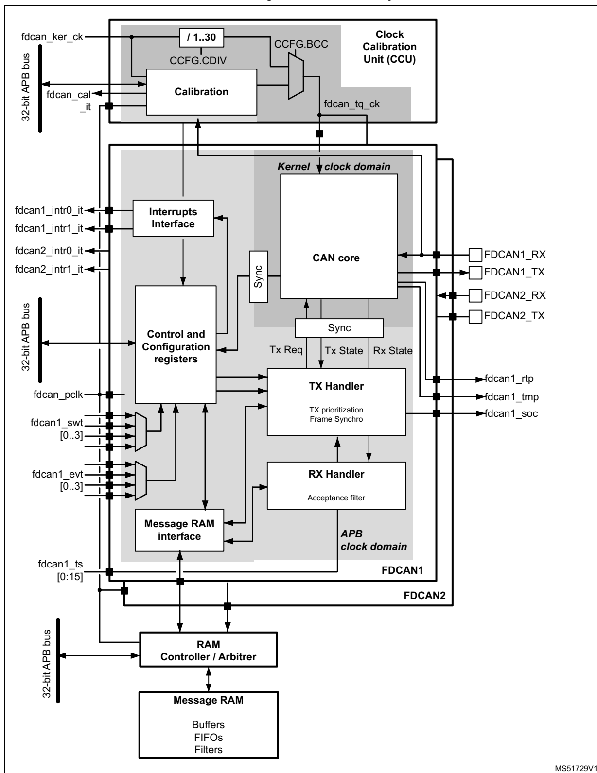
Figure 730. CAN subsystem
