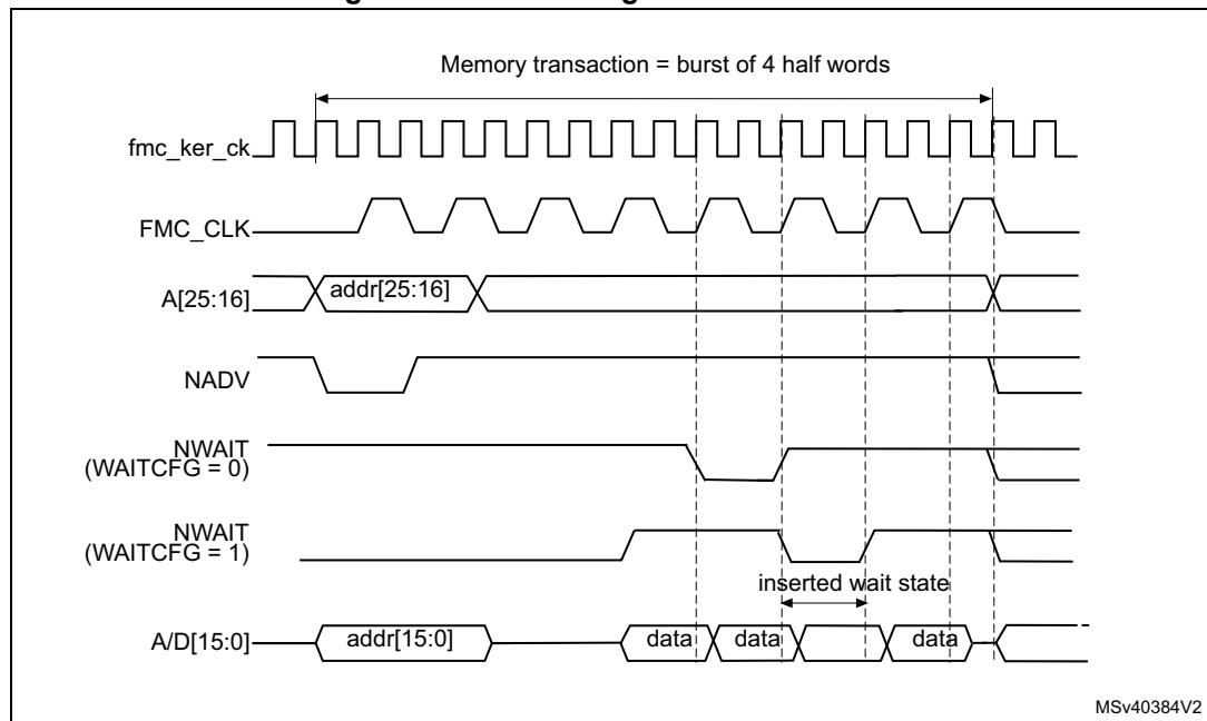
Figure 112. Synchronous multiplexed read mode waveforms - NOR, PSRAM (CRAM)
