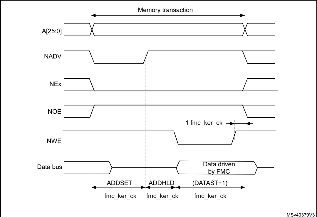
Figure 106. Mode D write access waveforms
