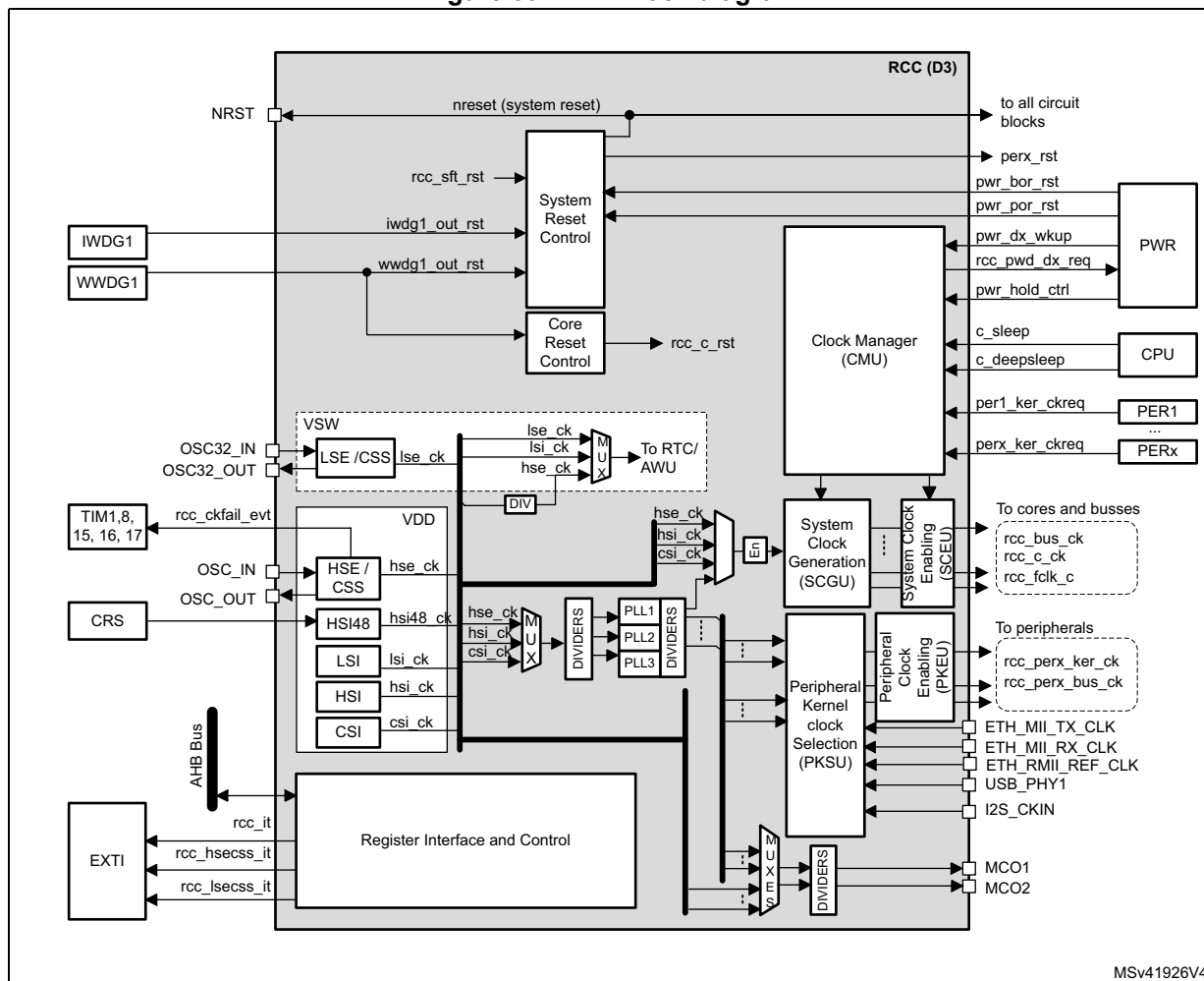
Figure 39. RCC Block diagram
