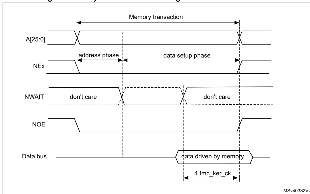
Figure 109. Asynchronous wait during a read access waveforms
