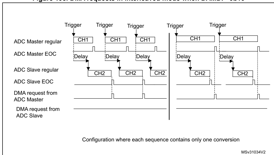
Figure 198. DMA requests in interleaved mode when DAMDF=0b10
