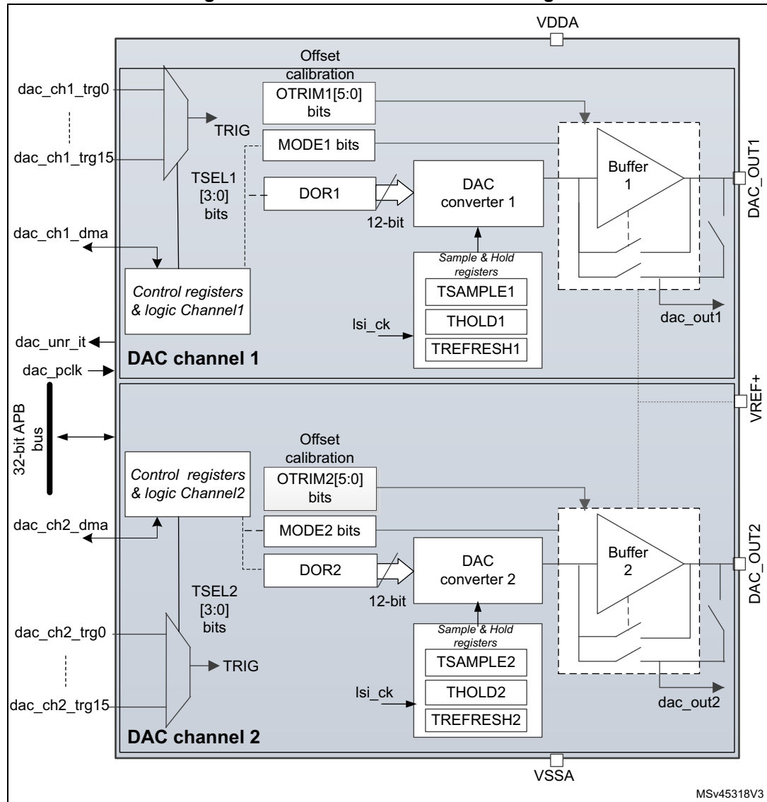
Figure 202. Dual-channel DAC block diagram
