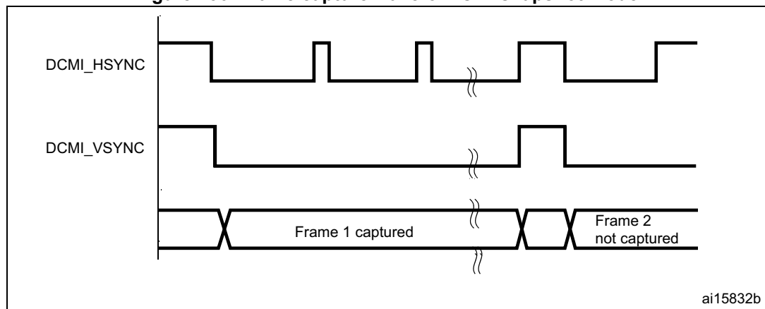
Figure 236. Frame capture waveforms in snapshot mode
