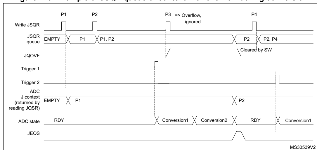
Figure 149. Example of JSQR queue of context with overflow during conversion
