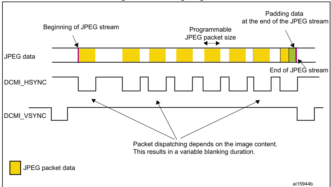
Figure 235. Timing diagram
