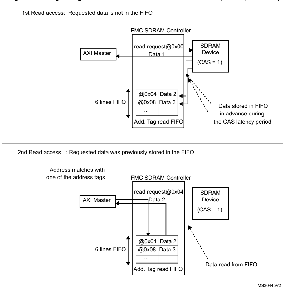
Figure 118. Logic diagram of Read access with RBURST bit set (CAS=2, RPIPE=0)
