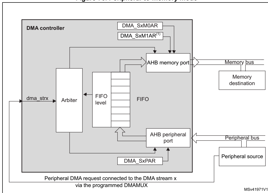
Figure 76. Peripheral-to-memory mode
