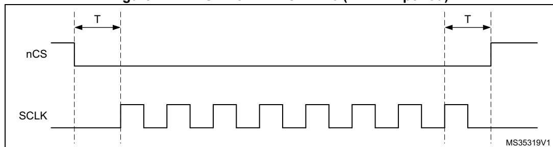
Figure 127. nCS when CKMODE = 0 (T = CLK period)
