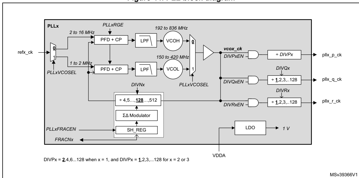
Figure 44. PLL block diagram
