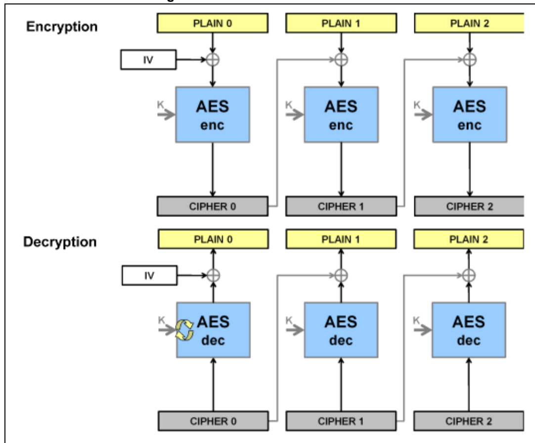
Figure 252. AES-CBC mode overview
