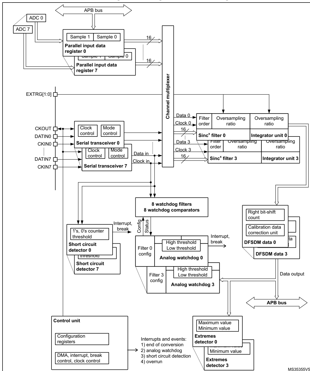
Figure 224. Single DFSDM block diagram
