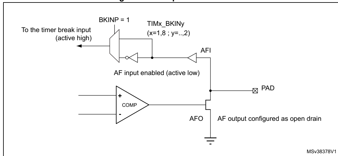
Figure 214. Output redirection
