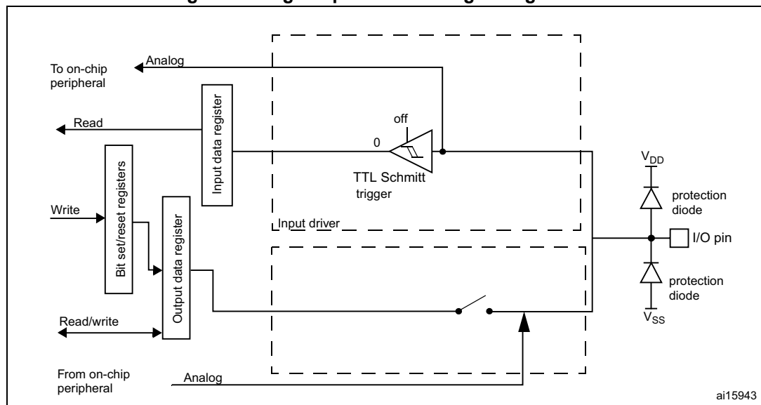
Figure 72. High impedance-analog configuration
