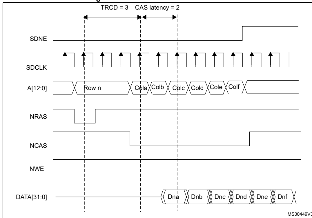
Figure 117. Burst read SDRAM access
