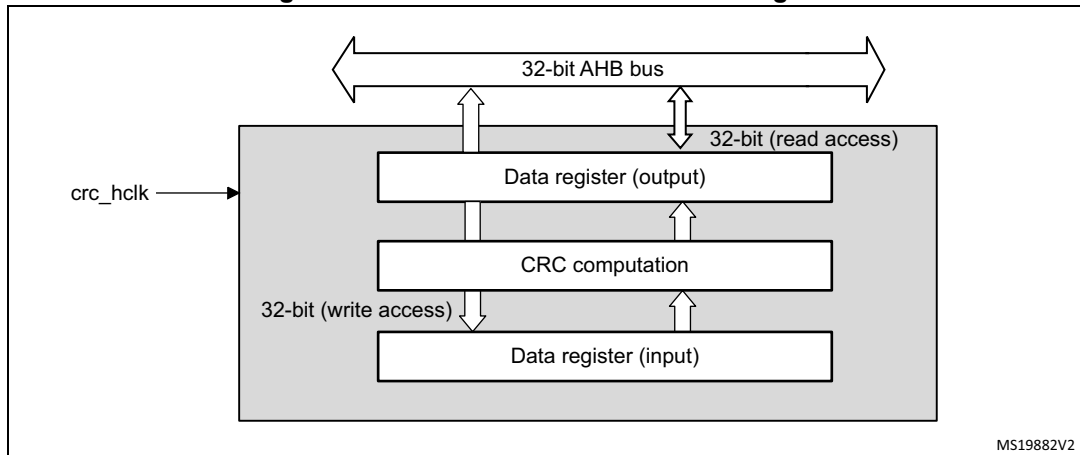
Figure 93. CRC calculation unit block diagram
