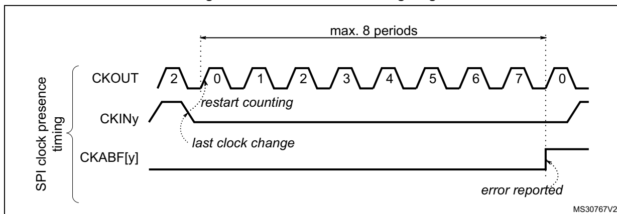
Figure 227. Clock absence timing diagram for SPI
