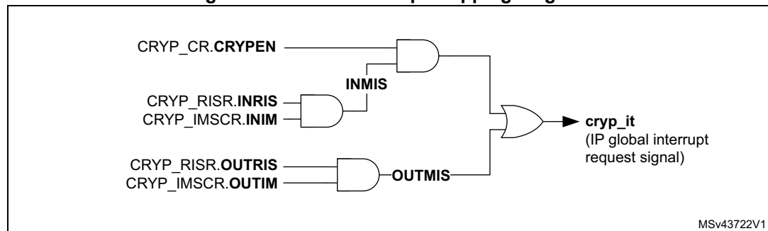
Figure 276. CRYP interrupt mapping diagram
