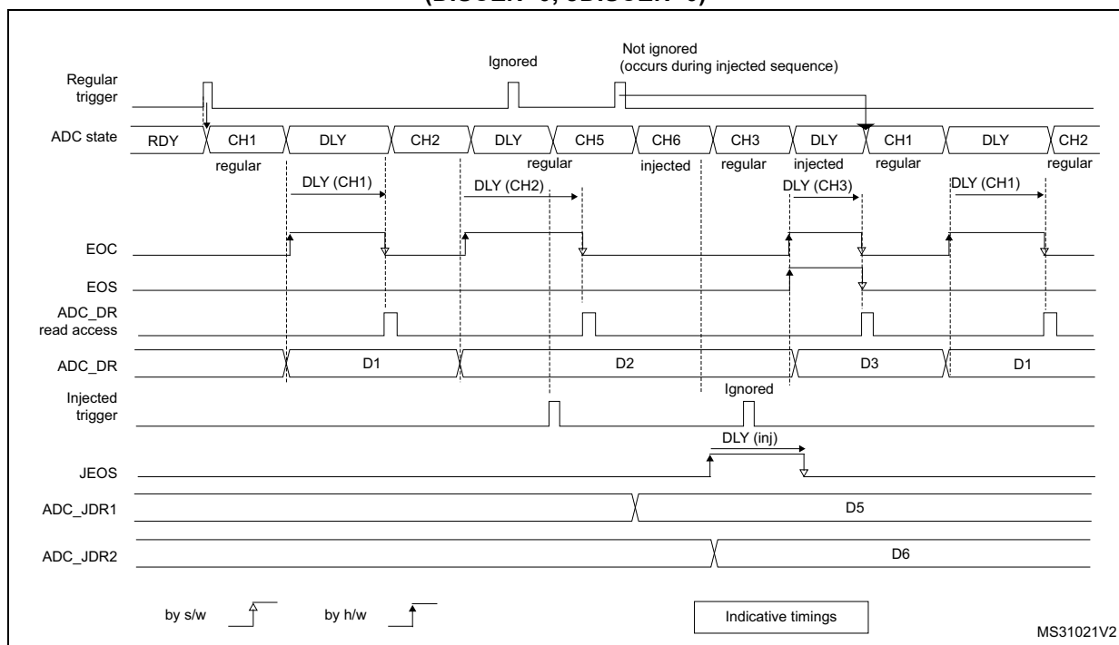
Figure 168. AUTDLY=1, regular HW conversions interrupted by injected conversions (DISCEN=0; JDISCEN=0)
