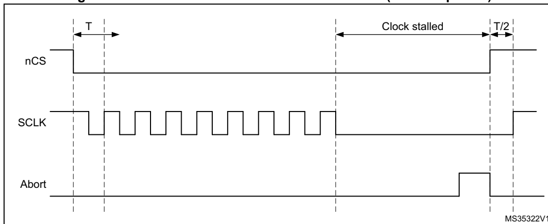
Figure 130. nCS when CKMODE = 1 with an abort ( T = \text{CLK period} )
