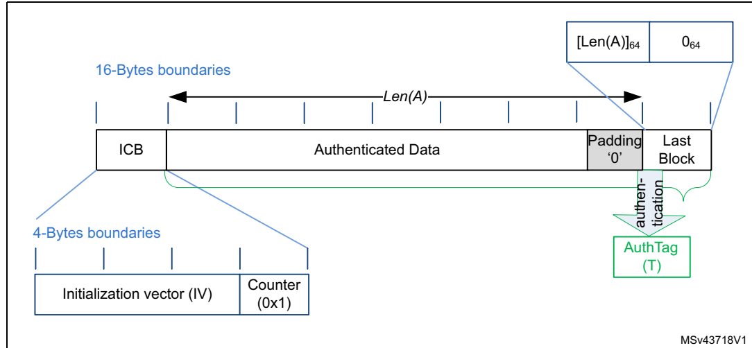
Figure 272. Message construction for the Galois Message Authentication Code mode
