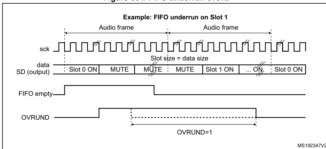
Figure 664. FIFO underrun event
