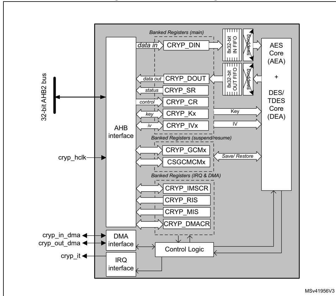
Figure 250. CRYP block diagram
