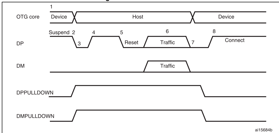
Figure 775. B-device HNP
