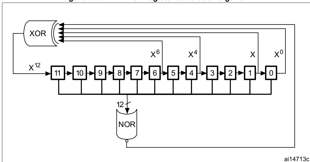
Figure 206. DAC LFSR register calculation algorithm
