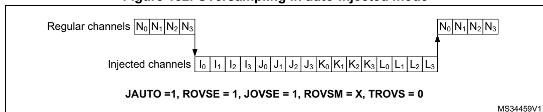
Figure 182. Oversampling in auto-injected mode
