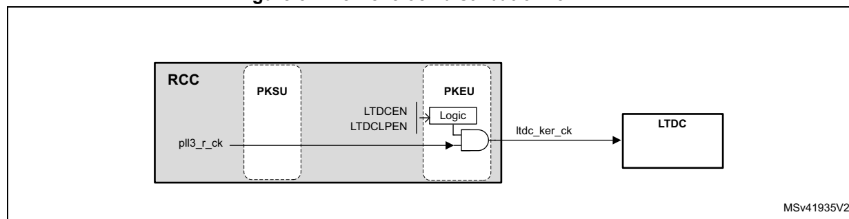
Figure 51. Kernel clock distribution for LTDC
