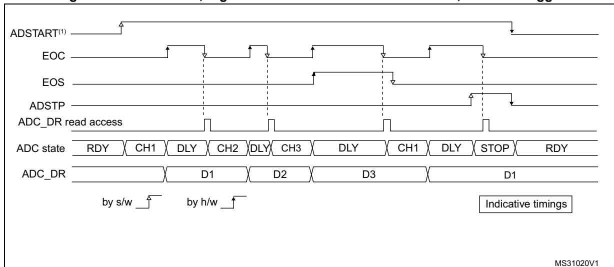
Figure 167. AUTDLY=1, regular conversion in continuous mode, software trigger
