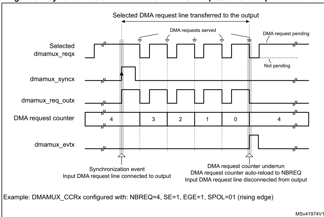
Figure 82. Synchronization mode of the DMAMUX request line multiplexer channel
