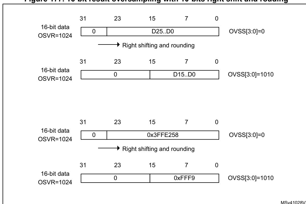
Figure 177. 16-bit result oversampling with 10-bits right shift and rounding
