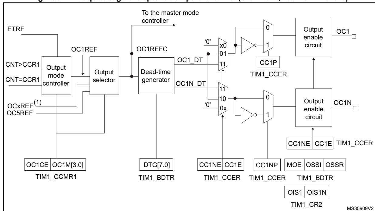
Figure 374. Output stage of capture/compare channel (channel 1, idem ch. 2 and 3)
