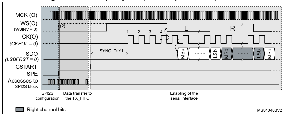
Figure 634. Start-up sequence, I2S Philips standard, master
