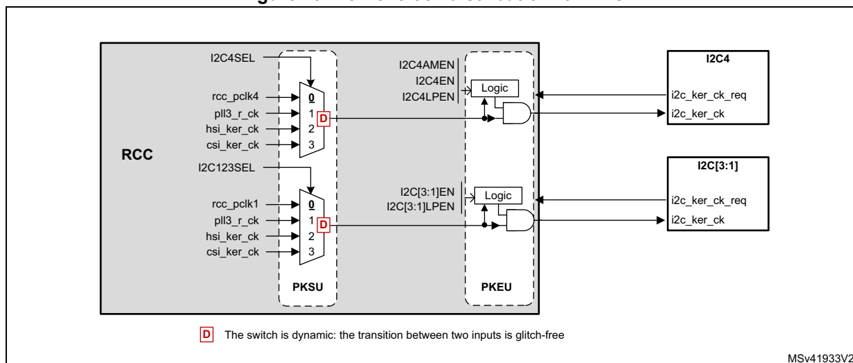
Figure 49. Kernel clock distribution for I2Cs
