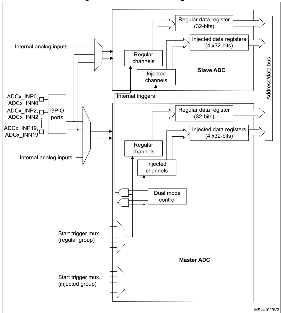
Figure 183. Dual ADC block diagram (1)
