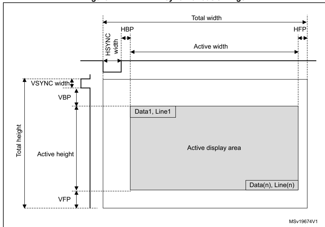
Figure 242. LCD-TFT synchronous timings
