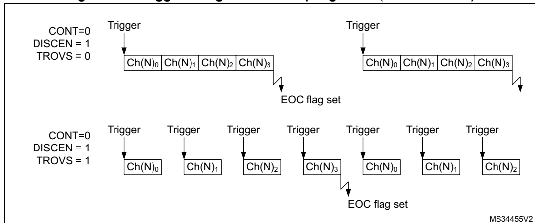
Figure 178. Triggered regular oversampling mode (TROVS bit = 1)
