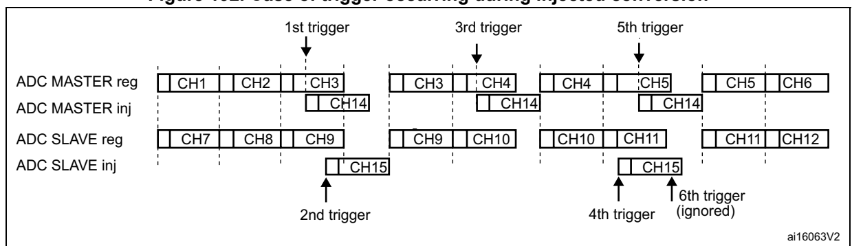
Figure 192. Case of trigger occurring during injected conversion
