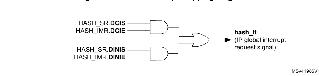
Figure 280. HASH interrupt mapping diagram
