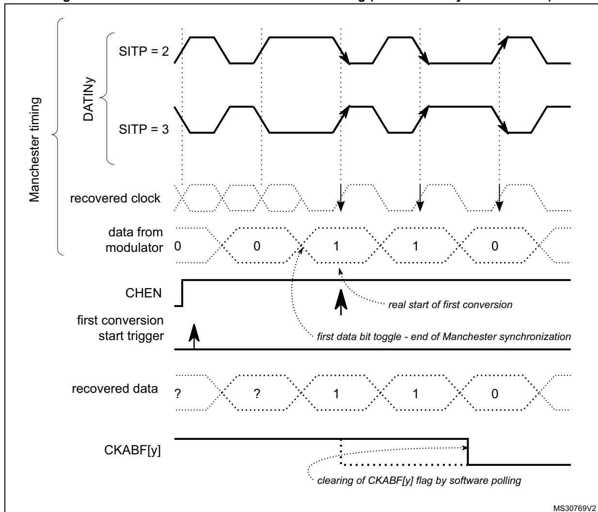
Figure 229. First conversion for Manchester coding (Manchester synchronization)
