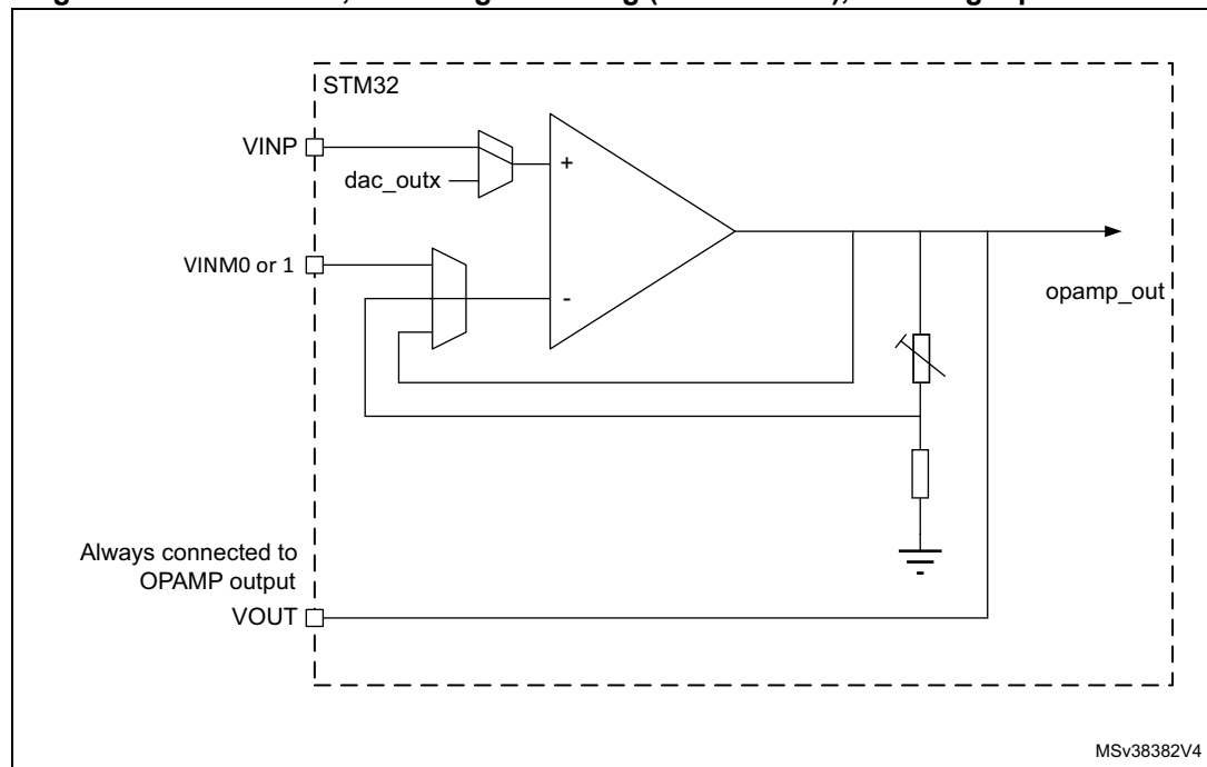
Figure 218. PGA mode, internal gain setting (x2/x4/x8/x16), inverting input not used
