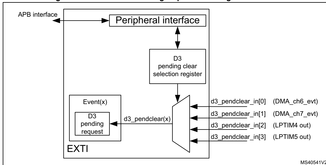
Figure 92. D3 domain Pending request clear logic
