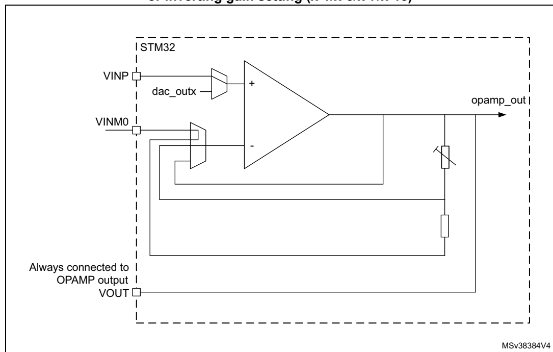
Figure 221. Example configuration
