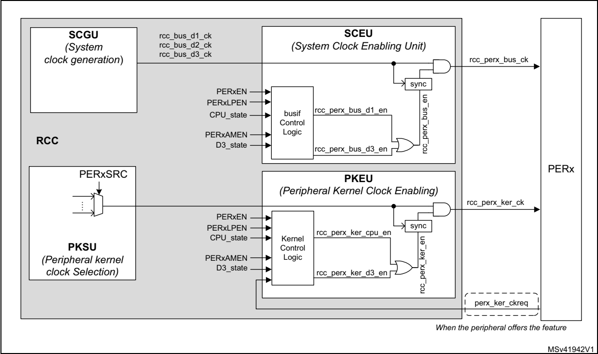
Figure 59. Peripheral kernel clock enable logic details
