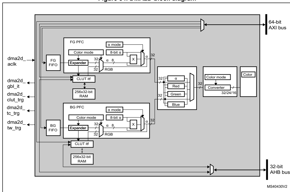
Figure 84. DMA2D block diagram
