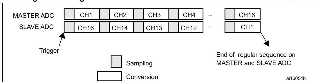
Figure 185. Regular simultaneous mode on 16 channels: dual ADC mode
