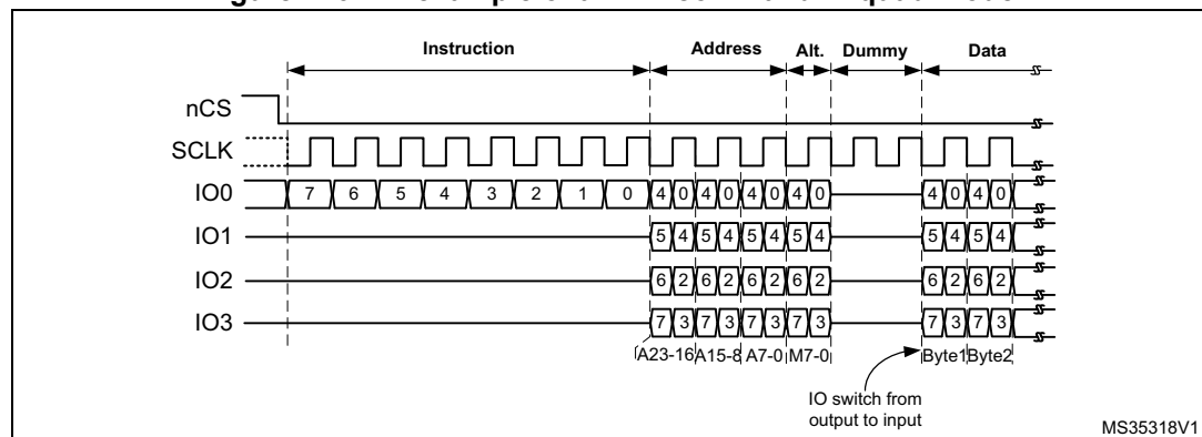
Figure 126. An example of a DDR command in quad mode
