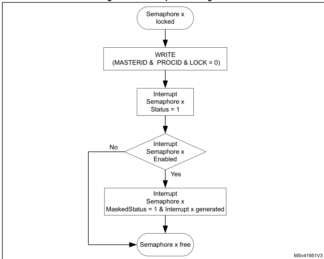
Figure 66. Interrupt state diagram
