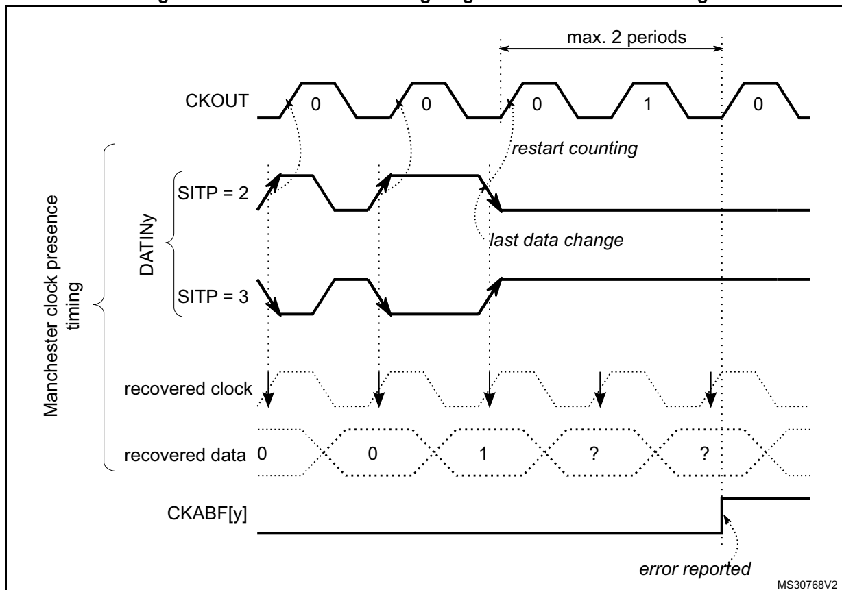
Figure 228. Clock absence timing diagram for Manchester coding
