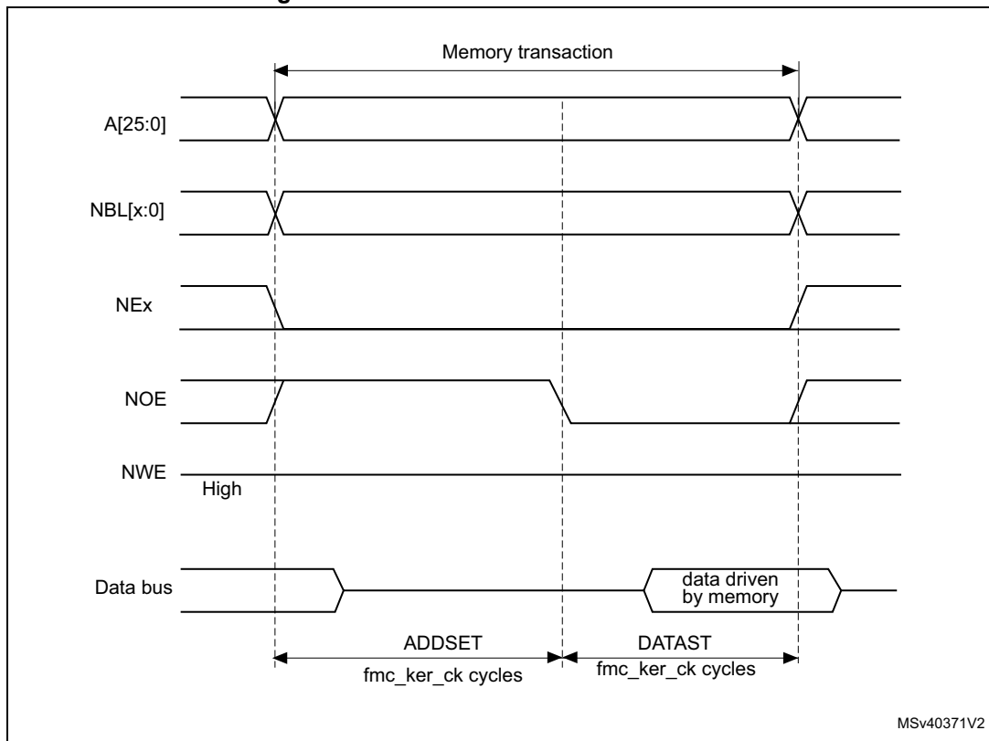
Figure 98. Mode A read access waveforms
