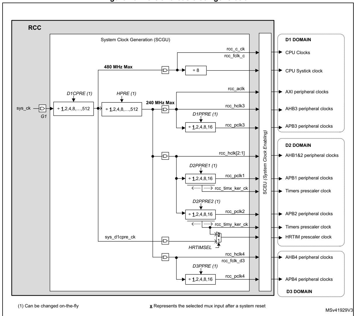
Figure 46. Core and bus clock generation
