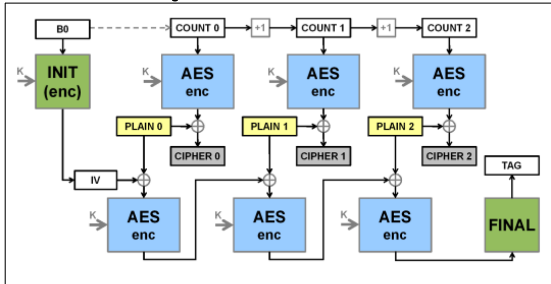
Figure 256. AES-CCM mode overview
