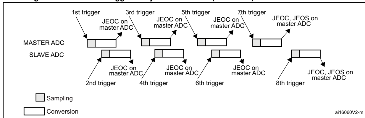
Figure 190. Alternate trigger: 4 injected channels (each ADC) in discontinuous mode
