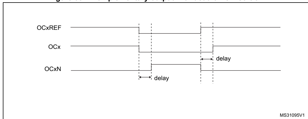
Figure 384. Complementary output with dead-time insertion
