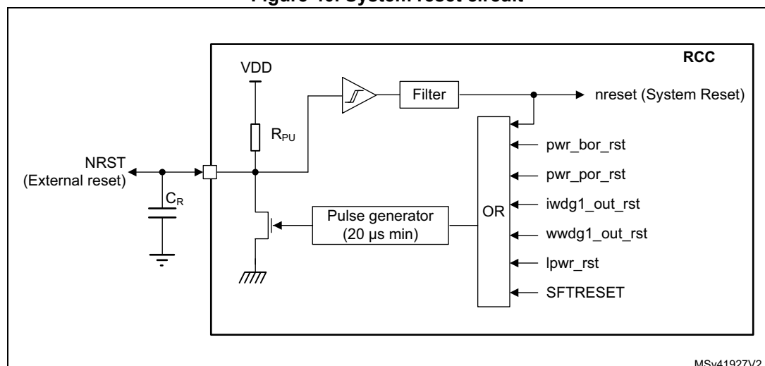
Figure 40. System reset circuit
