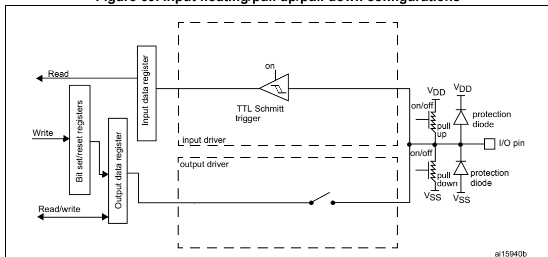
Figure 69. Input floating/pull up/pull down configurations
