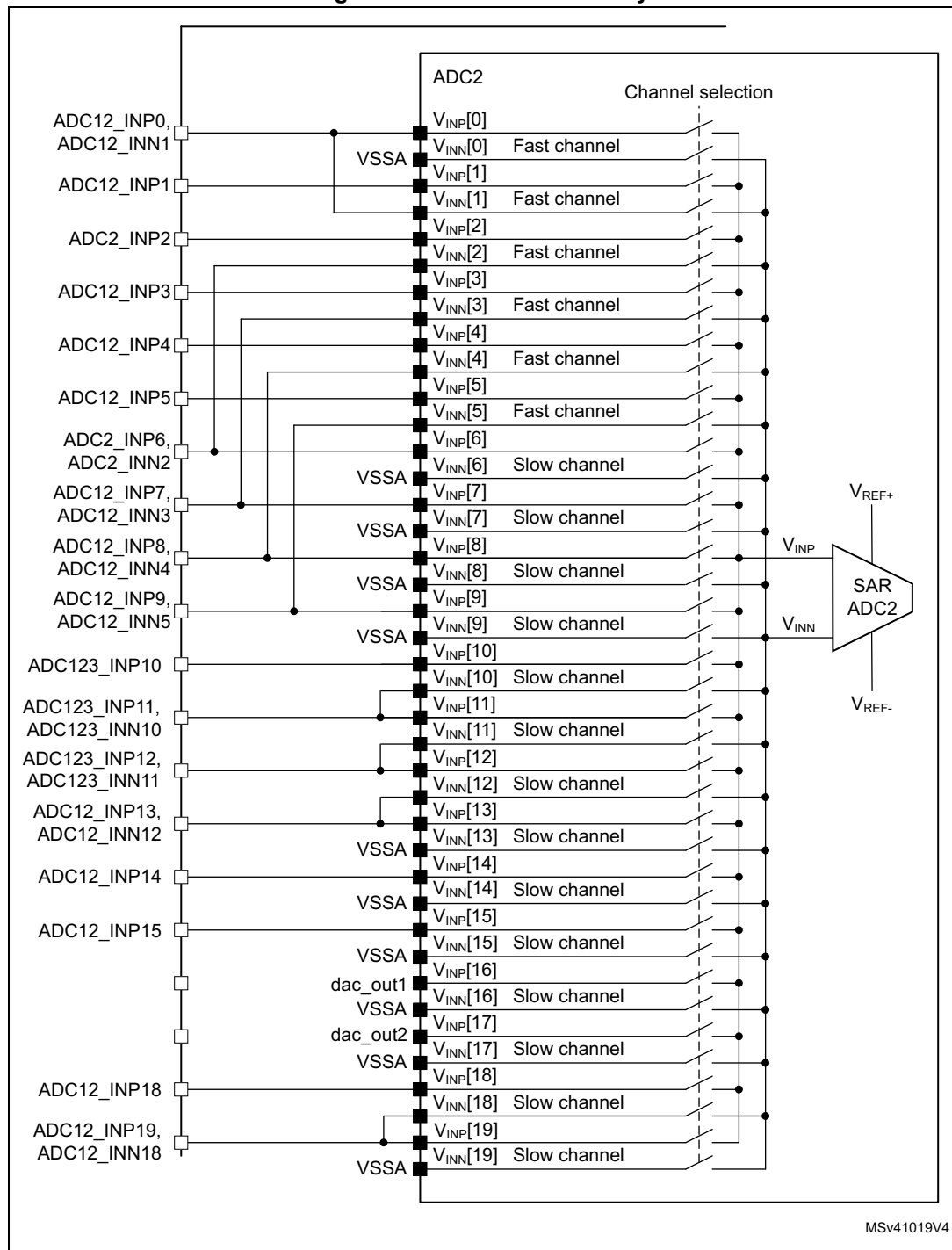
Figure 135. ADC2 connectivity
