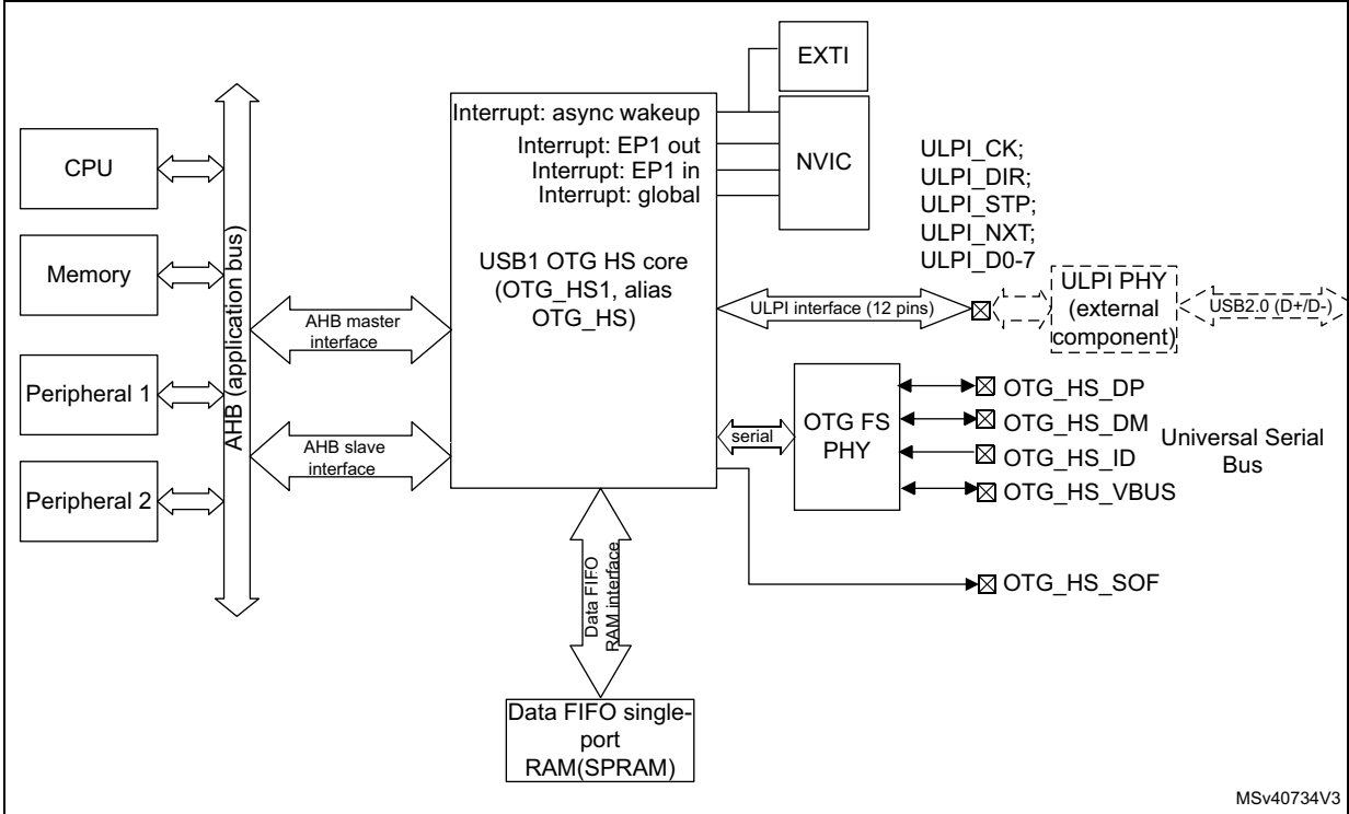
Figure 747. USB1 OTG high-speed block diagram (OTG_HS1)
