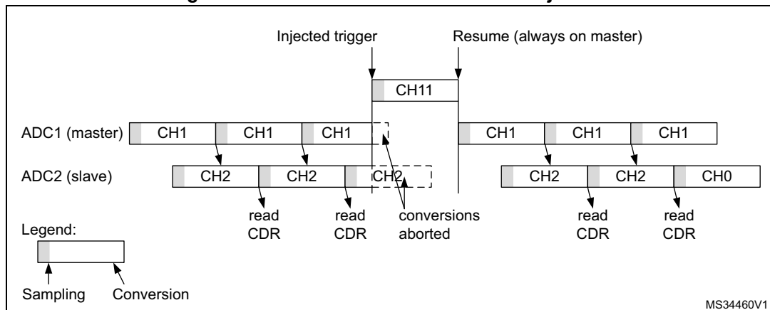
Figure 188. Interleaved conversion with injection
