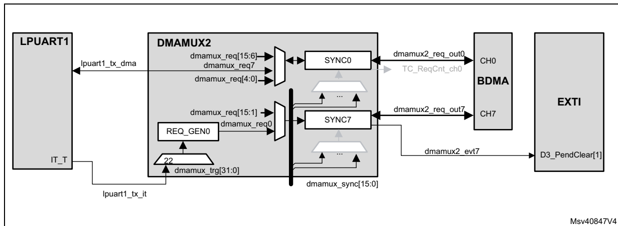
Figure 37. BDMA and DMAMUX2 interconnection
