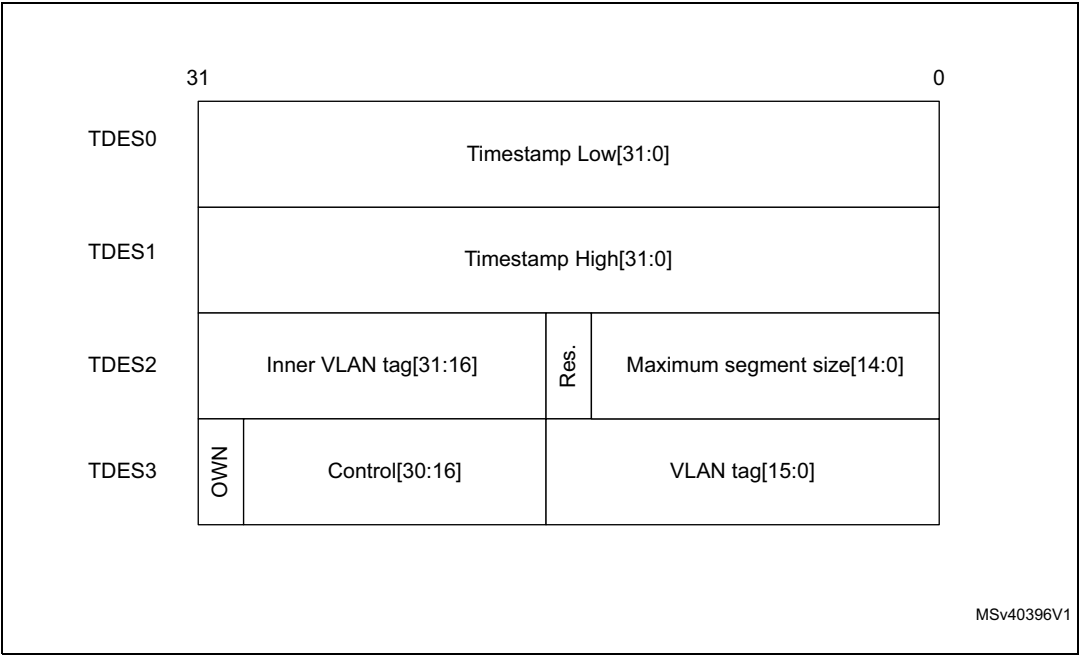
Figure 801. Transmit context descriptor format
