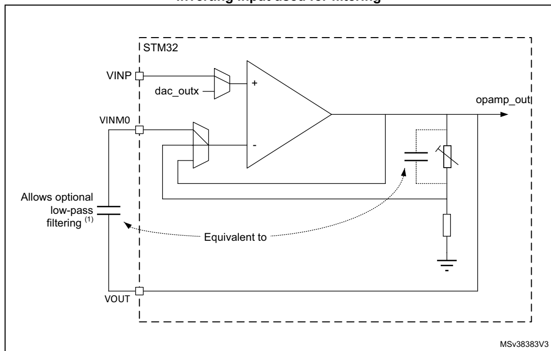
Figure 219. PGA mode, internal gain setting (x2/x4/x8/x16), inverting input used for filtering
