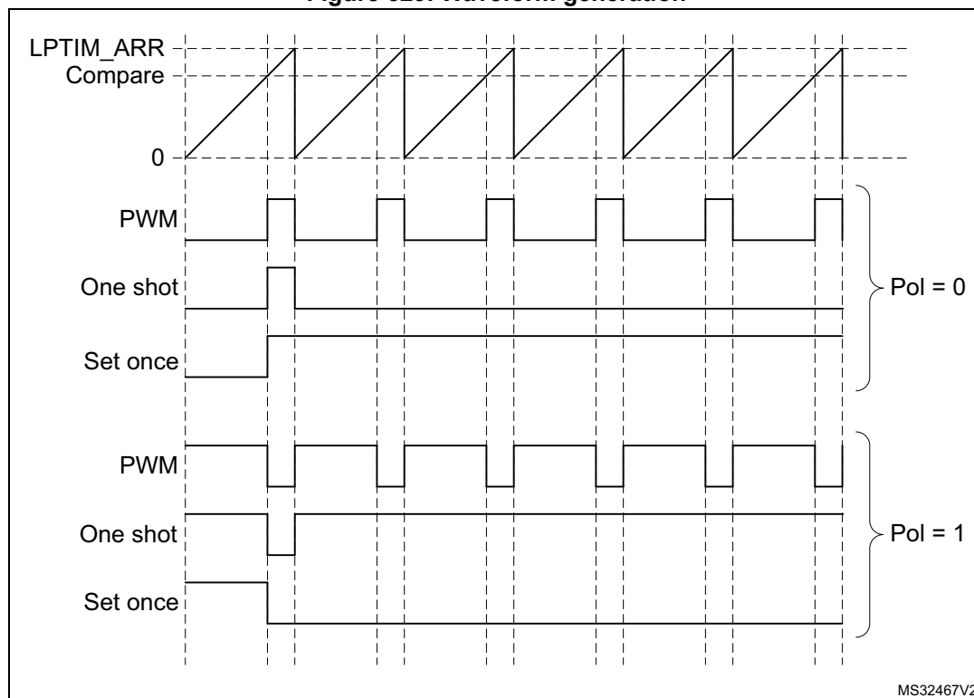
Figure 529. Waveform generation
