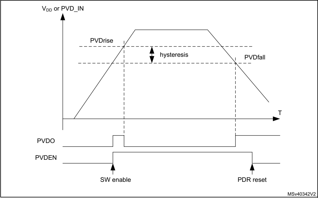
Figure 25. PVD thresholds
