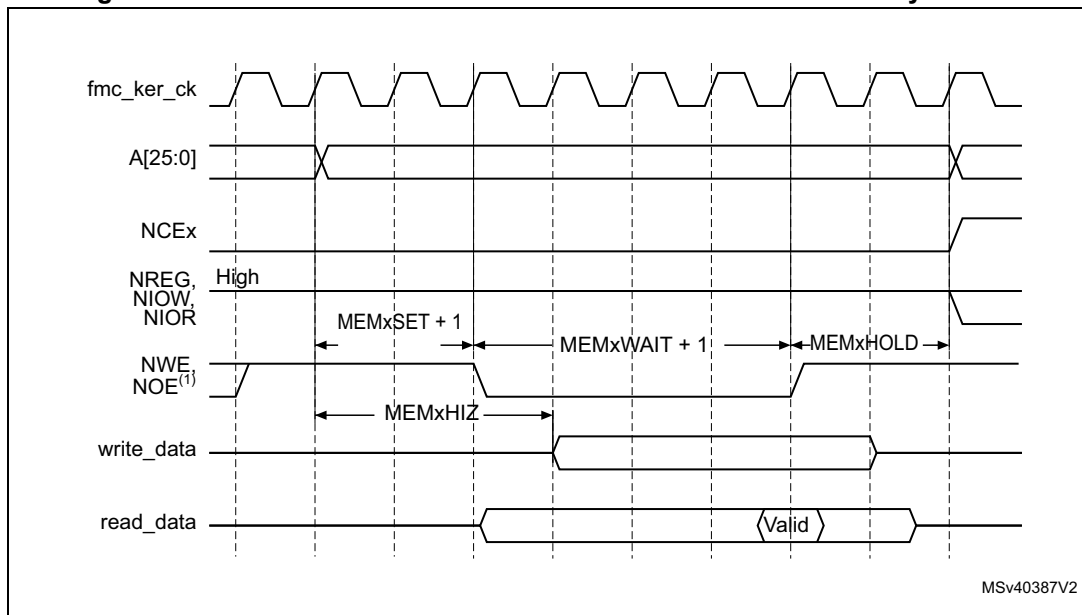
Figure 114. NAND Flash controller waveforms for common memory access
