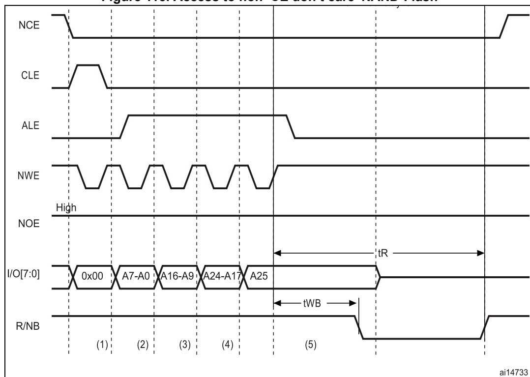
Figure 115. Access to non 'CE don't care' NAND-Flash
