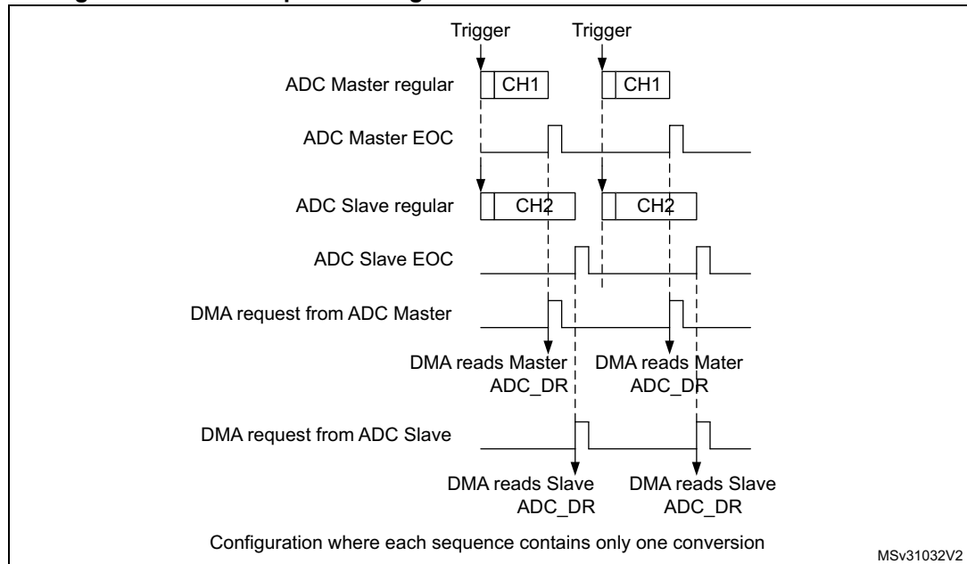
Figure 196. DMA Requests in regular simultaneous mode when DAMDF=0b00
