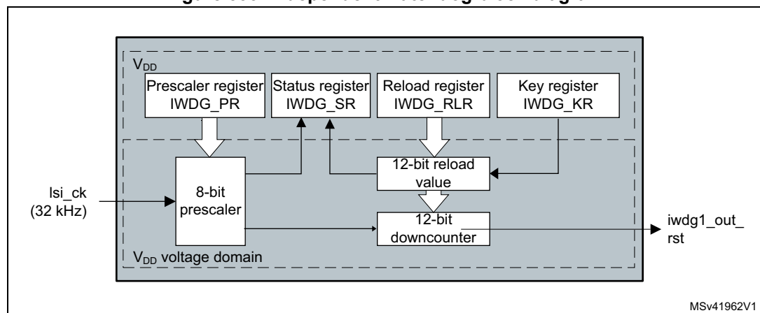
Figure 533. Independent watchdog block diagram
