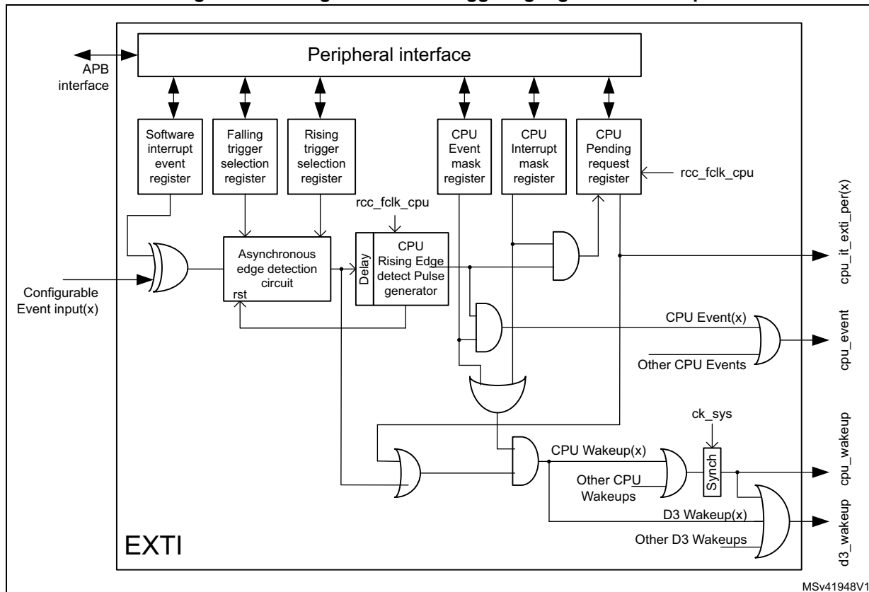
Figure 88. Configurable event triggering logic CPU wakeup
