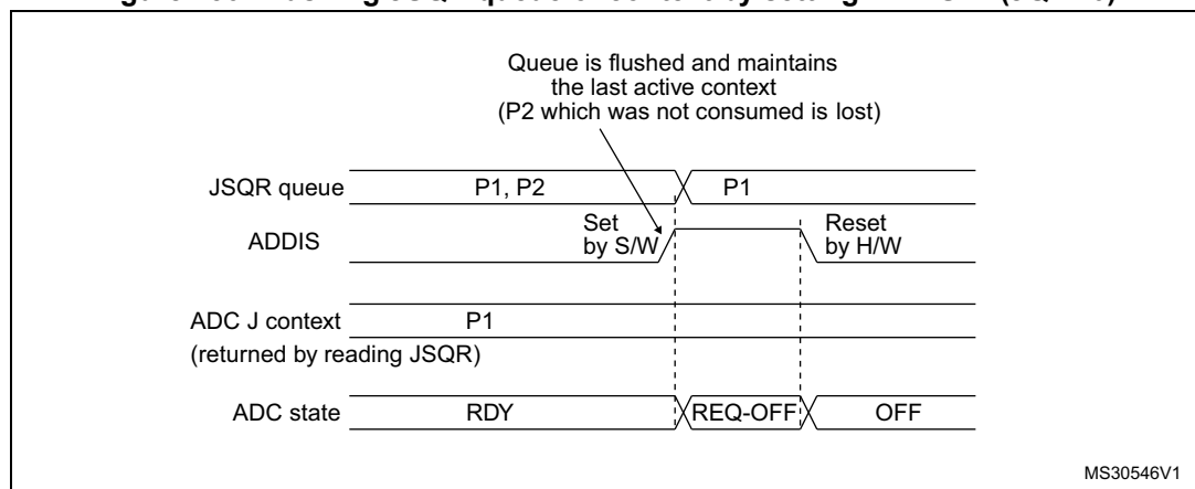
Figure 156. Flushing JSQR queue of context by setting ADDIS=1 (JQM=0)
