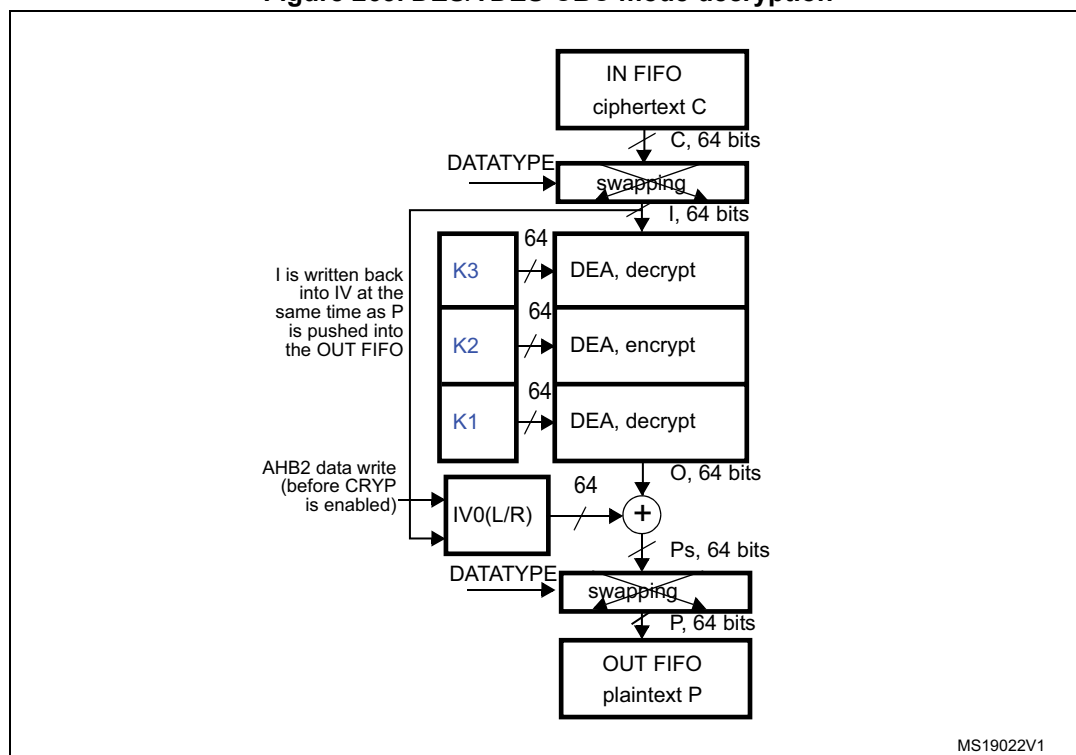
Figure 263. DES/TDES-CBC mode decryption
