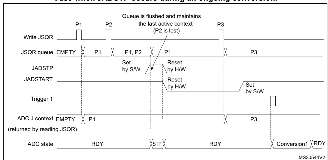
Figure 152. Flushing JSQR queue of context by setting JADSTP=1 (JQM=0). Case when JADSTP occurs during an ongoing conversion.
