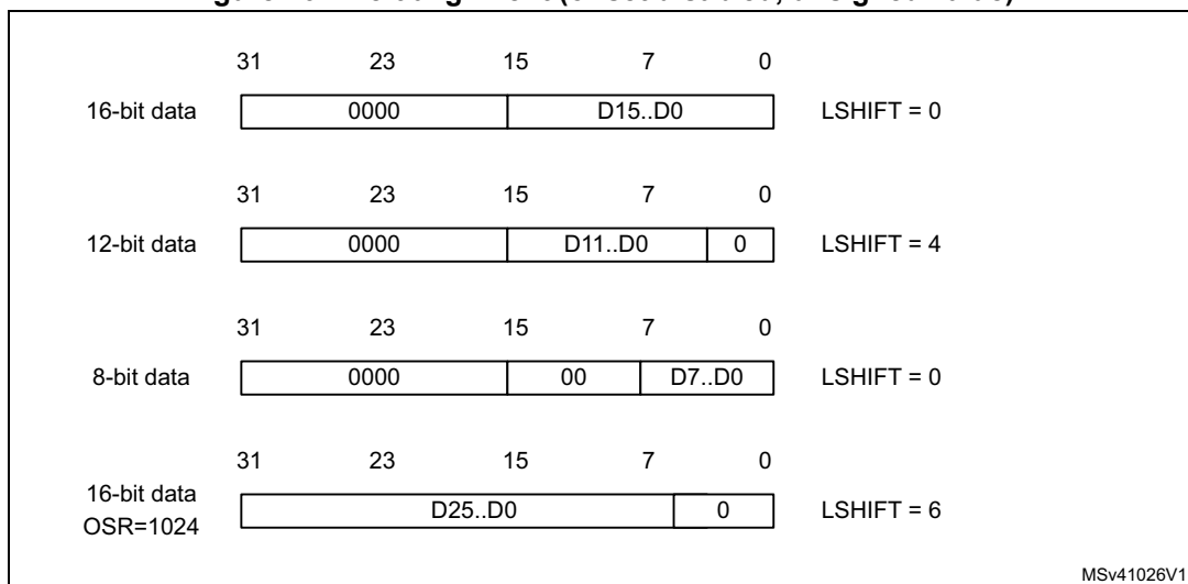
Figure 164. Left alignment (offset disabled, unsigned value)
