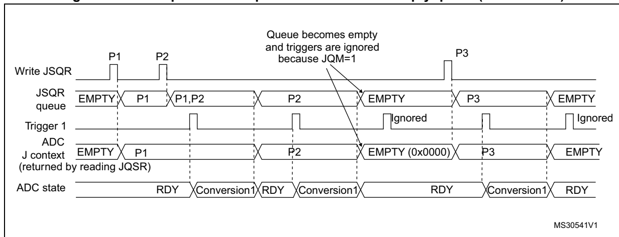
Figure 151. Example of JSQR queue of context with empty queue (case JQM=1)
