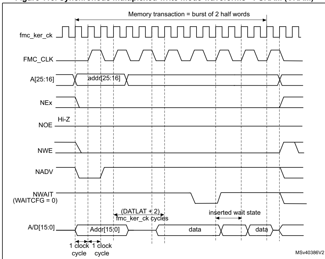
Figure 113. Synchronous multiplexed write mode waveforms - PSRAM (CRAM)
