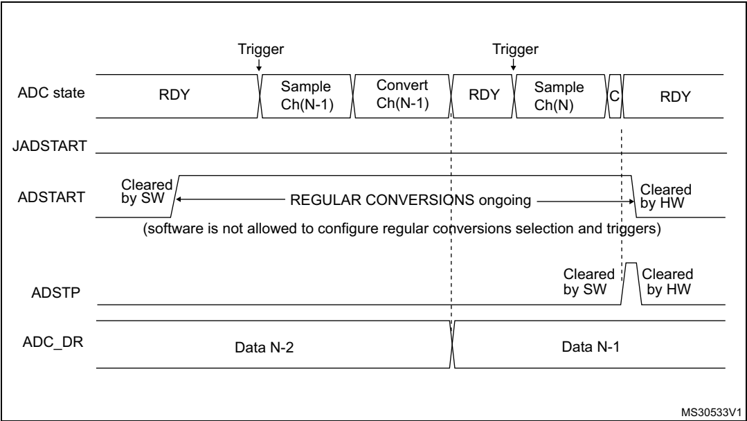
Figure 142. Stopping ongoing regular conversions
