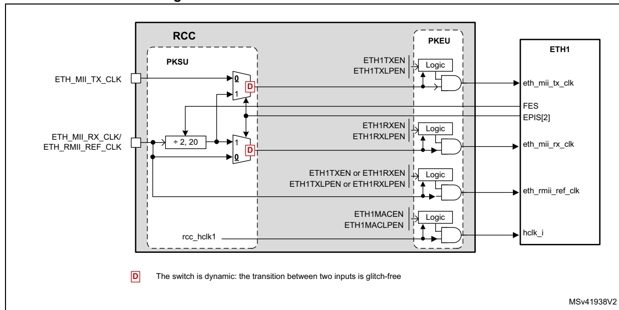
Figure 54. Kernel clock distribution for Ethernet
