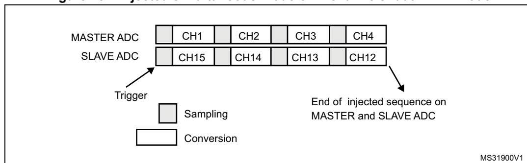
Figure 184. Injected simultaneous mode on 4 channels: dual ADC mode
