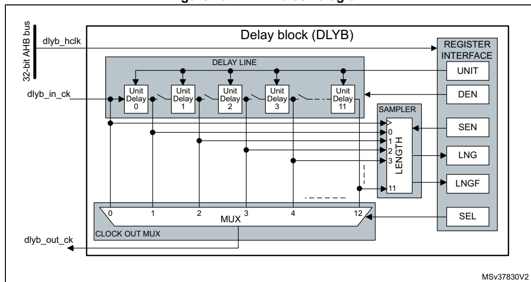
Figure 131. DLYB block diagram
