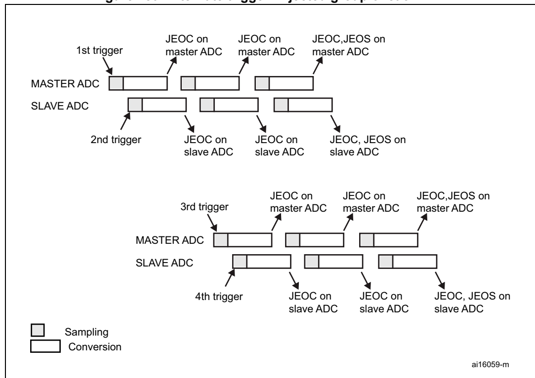
Figure 189. Alternate trigger: injected group of each ADC
