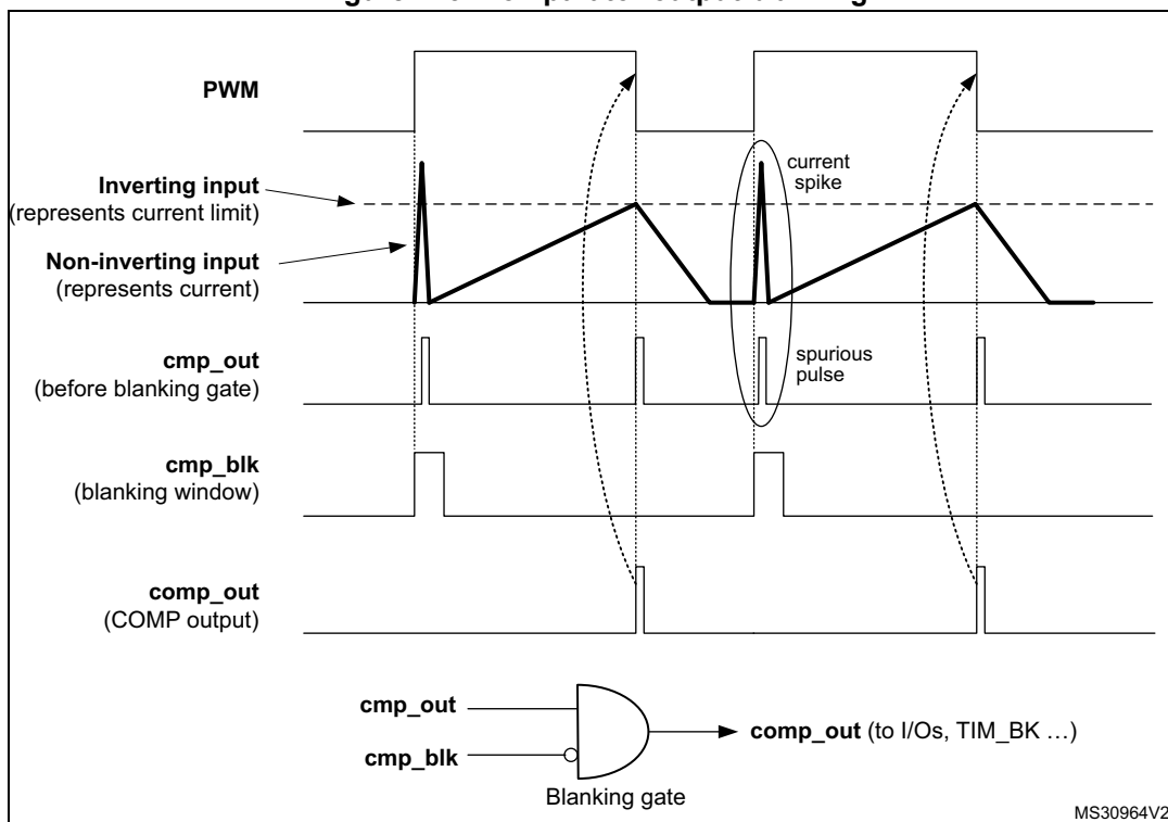
Figure 213. Comparator output blanking
