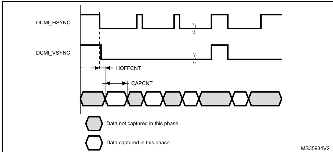
Figure 239. Data capture waveforms
