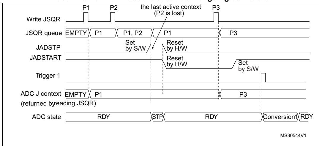
Figure 154. Flushing JSQR queue of context by setting JADSTP=1 (JQM=0). Case when JADSTP occurs outside an ongoing conversion
