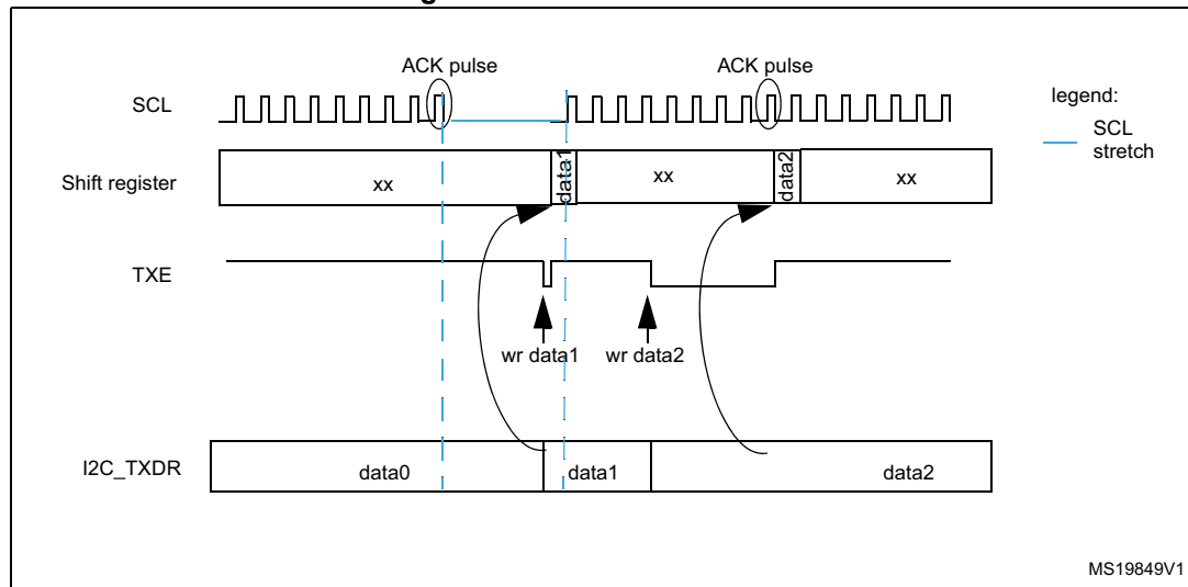
Figure 542. Data transmission
