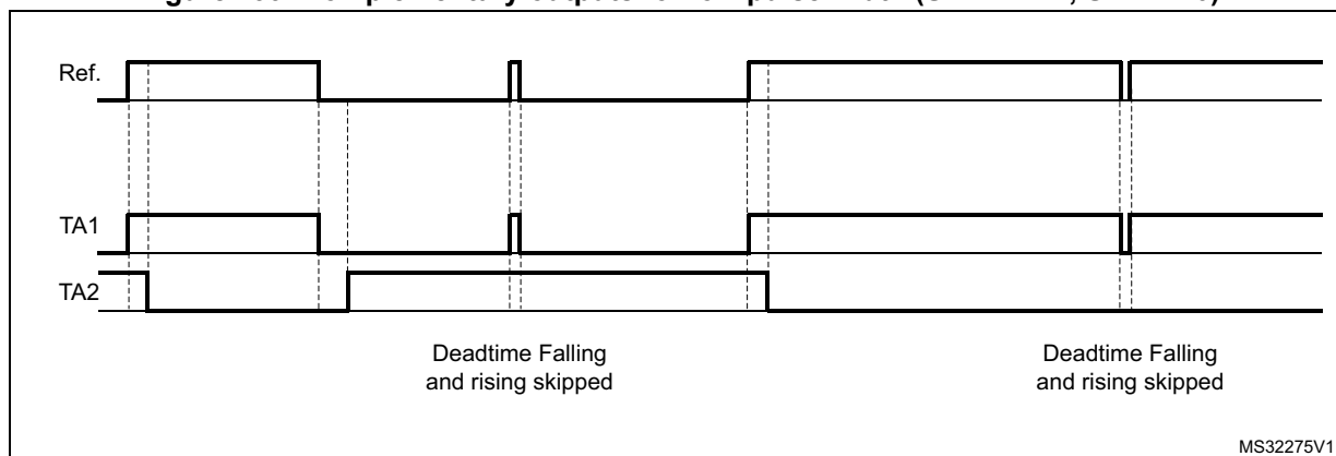
Figure 299. Complementary outputs for low pulse width (SDTRx = 1, SDTFx=0)
