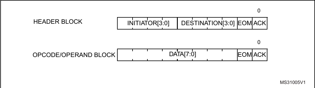
Figure 808. Blocks
