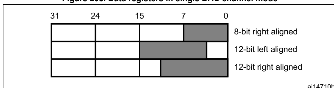
Figure 203. Data registers in single DAC channel mode
