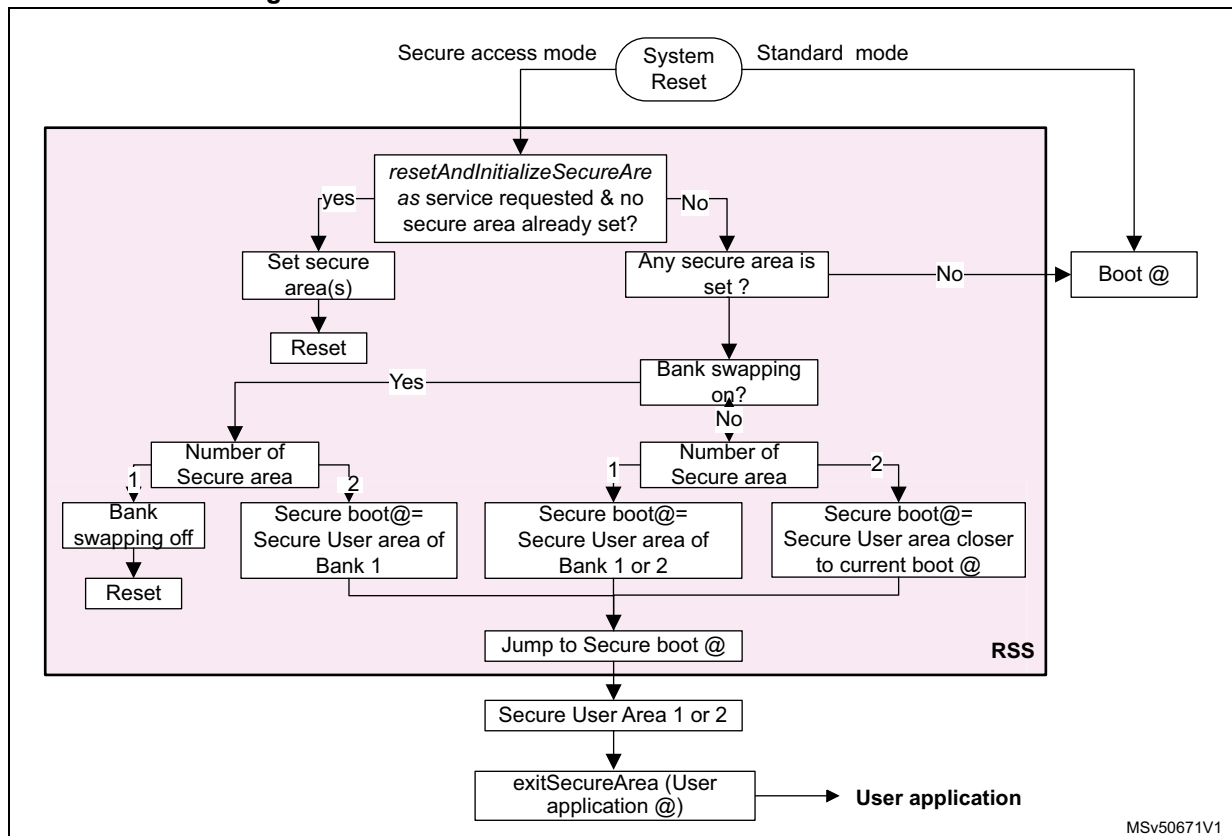
Figure 14. Bootloader state machine in Secure access mode
