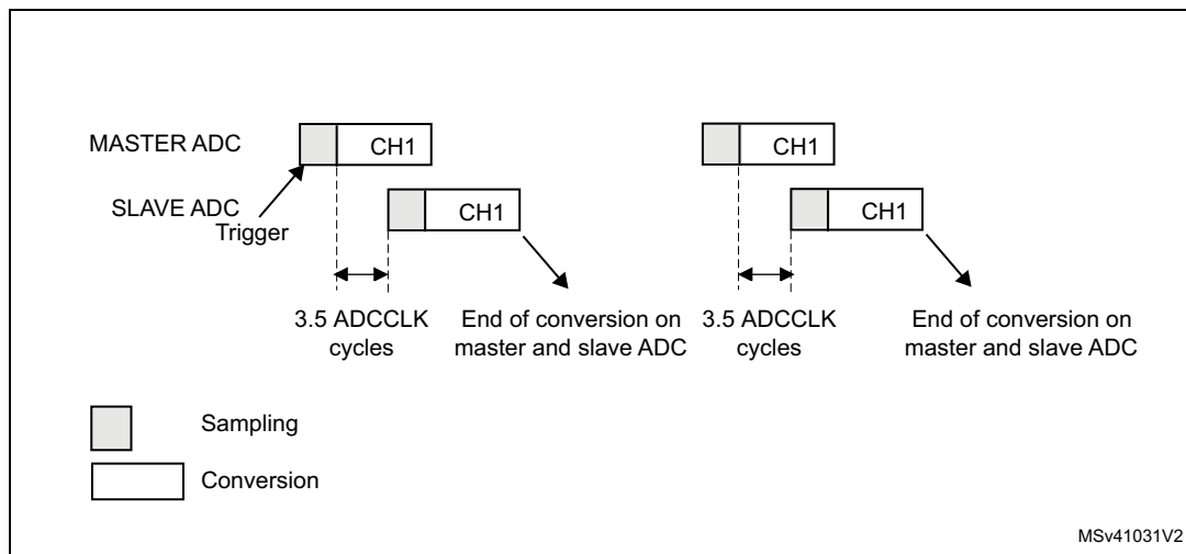
Figure 187. Interleaved mode on 1 channel in single conversion mode: dual ADC mode
