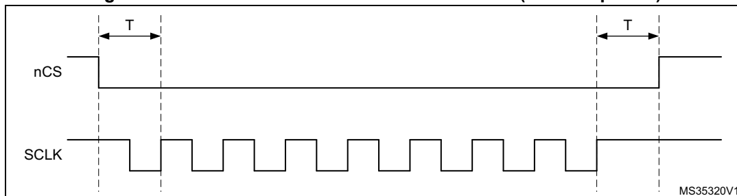
Figure 128. nCS when CKMODE = 1 in SDR mode ( T = \text{CLK period} )
