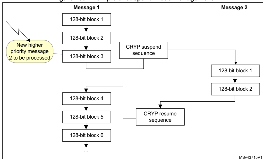
Figure 259. Example of suspend mode management
