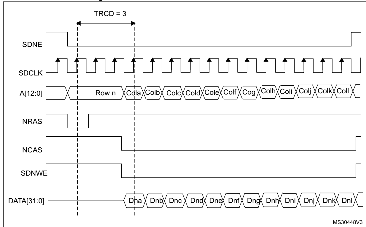
Figure 116. Burst write SDRAM access waveforms
