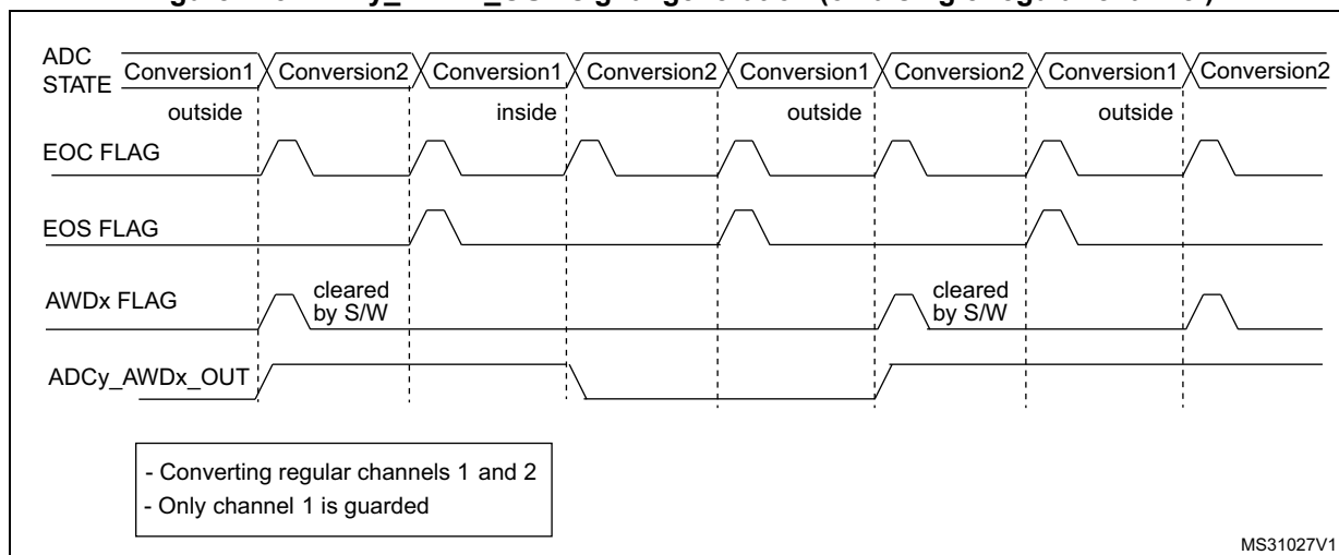
Figure 175. ADCy_AWDx_OUT signal generation (on a single regular channel)
