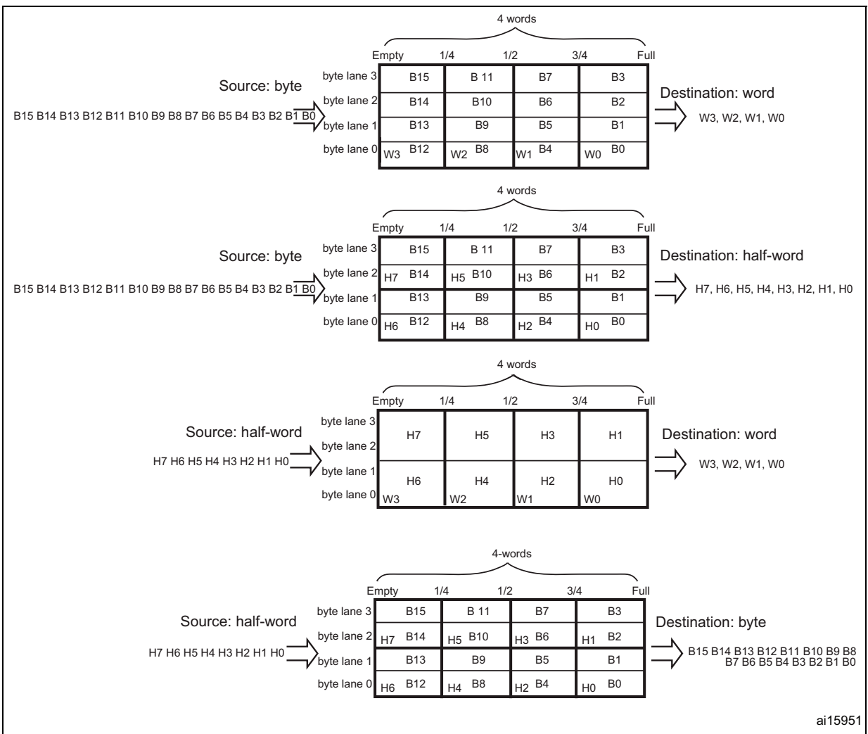
Figure 79. FIFO structure
