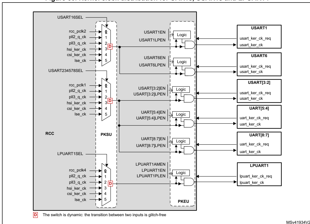
Figure 50. Kernel clock distribution for UARTs, USARTs and LPUART1
