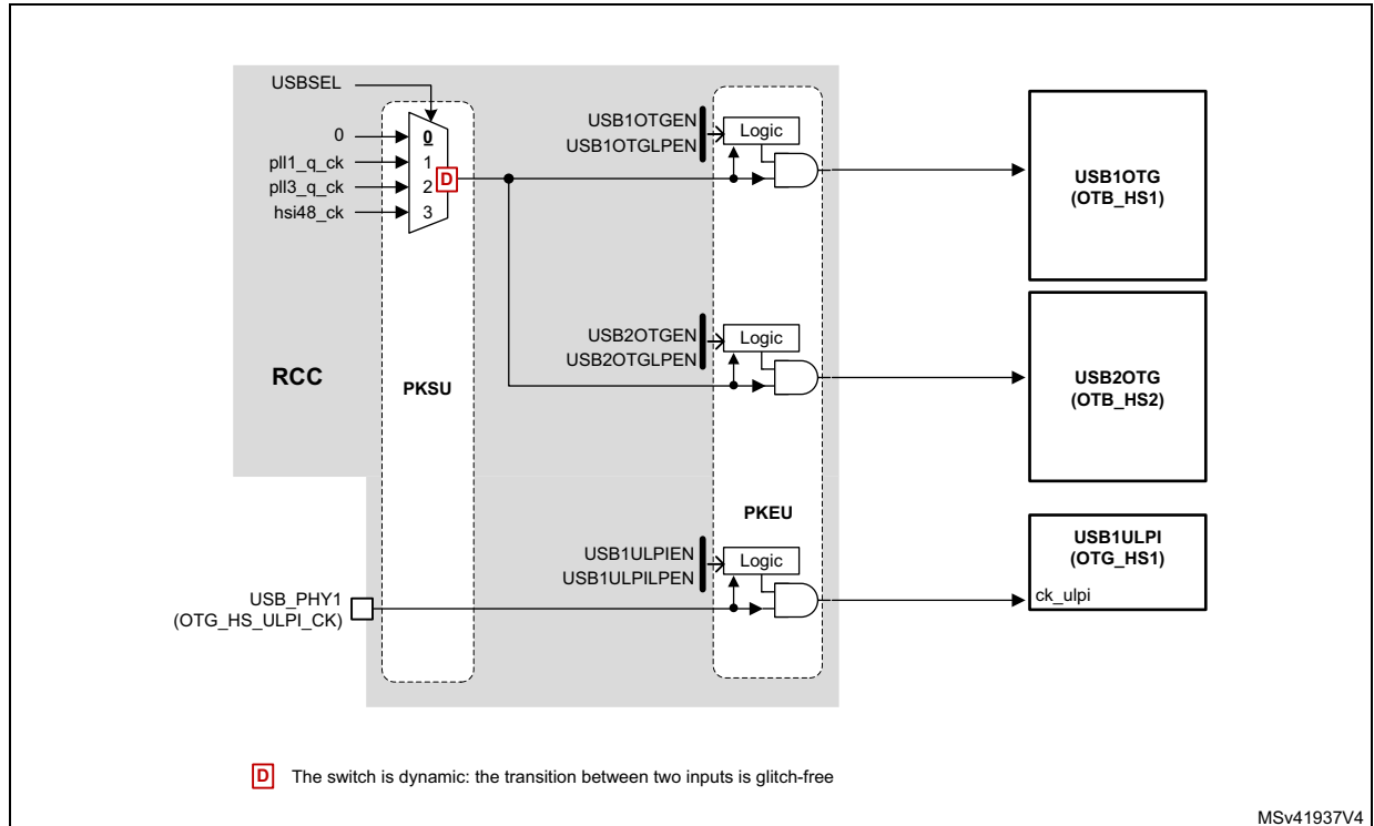
Figure 53. Kernel clock distribution for USB (2)
