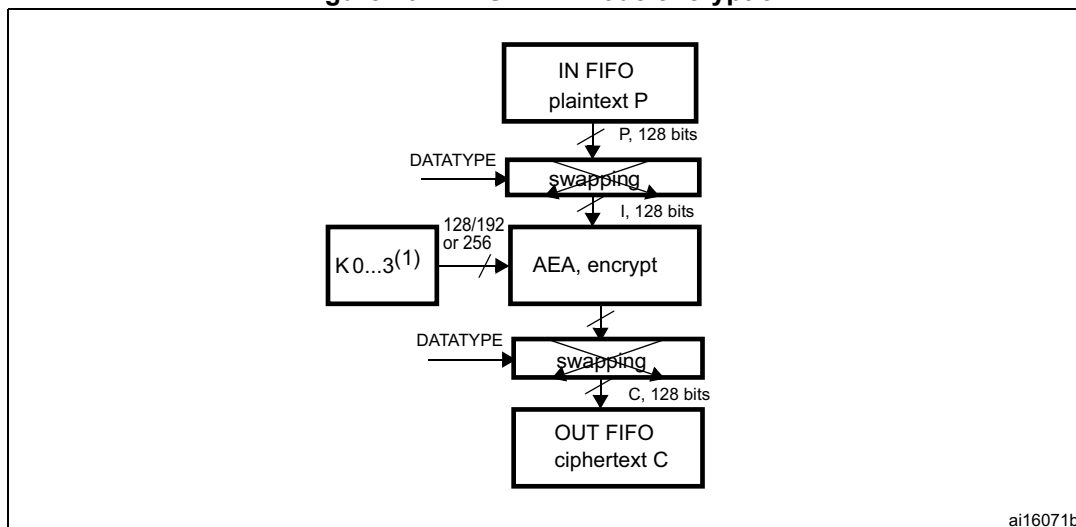
Figure 264. AES-ECB mode encryption
