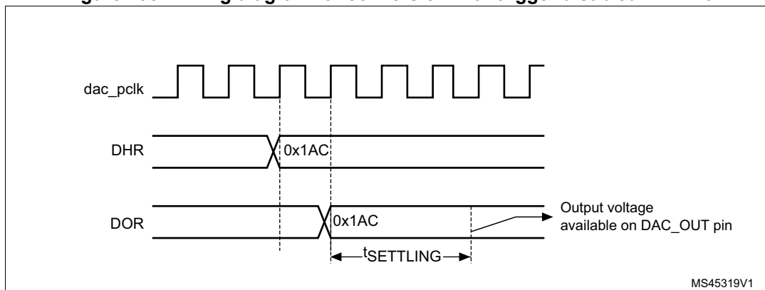
Figure 205. Timing diagram for conversion with trigger disabled TEN = 0
