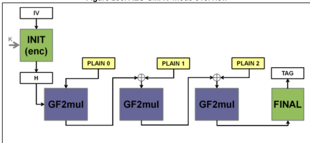
Figure 255. AES-GMAC mode overview
