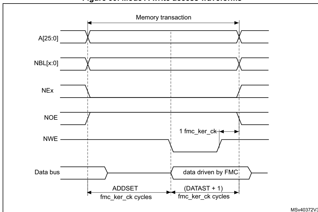
Figure 99. Mode A write access waveforms
