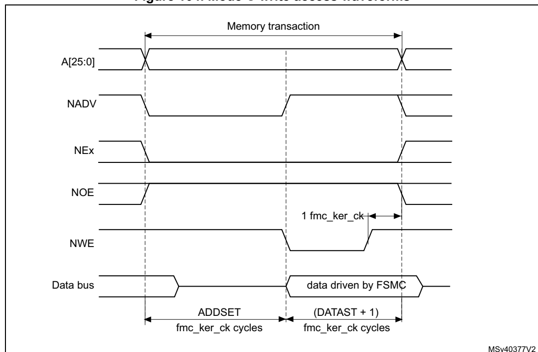
Figure 104. Mode C write access waveforms
