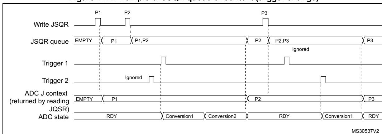
Figure 147. Example of JSQR queue of context (trigger change)
