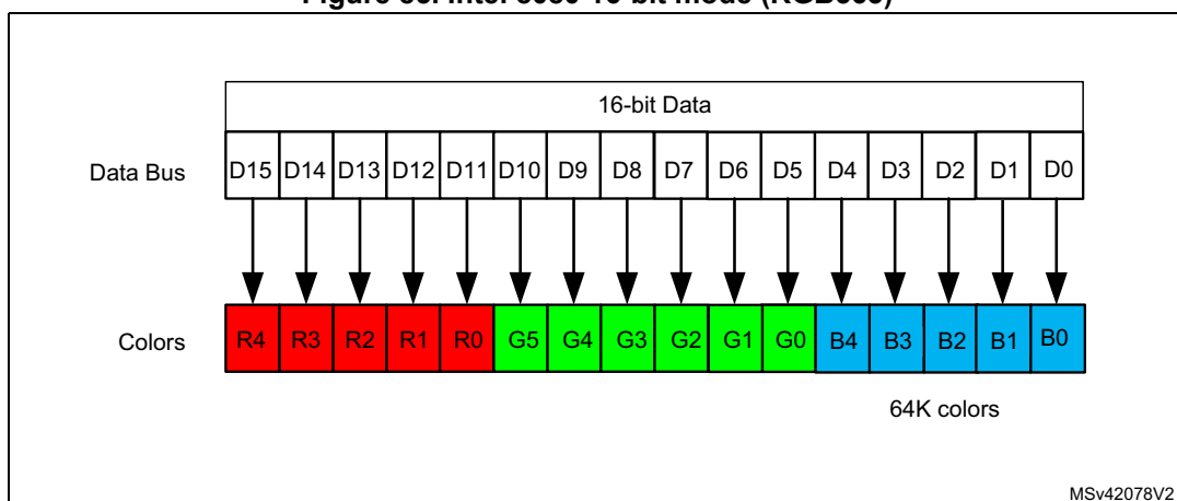
Figure 85. Intel 8080 16-bit mode (RGB565)
