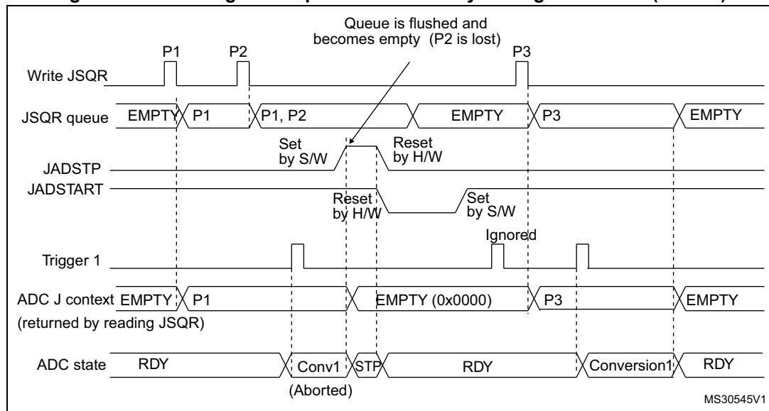
Figure 155. Flushing JSQR queue of context by setting JADSTP=1 (JQM=1)
