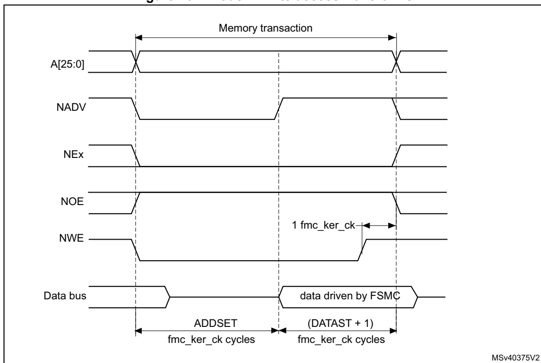
Figure 102. Mode B write access waveforms
