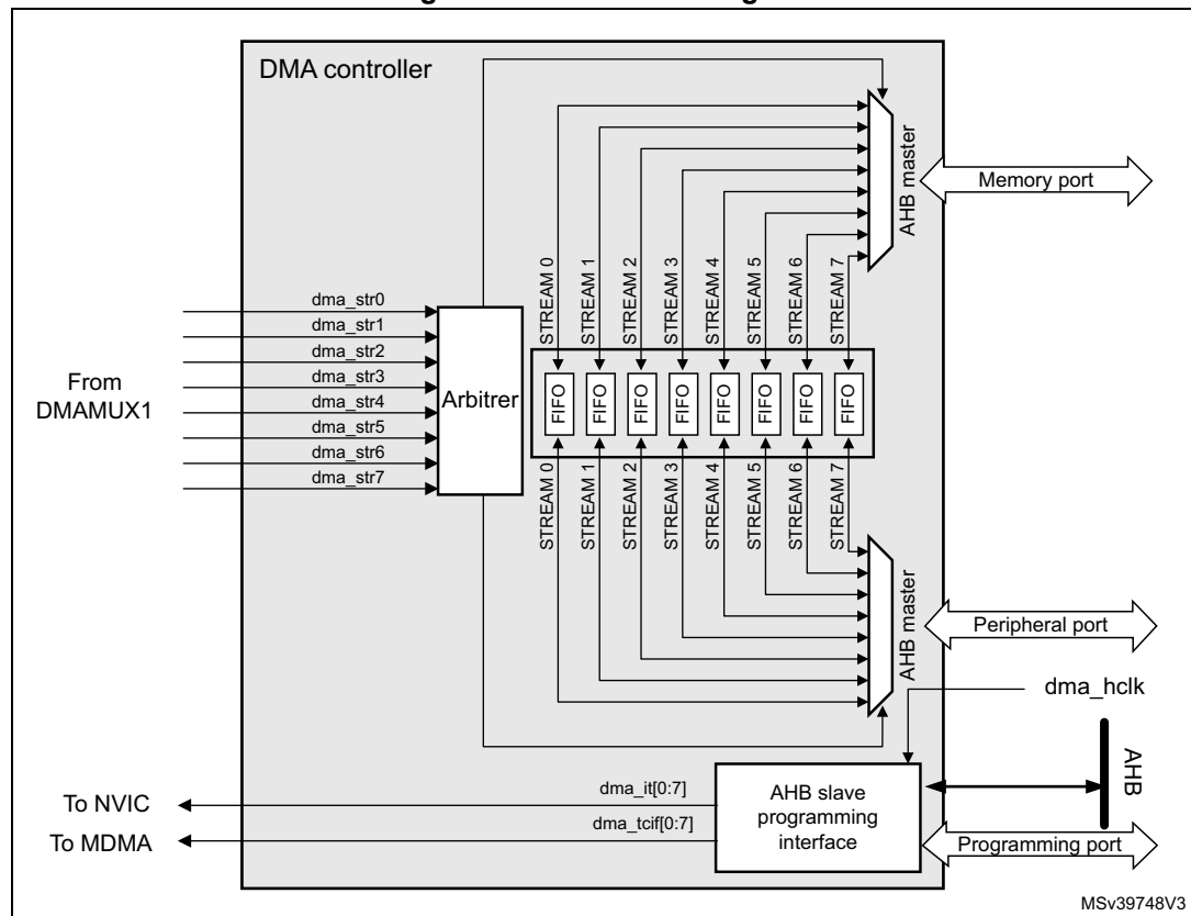
Figure 75. DMA block diagram
