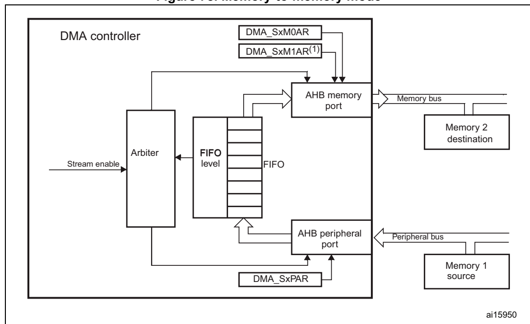
Figure 78. Memory-to-memory mode
