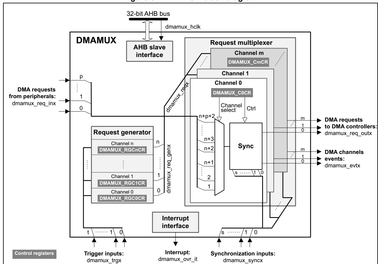
Figure 81. DMAMUX block diagram
