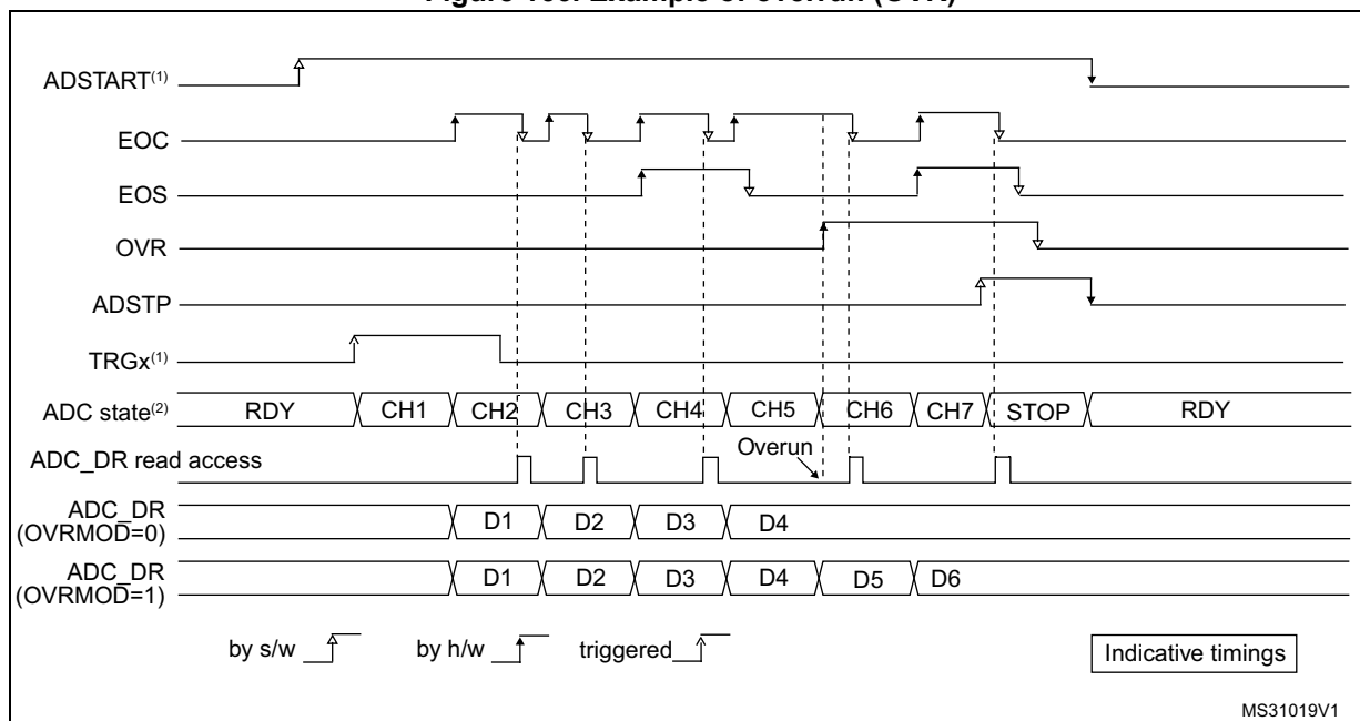
Figure 166. Example of overrun (OVR)
