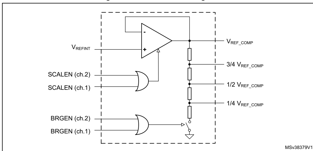
Figure 215. Scaler block diagram
