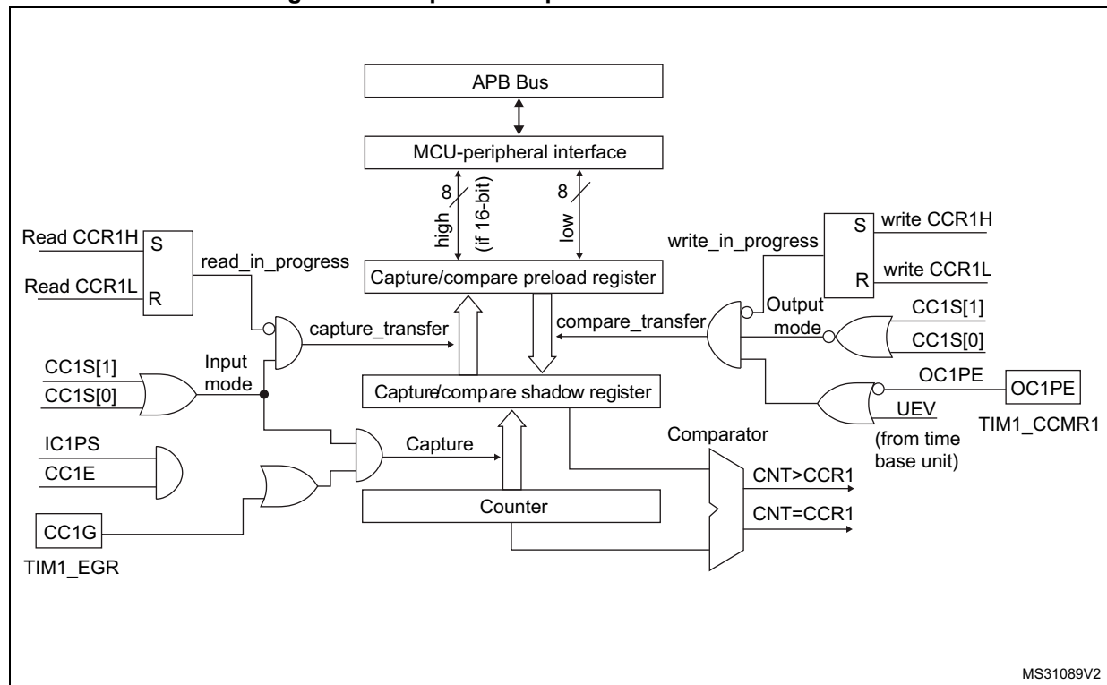
Figure 373. Capture/compare channel 1 main circuit
