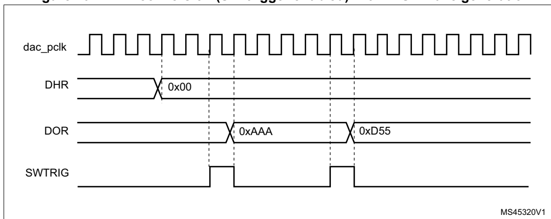
Figure 207. DAC conversion (SW trigger enabled) with LFSR wave generation
