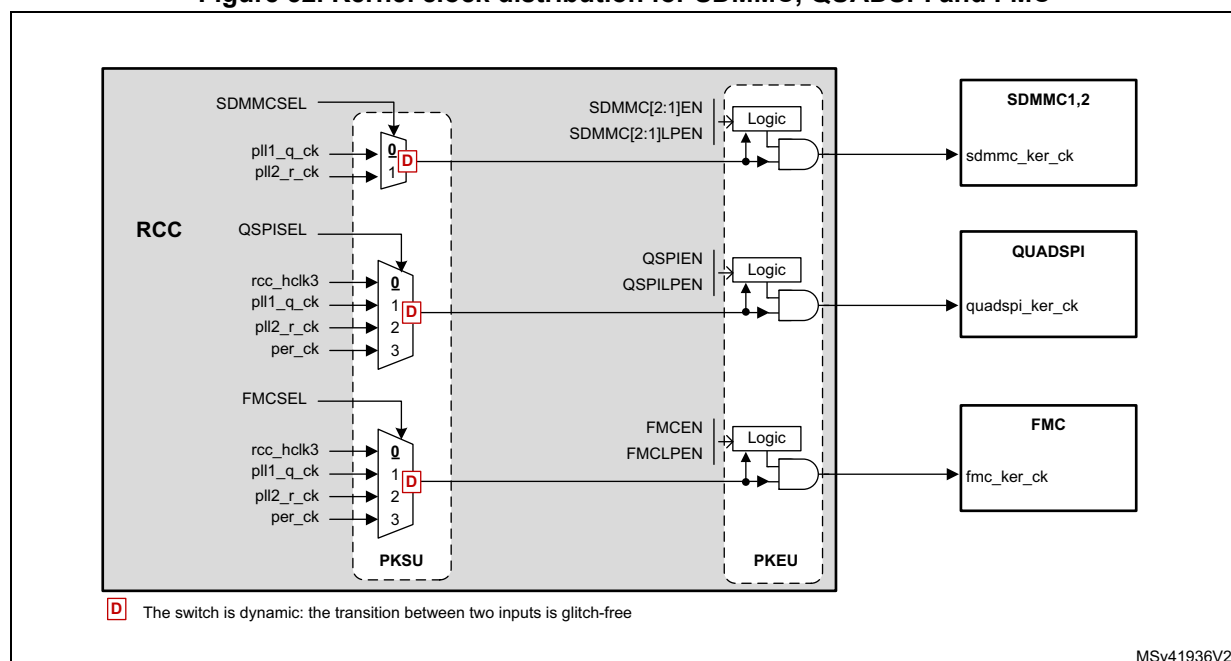
Figure 52. Kernel clock distribution for SDMMC, QUADSPI and FMC
