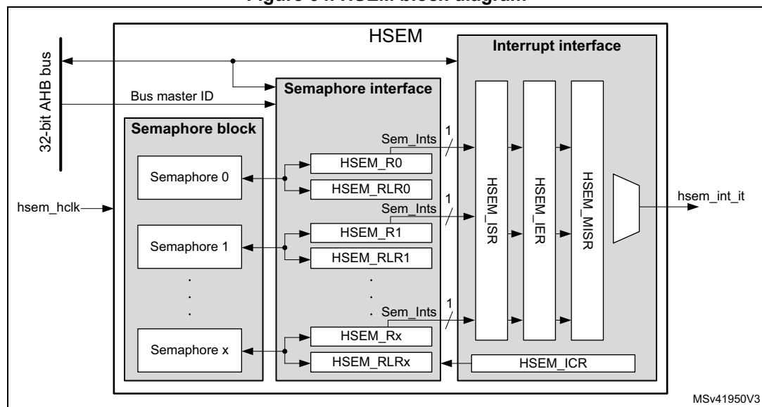
Figure 64. HSEM block diagram
