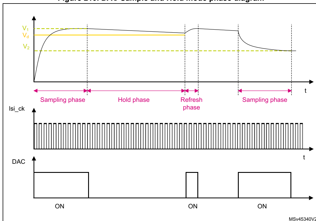
Figure 210. DAC Sample and Hold mode phase diagram
