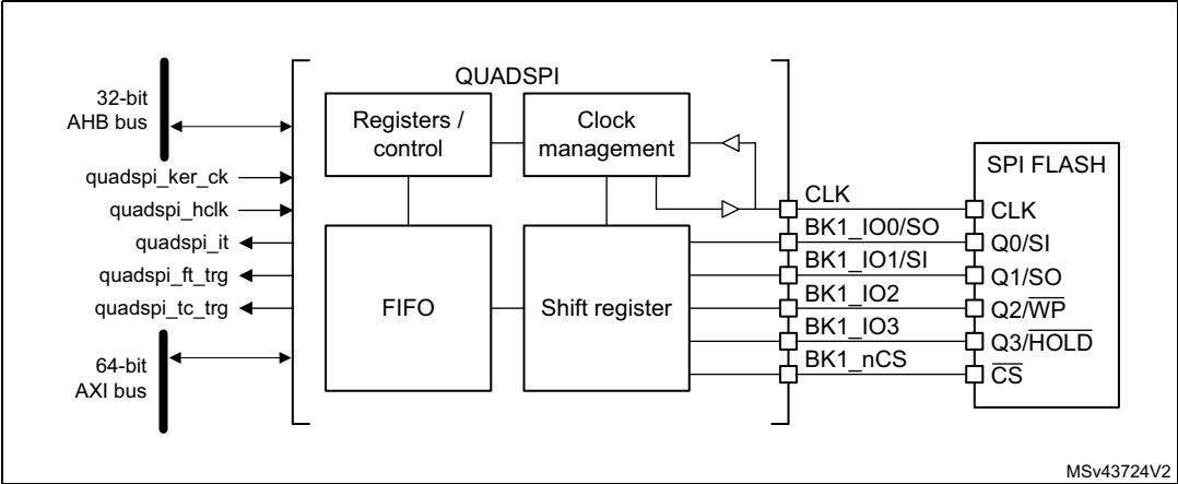
Figure 123. QUADSPI block diagram when dual-flash mode is disabled
