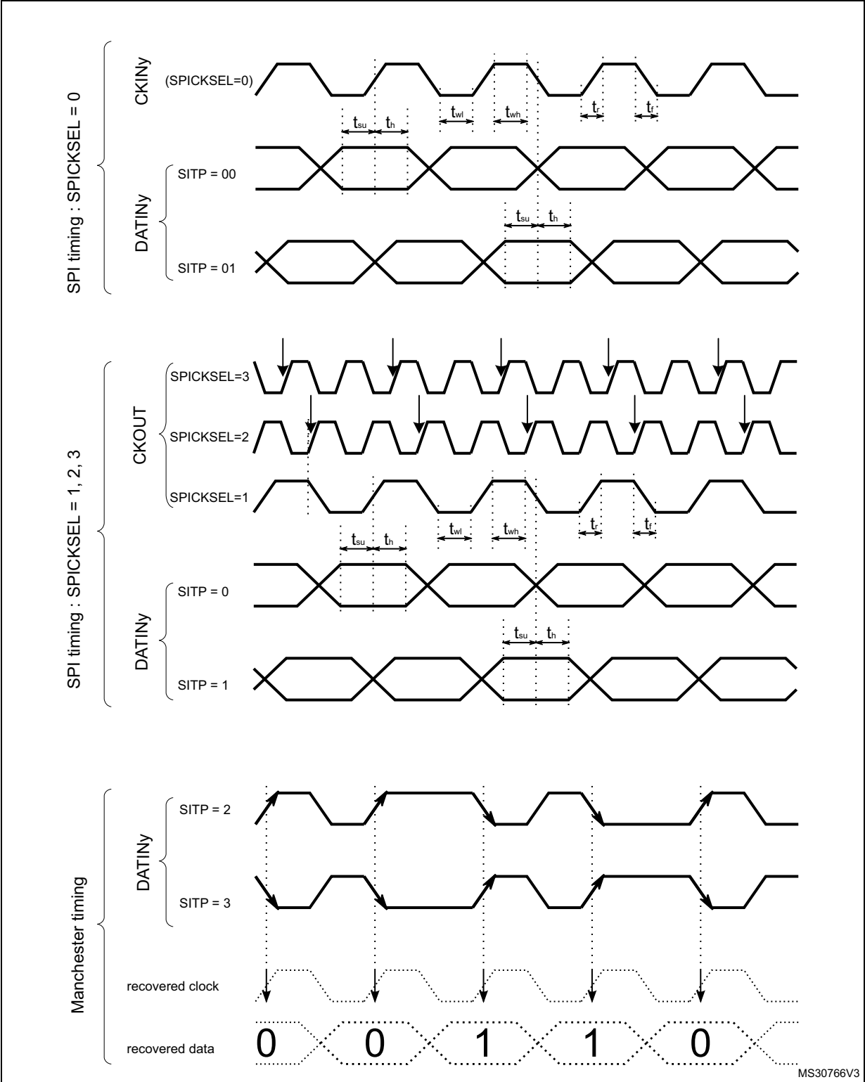
Figure 226. Channel transceiver timing diagrams
