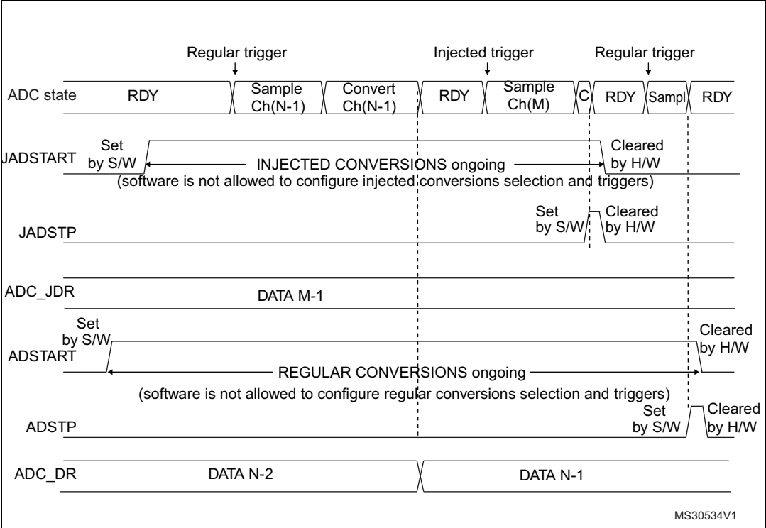
Figure 143. Stopping ongoing regular and injected conversions
