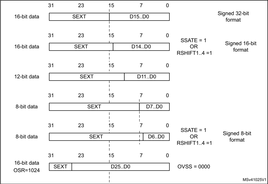
Figure 163. Right alignment (offset enabled, signed value)
