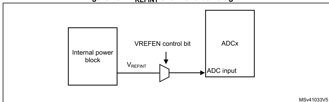
Figure 201. V_{REFINT} channel block diagram
