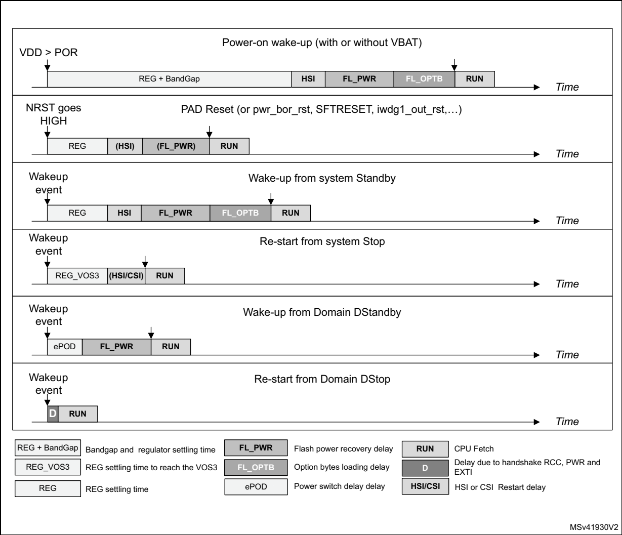
Figure 41. Boot sequences versus system states
