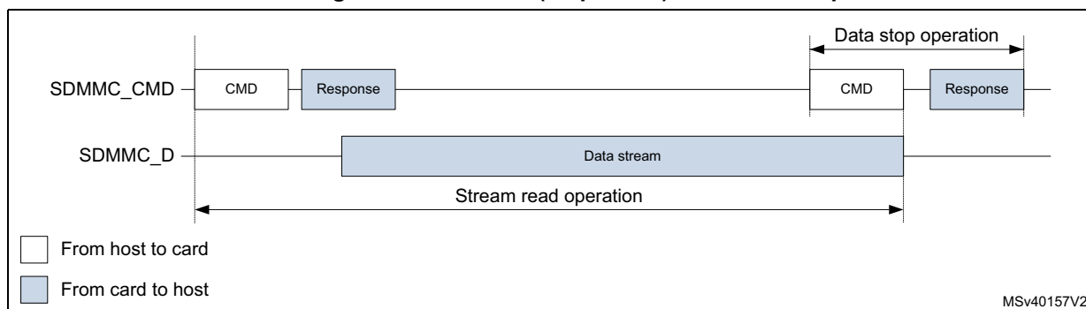
Figure 699. SDMMC (sequential) stream read operation
