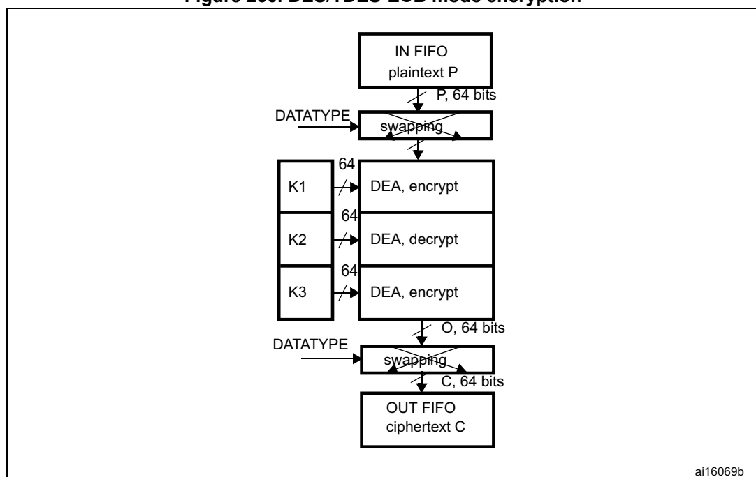
Figure 260. DES/TDES-ECB mode encryption
