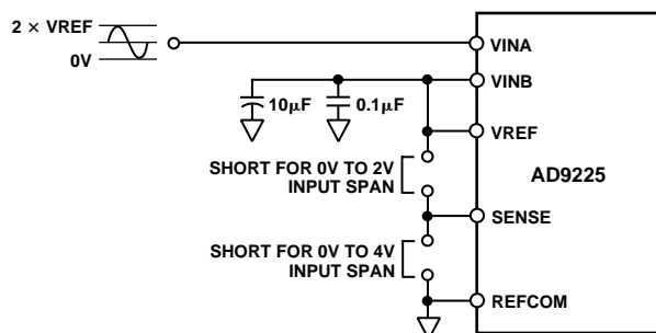
Figure 26. Internal Reference—2 V p-p Input Span, V_{CM} = 1 V, or 4 V p-p Input Span
