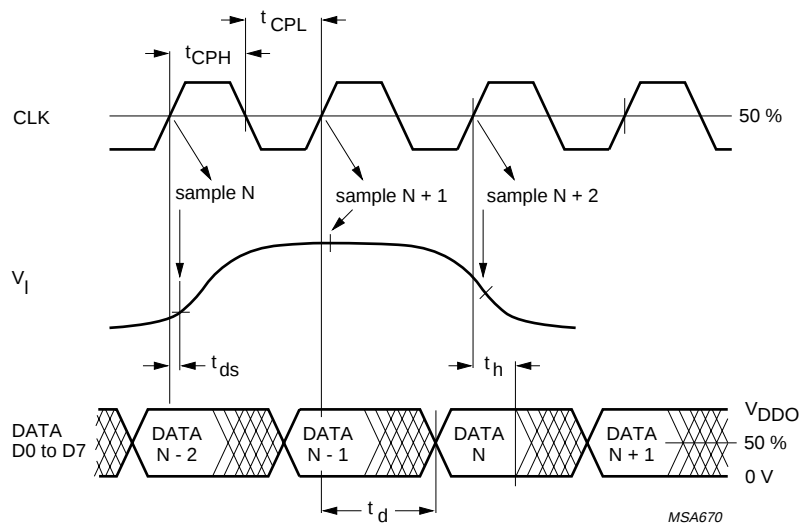
Fig.4 Timing diagram.
