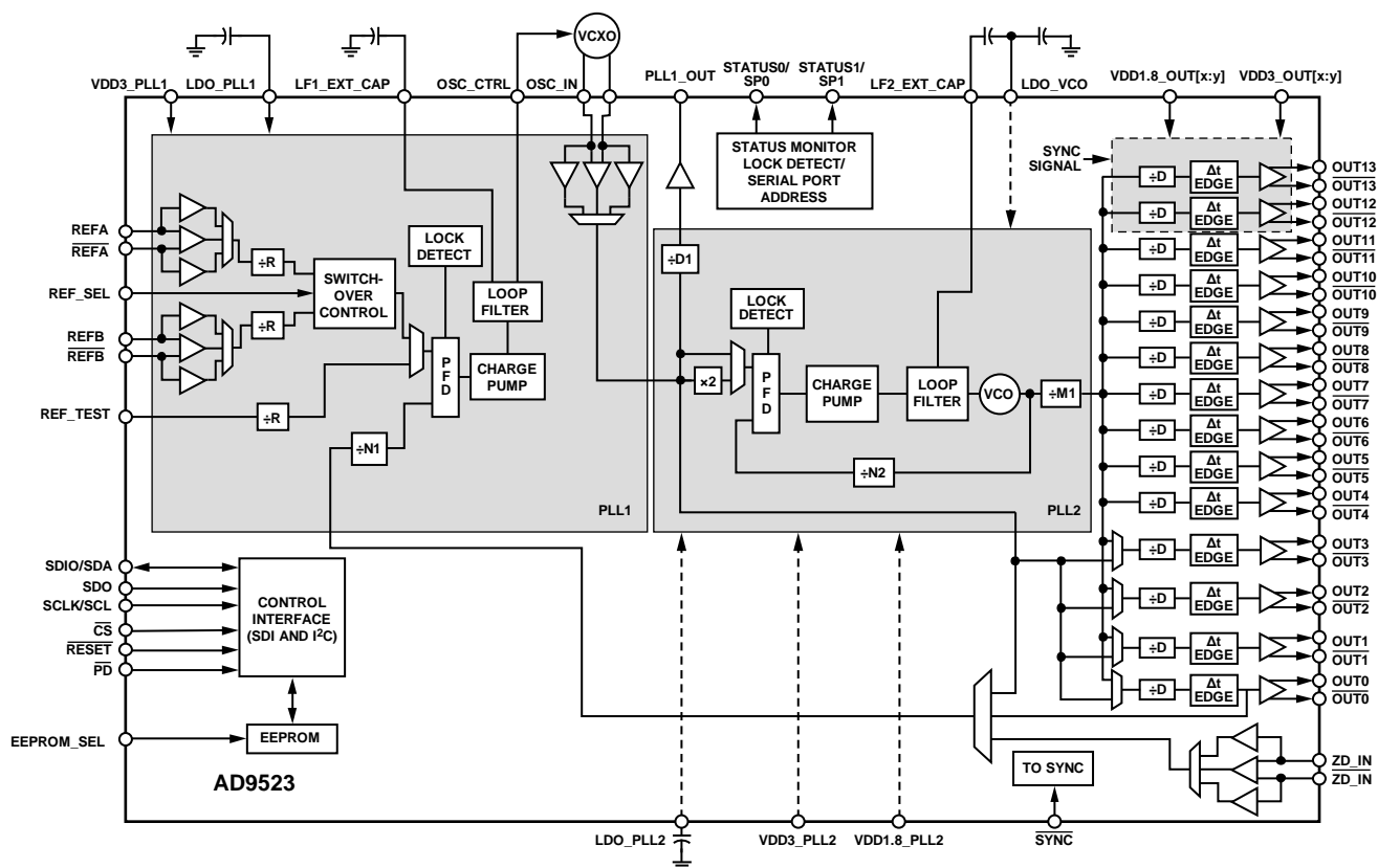
Figure 21. Top Level Diagram
