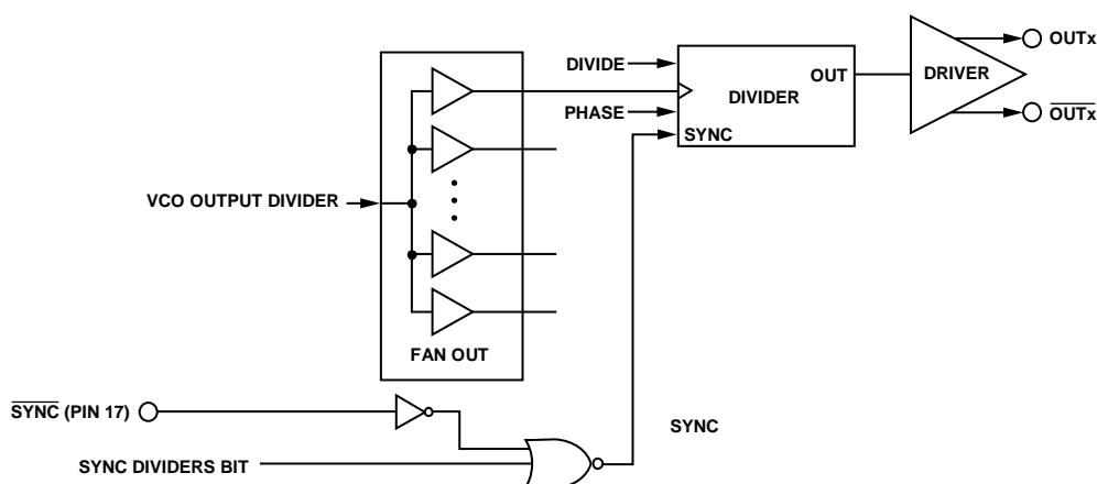
Figure 25. Clock Output Synchronization Block Diagram
