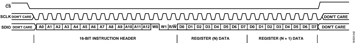
Figure 40. Serial Control Port Write—LSB First, 16-Bit Instruction, Two Bytes of Data
