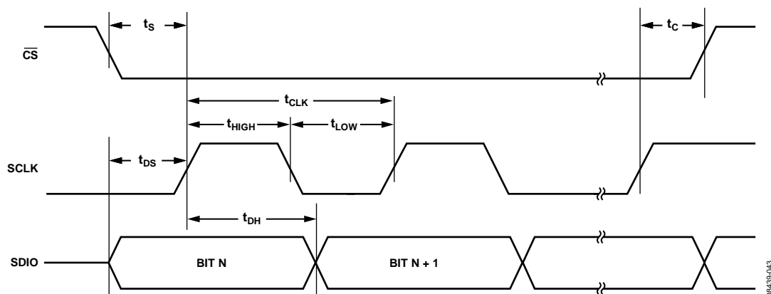
Figure 41. Serial Control Port Timing—Write
