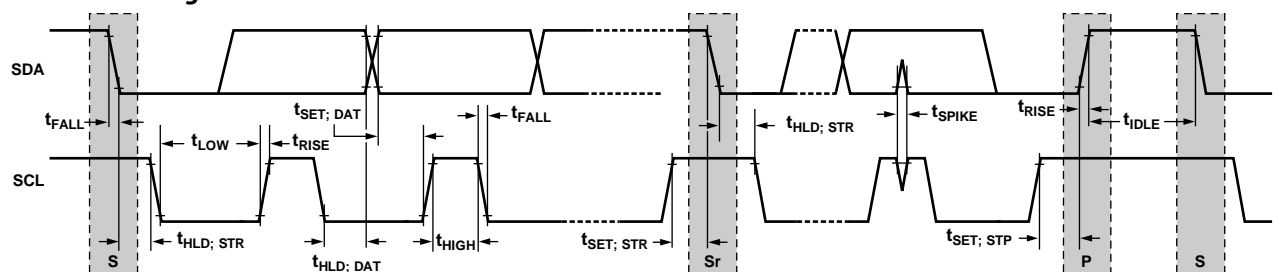
Figure 33. I 2 C Serial Port Timing
