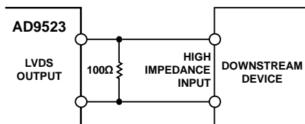
Figure 15. DC-Coupled LVDS Output Driver
