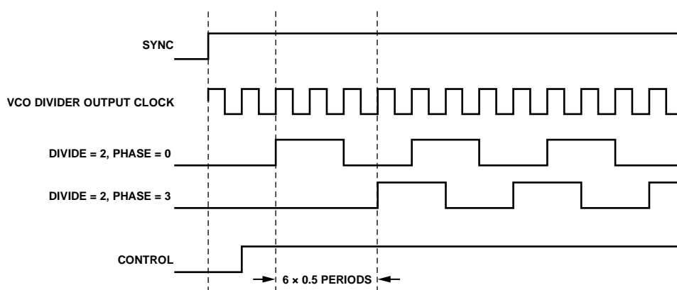
Figure 26. Clock Output Synchronization Timing Diagram
