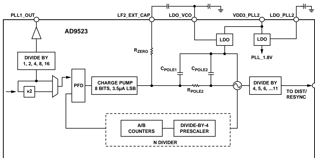
Figure 24. Output PLL (PLL2) Block Diagram
