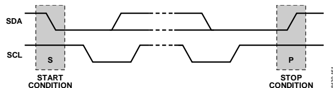
Figure 29. Start and Stop Conditions
