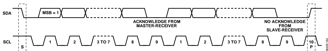
Figure 32. Data Transfer Process (Master Read Mode, 2-Byte Transfer Used for Illustration)
