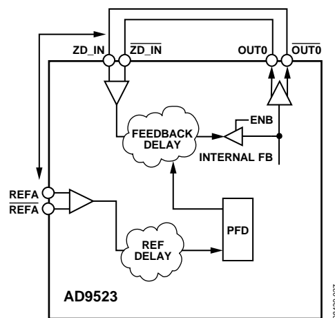
Figure 27. Zero Delay Function
