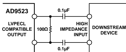
Figure 16. AC-Coupled LVPECL Output Driver
