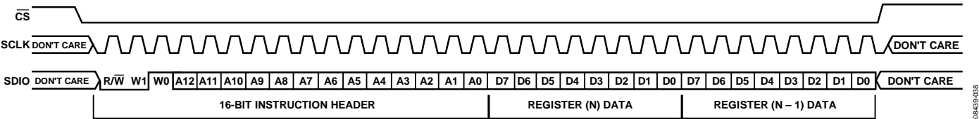
Figure 36. Serial Control Port Write—MSB First, 16-Bit Instruction, Two Bytes of Data
