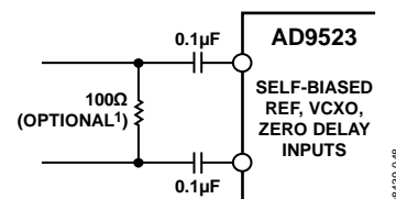
Figure 20. REF, VCXO, and Zero Delay Input Differential Mode
