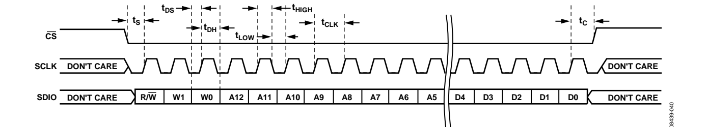
Figure 38. Serial Control Port Write—MSB First, 16-Bit Instruction, Timing Measurements
