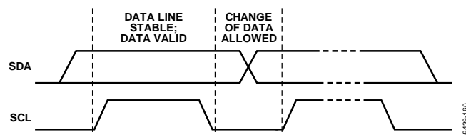
Figure 28. Valid Bit Transfer
