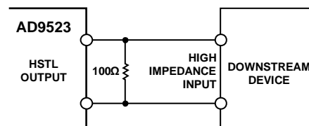
Figure 19. DC-Coupled HSTL Output Driver
