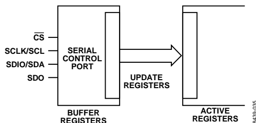
Figure 35. Relationship Between Serial Control Port Buffer Registers and Active Registers
