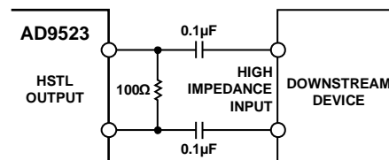
Figure 18. AC-Coupled HSTL Output Driver
