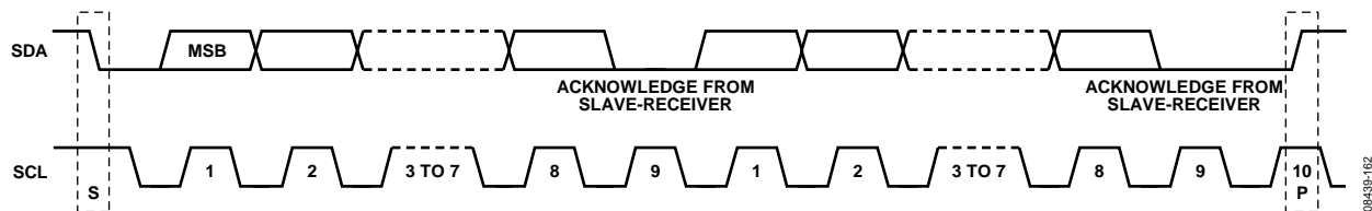
Figure 30. Acknowledge Bit
