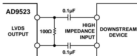
Figure 14. AC-Coupled LVDS Output Driver
