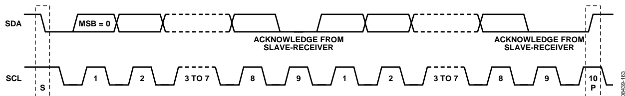
Figure 31. Data Transfer Process (Master Write Mode, 2-Byte Transfer Used for Illustration)
