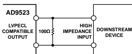
Figure 17. DC-Coupled LVPECL Output Driver
