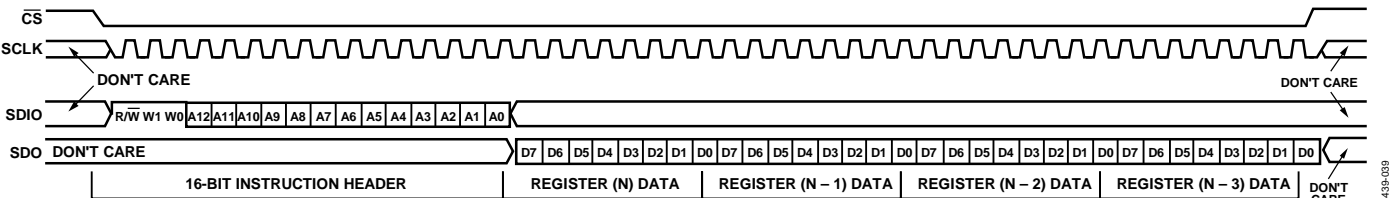
Figure 37. Serial Control Port Read—MSB First, 16-Bit Instruction, Four Bytes of Data
