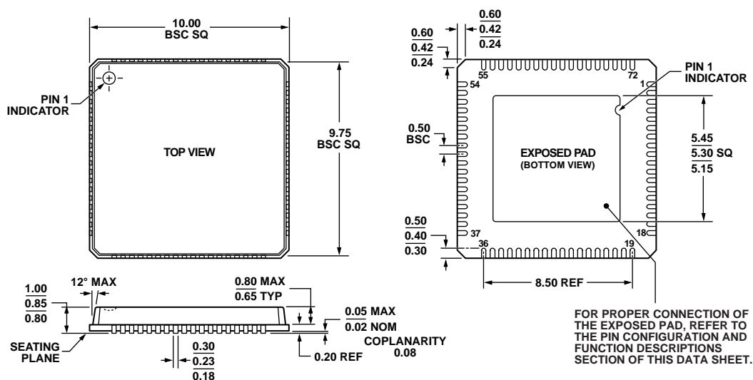
Figure 42. 72-Lead Lead Frame Chip Scale Package [LFCSP_VQ] 10 mm × 10 mm Body, Very Thin Quad (CP-72-6) Dimensions shown in millimeters
