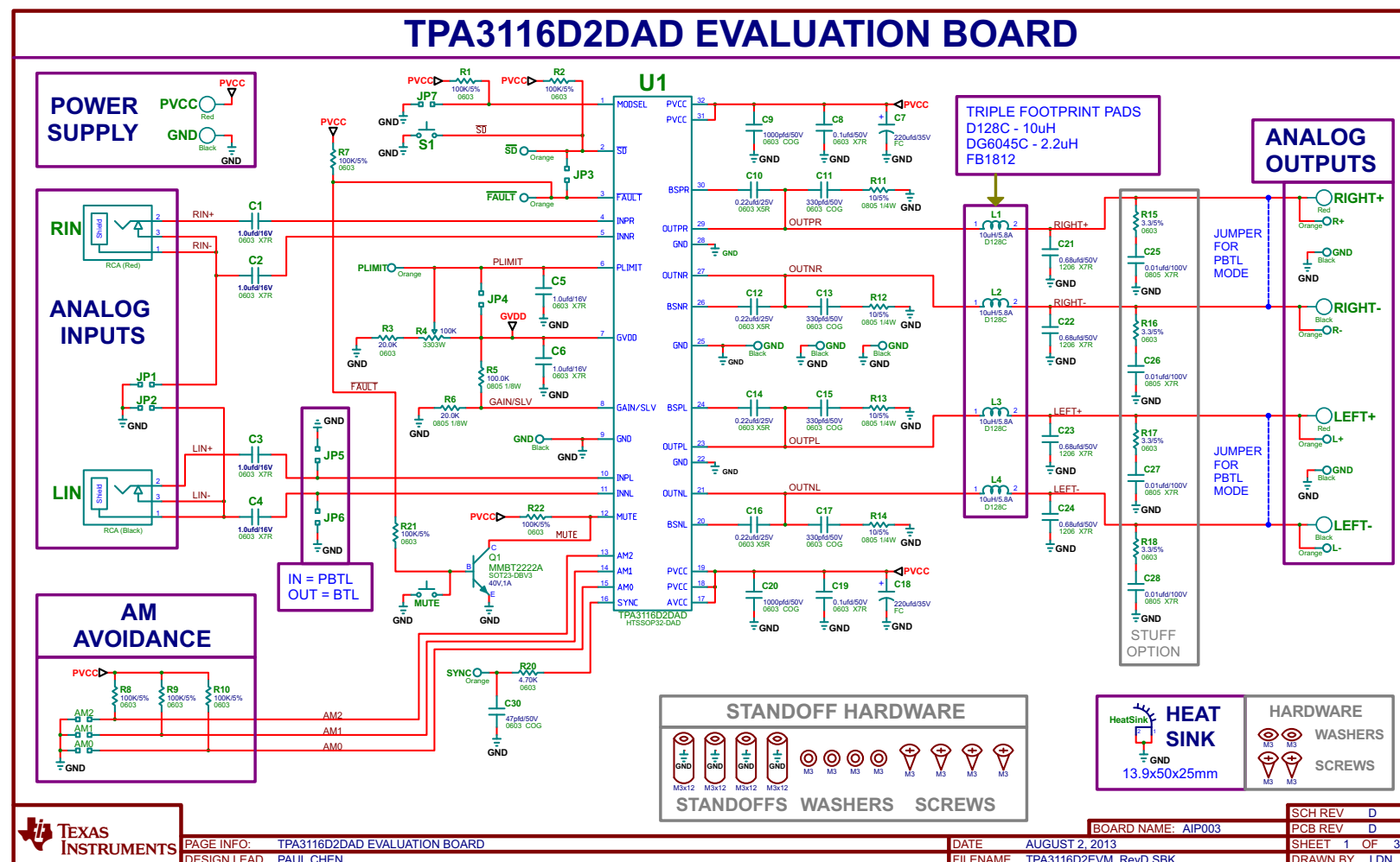
Figure 2. TPA3116D2EVM Schematic
