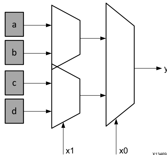
Figure 2-3: Functional Representation of a LUT as Collection of Memory Cells
