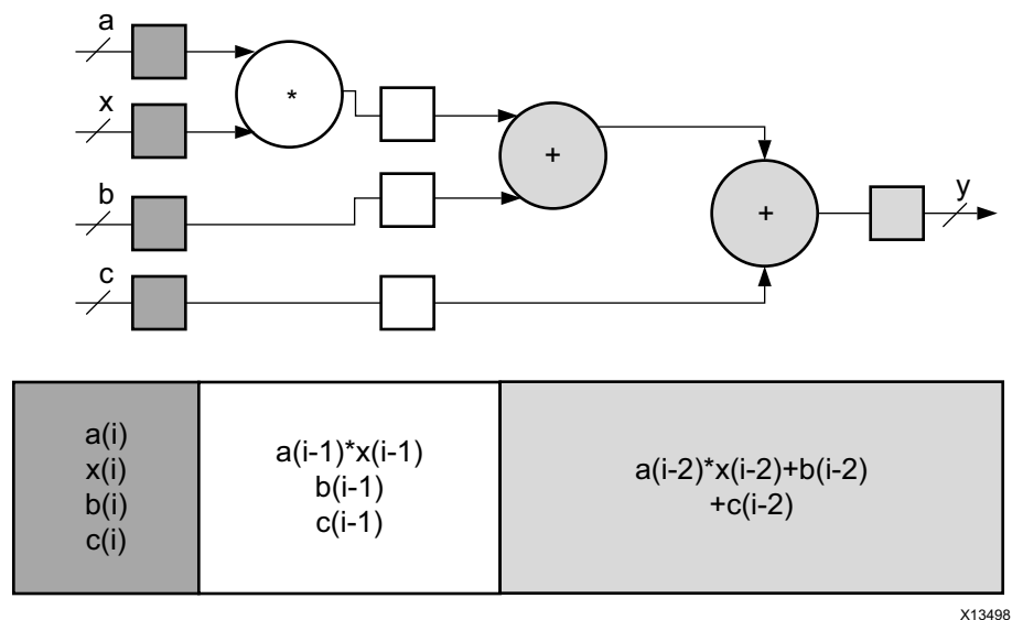
Figure 2-10: Pipelined Architecture
