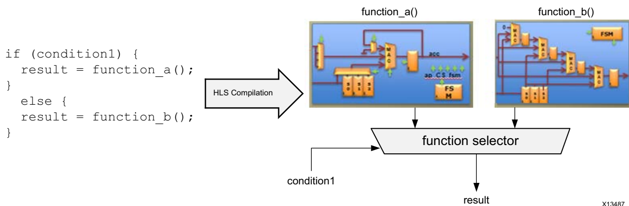
Figure 6-2: If-Else Example
